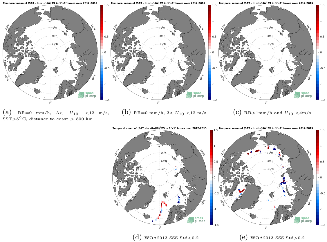
Figure 12: Temporal mean gridded over spatial boxes of size 1°x1° of \Delta SSS (SMOS SSS L3 v2 - Monthly - 0.25 Deg (CATDS-CECOS-IFREMER) - TSG (GOSUD-Sailing-ship)) for 5 different subdatasets corresponding to:RR=0 mm/h, 3 < U_{10} < 12 m/s, SST>5°C, distance to coast > 800 km (a), RR=0 mm/h, 3 < U_{10} < 12 m/s (b), RR>1mm/h and U_{10} < 4 m/s (c), WOA2013 SSS Std<0.2 (d), WOA2013 SSS Std>0.2 (e).
