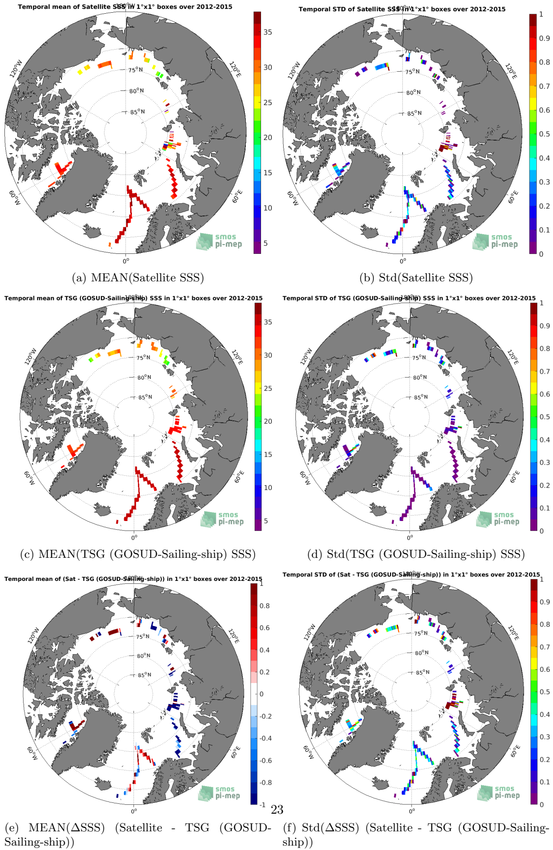
Figure 6: Temporal mean (left) and Std (right) of SSS from SMOS SSS L3 v2 - Monthly - 0.25 Deg (CATDS-CECOS-IFREMER) (top), TSG (GOSUD-Sailing-ship) (middle), and of \Delta SSS (Satellite - TSG (GOSUD-Sailing-ship)). Only match-up pairs are used to generate these maps.
