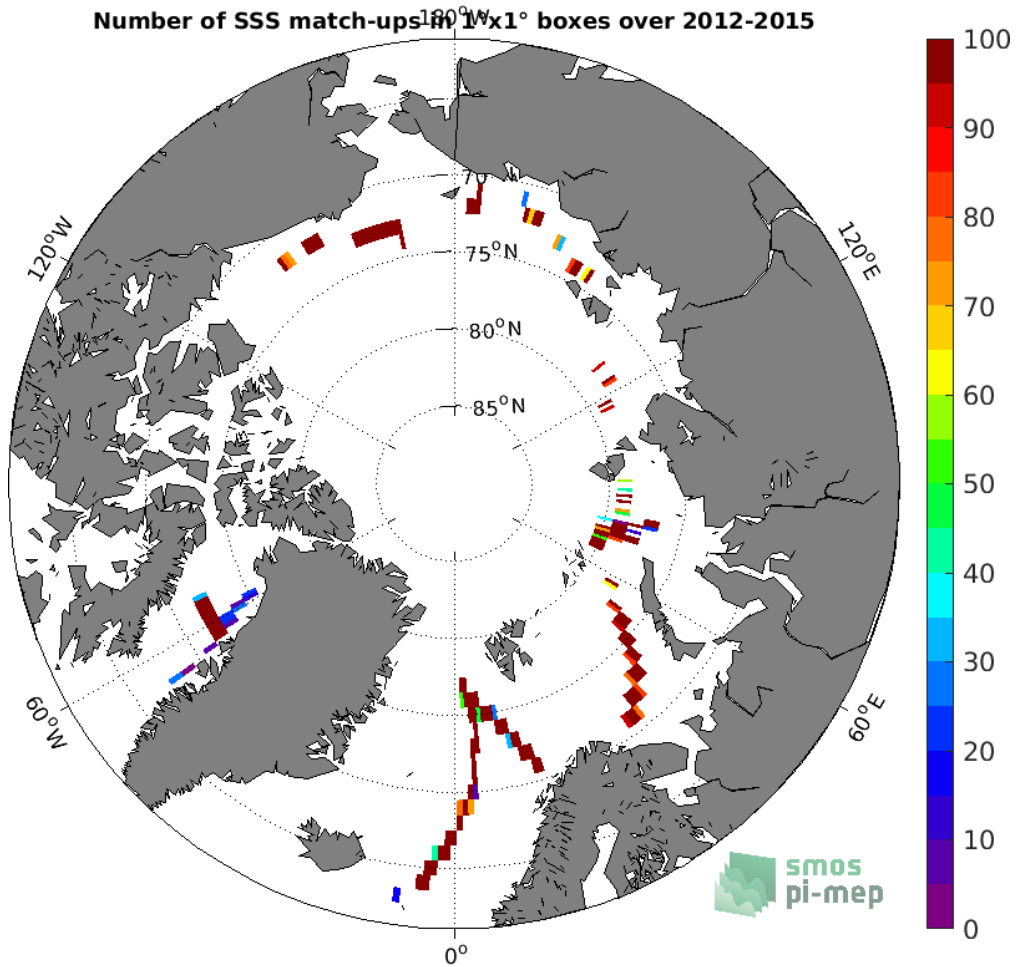
Figure 4: Number of SSS match-ups between TSG (GOSUD-Sailing-ship) SSS and the SMOS SSS L3 v2 - Monthly - 0.25 Deg (CATDS-CECOS-IFREMER) SSS product for the Arctic Ocean Pi-MEP region over 1°x1° boxes and for the full satellite product period.
