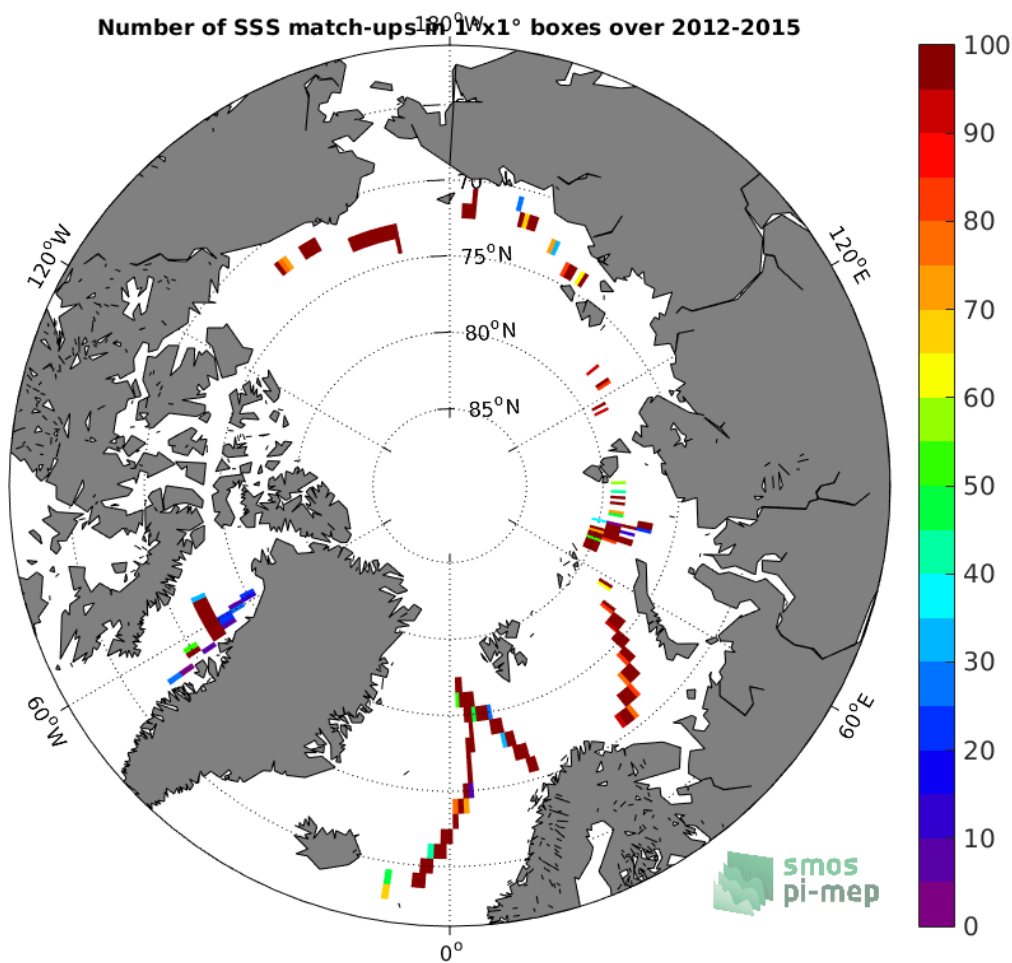
Figure 4: Number of SSS match-ups between TSG-GOSUD-Sailing-ship SSS and the SMOS L3 v2 - Monthly - 0.25 Deg (CATDS-CECOS-IFREMER) SSS product for the Arctic Ocean Pi-MEP region over 1°x1° boxes and for the full satellite product period.
