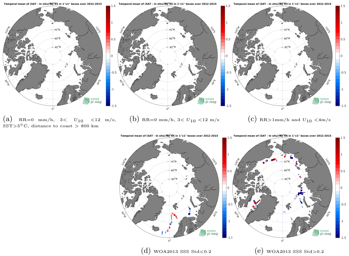
Figure 12: Temporal mean gridded over spatial boxes of size 1°x1° of \Delta SSS (SMOS L3 v2 - Monthly - 0.25 Deg (CATDS-CECOS-IFREMER) - TSG-GOSUD-Sailing-ship) for 5 different subdatasets corresponding to: RR=0 mm/h, 3 < U_{10} < 12 m/s, SST > 5°C, distance to coast > 800 km (a), RR=0 mm/h, 3 < U_{10} < 12 m/s (b), RR > 1mm/h and U_{10} < 4 m/s (c), WOA2013 SSS Std < 0.2 (d), WOA2013 SSS Std > 0.2 (e).
