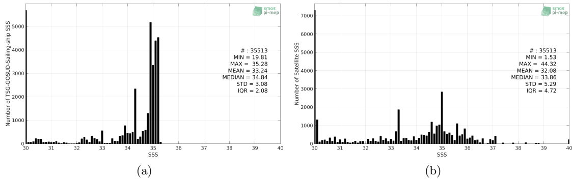
Figure 2: Histograms of SSS from TSG-GOSUD-Sailing-ship (a) and SMOS L3 v2 - Monthly - 0.25 Deg (CATDS-CECOS-IFREMER) (b) considering all match-up pairs per bins of 0.1 over the Arctic Ocean Pi-MEP region and for the full satellite product period.
