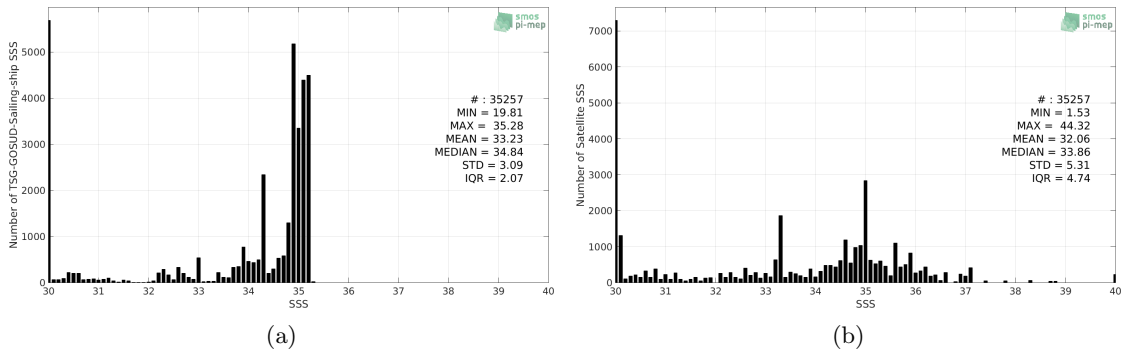
Figure 2: Histograms of SSS from TSG-GOSUD-Sailing-ship (a) and SMOS-L3-CATDS-IFREMER-CECOS-V2-MONTHLY-0.25DEG (b) considering all match-up pairs per bins of 0.1 over the Arctic Ocean Pi-MEP region and for the full satellite product period.
