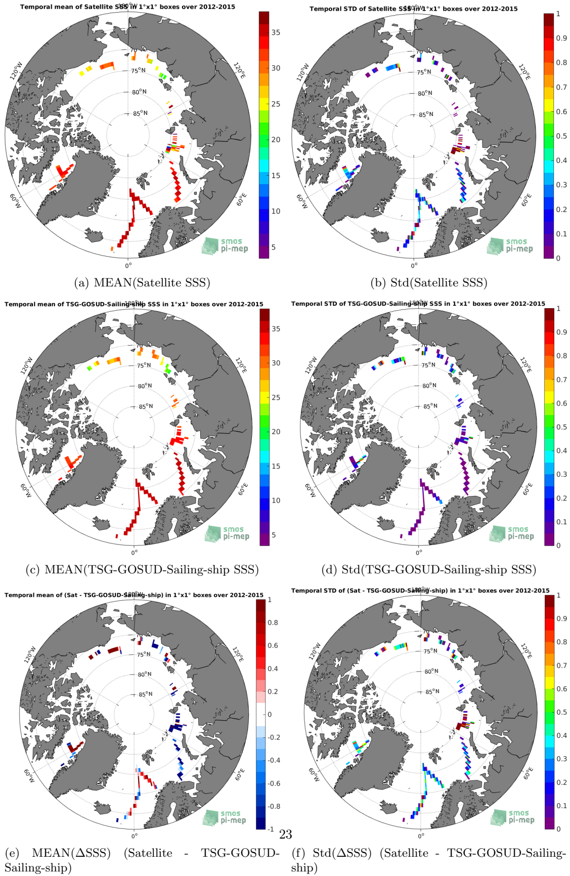
Figure 6: Temporal mean (left) and Std (right) of SSS from SMOS-L3-CATDS-IFREMER-CECOS-V2-MONTHLY-0.25DEG (top), TSG-GOSUD-Sailing-ship (middle), and of \Delta SSS (Satellite - TSG-GOSUD-Sailing-ship). Only match-up pairs are used to generate these maps.
