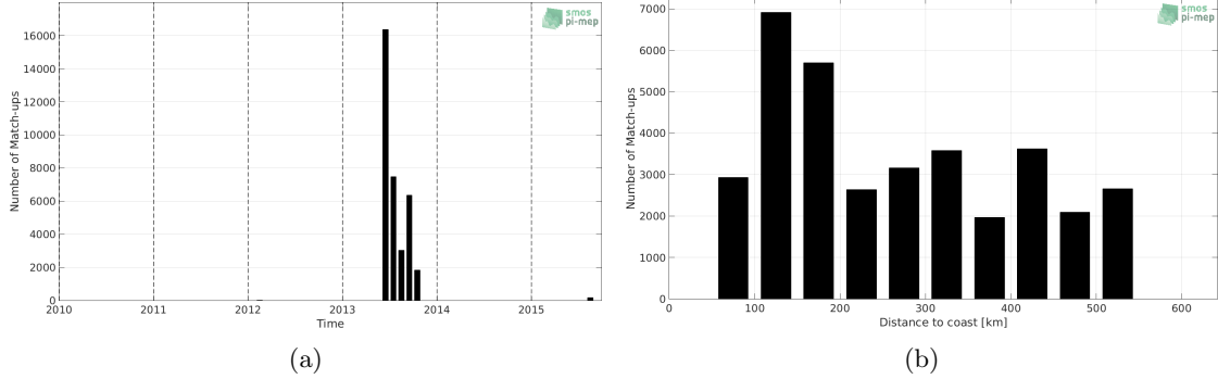
Figure 1: Number of match-ups between TSG-GOSUD-Sailing-ship and SMOS-L3-CATDS-IFREMER-CECOS-V2-MONTHLY-0.25DEG SSS as a function of time (a) and as function of the distance to coast (b) over the Arctic Ocean Pi-MEP region and for the full satellite product period.
