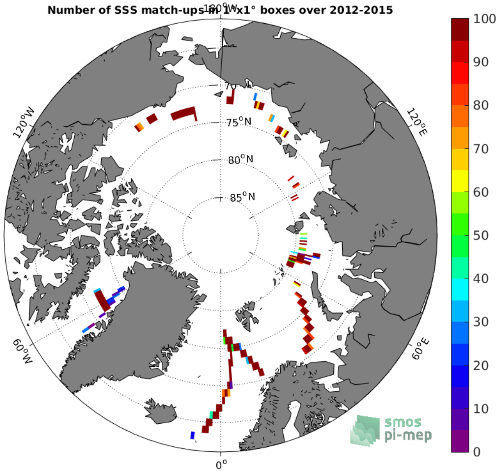
Figure 4: Number of SSS match-ups between TSG-GOSUD-Sailing-ship SSS and the SMOS-L3-CATDS-IFREMER-CECOS-V2-MONTHLY-0.25DEG SSS product for the Arctic Ocean Pi-MEP region over 1^\circ \times 1^\circ boxes and for the full satellite product period.
