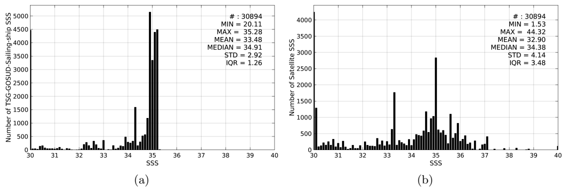
Figure 2: Histograms of SSS from TSG-GOSUD-Sailing-ship (a) and SMOS-L3-CATDS-IFREMER-CECOS-V2-MONTHLY-0.25DEG (b) considering all match-up pairs per bins of 0.1 over the Arctic Ocean Pi-MEP region and for the full satellite product period.
