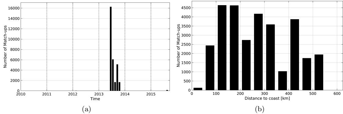
Figure 1: Number of match-ups between TSG-GOSUD-Sailing-ship and SMOS-L3-CATDS-IFREMER-CECOS-V2-MONTHLY-0.25DEG SSS as a function of time (a) and as function of the distance to coast (b) over the Arctic Ocean Pi-MEP region and for the full satellite product period.
