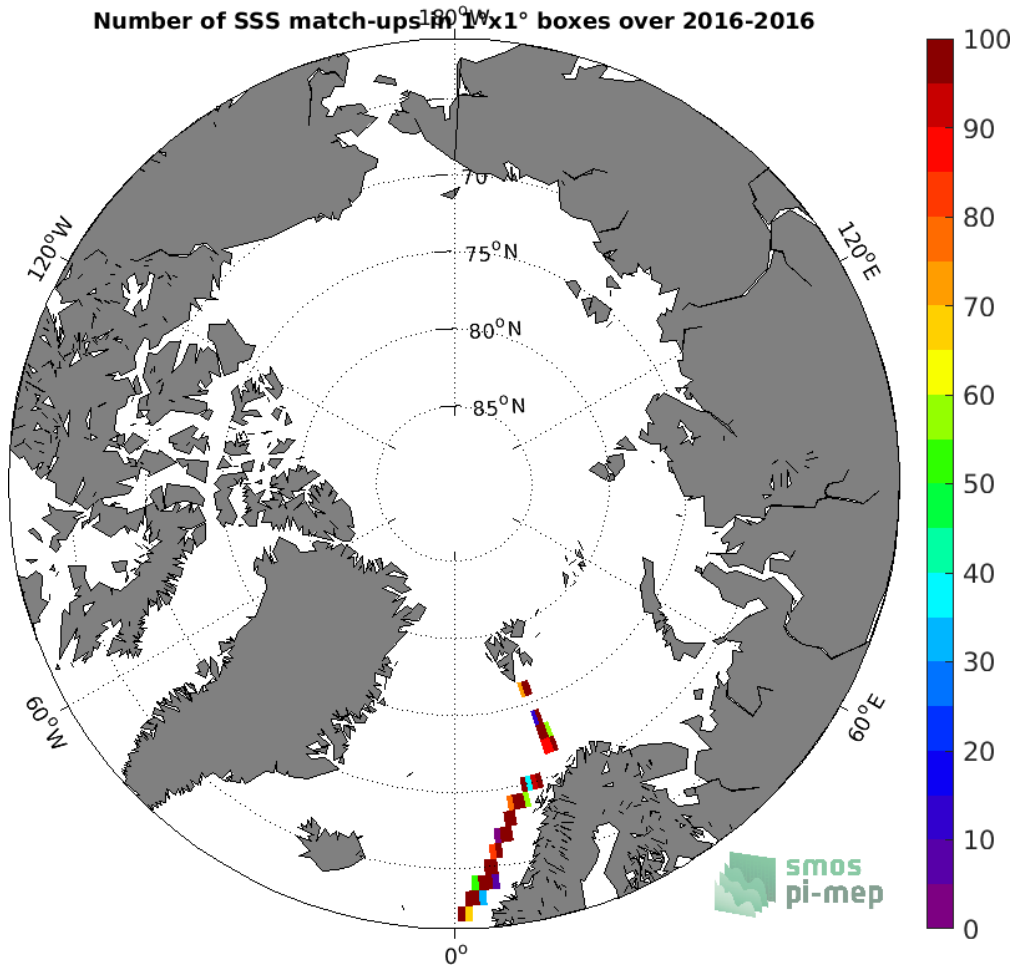
Figure 4: Number of SSS match-ups between TSG (GOSUD-Research-vessel) SSS and the SMOS SSS L3 v2 - Monthly - 0.25 Deg (CATDS-CECOS-IFREMER) SSS product for the Arctic Ocean Pi-MEP region over 1°x1° boxes and for the full satellite product period.
