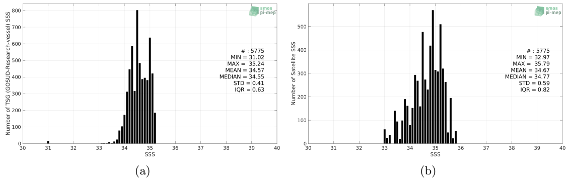
Figure 2: Histograms of SSS from TSG (GOSUD-Research-vessel) (a) and SMOS SSS L3 v2 - Monthly - 0.25 Deg (CATDS-CECOS-IFREMER) (b) considering all match-up pairs per bins of 0.1 over the Arctic Ocean Pi-MEP region and for the full satellite product period.
