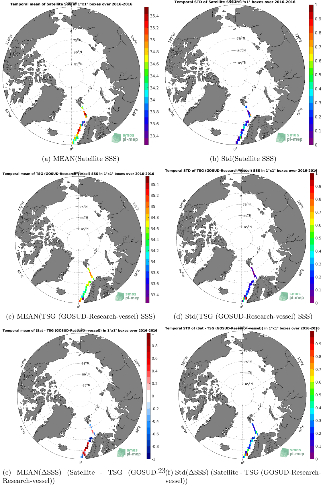
Figure 6: Temporal mean (left) and Std (right) of SSS from SMOS SSS L3 v2 - Monthly - 0.25 Deg (CATDS-CECOS-IFREMER) (top), TSG (GOSUD-Research-vessel) (middle), and of \Delta SSS (Satellite - TSG (GOSUD-Research-vessel)). Only match-up pairs are used to generate these maps.
