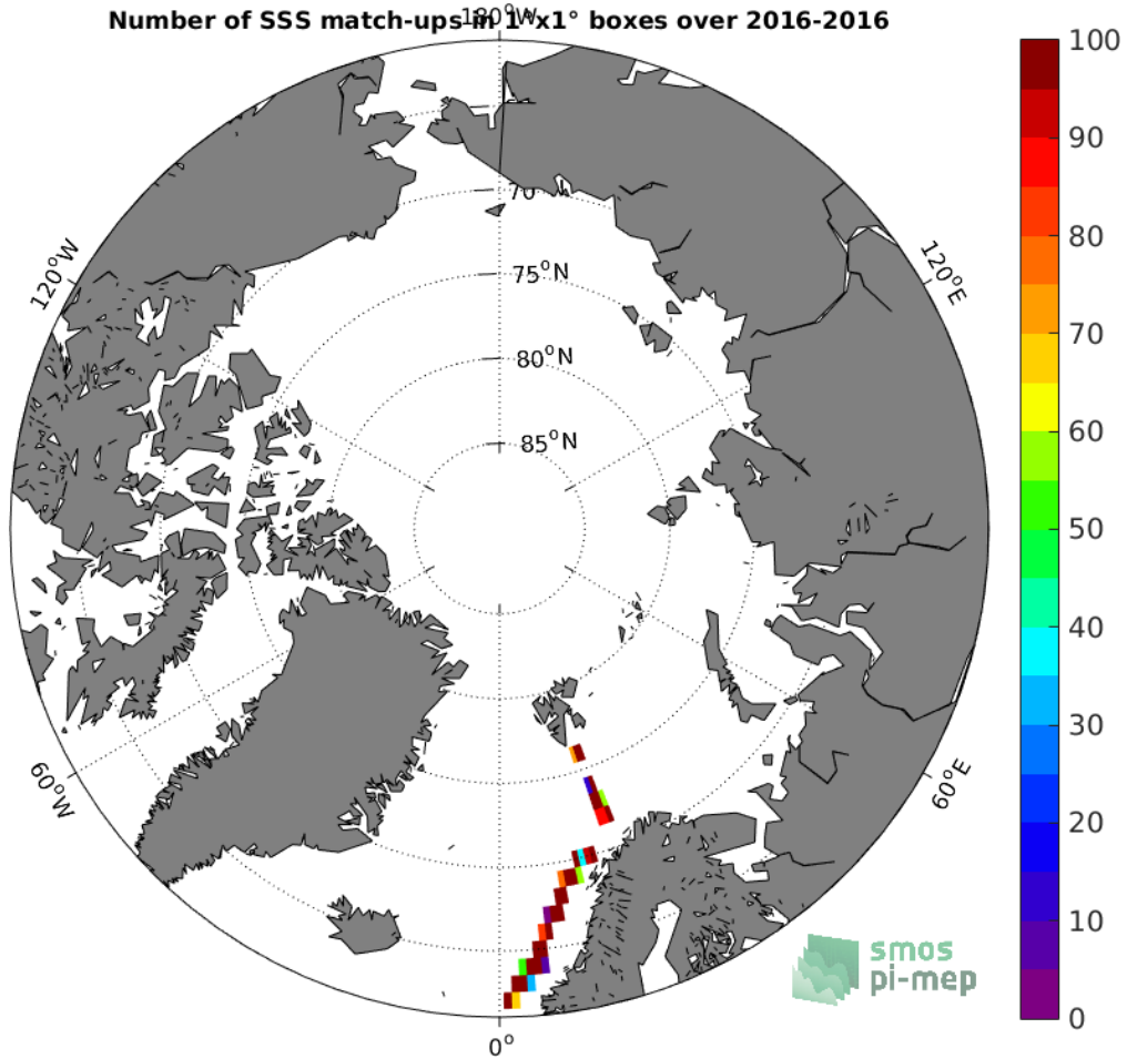
Figure 4: Number of SSS match-ups between TSG (GOSUD-Research-vessel) SSS and the SMOS SSS L3 v2 - Monthly - 0.25 Deg (CATDS-CECOS-IFREMER) SSS product for the Arctic Ocean Pi-MEP region over 1^{\circ} \times 1^{\circ} boxes and for the full satellite product period.
