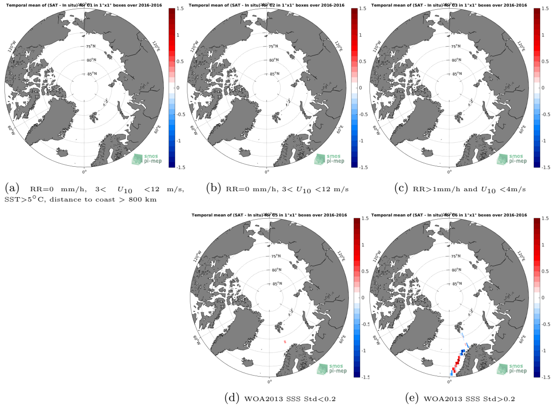
Figure 12: Temporal mean gridded over spatial boxes of size 1°x1° of \Delta SSS (SMOS SSS L3 v2 - Monthly - 0.25 Deg (CATDS-CECOS-IFREMER) - TSG (GOSUD-Research-vessel)) for 5 different subdatasets corresponding to: RR=0 mm/h, 3 < U_{10} < 12 m/s, SST > 5°C, distance to coast > 800 km (a), RR=0 mm/h, 3 < U_{10} < 12 m/s (b), RR > 1mm/h and U_{10} < 4 m/s (c), WOA2013 SSS Std < 0.2 (d), WOA2013 SSS Std > 0.2 (e).
