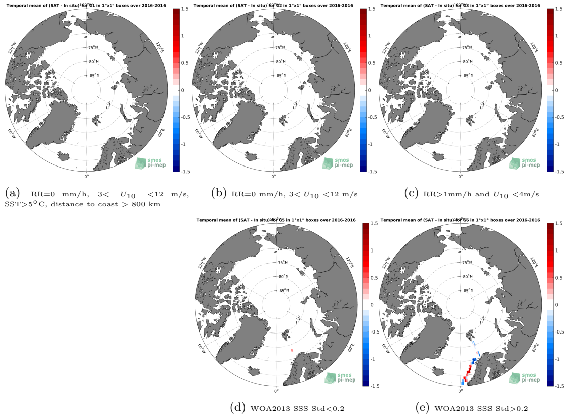
Figure 12: Temporal mean gridded over spatial boxes of size 1°x1° of \Delta SSS (SMOS L3 v2 - Monthly - 0.25 Deg (CATDS-CECOS-IFREMER) - TSG-GOSUD-Research-vessel) for 5 different subdatasets corresponding to: RR=0 mm/h, 3 < U_{10} < 12 m/s, SST > 5°C, distance to coast > 800 km (a), RR=0 mm/h, 3 < U_{10} < 12 m/s (b), RR > 1mm/h and U_{10} < 4 m/s (c), WOA2013 SSS Std < 0.2 (d), WOA2013 SSS Std > 0.2 (e).
