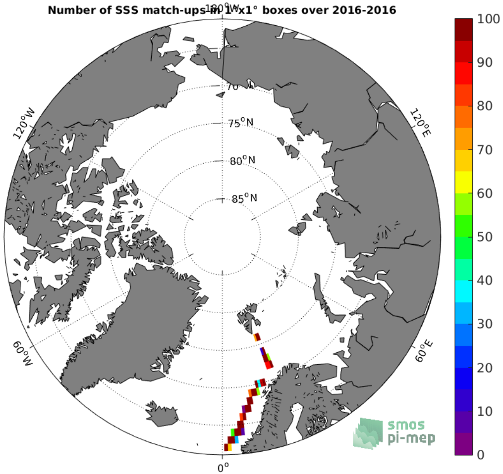
Figure 4: Number of SSS match-ups between TSG-GOSUD-Research-vessel SSS and the SMOS L3 v2 - Monthly - 0.25 Deg (CATDS-CECOS-IFREMER) SSS product for the Arctic Ocean Pi-MEP region over 1^{\circ} \times 1^{\circ} boxes and for the full satellite product period.
