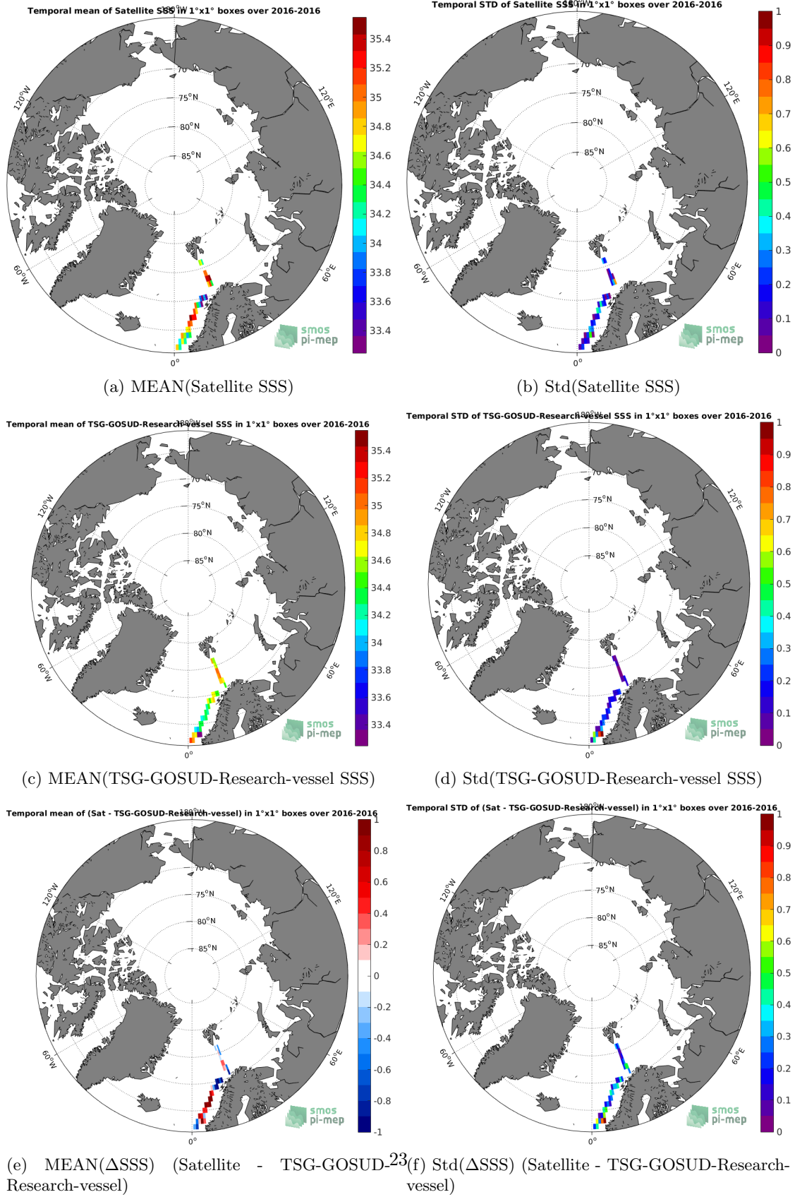
Figure 6: Temporal mean (left) and Std (right) of SSS from SMOS L3 v2 - Monthly - 0.25 Deg (CATDS-CECOS-IFREMER) (top), TSG-GOSUD-Research-vessel (middle), and of \Delta SSS (Satellite - TSG-GOSUD-Research-vessel). Only match-up pairs are used to generate these maps.
