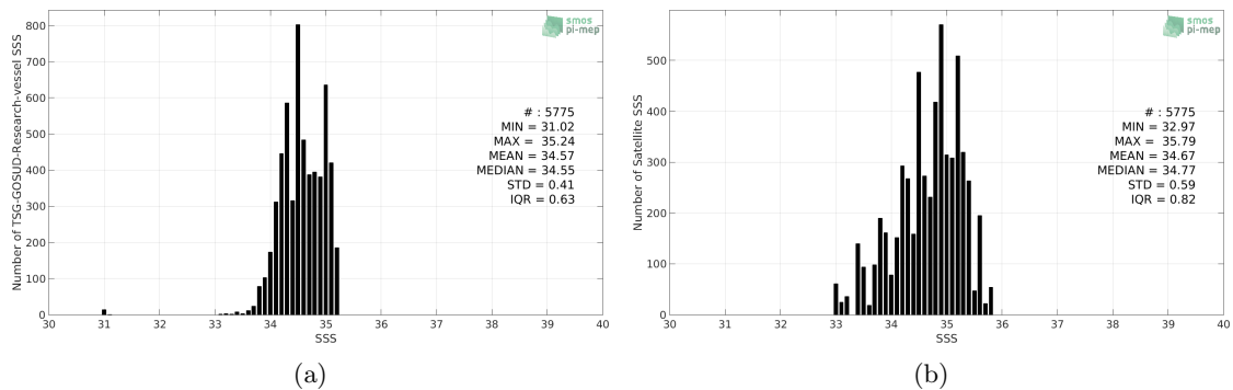
Figure 2: Histograms of SSS from TSG-GOSUD-Research-vessel (a) and SMOS-L3-CATDS-IFREMER-CECOS-V2-MONTHLY-0.25DEG (b) considering all match-up pairs per bins of 0.1 over the Arctic Ocean Pi-MEP region and for the full satellite product period.
