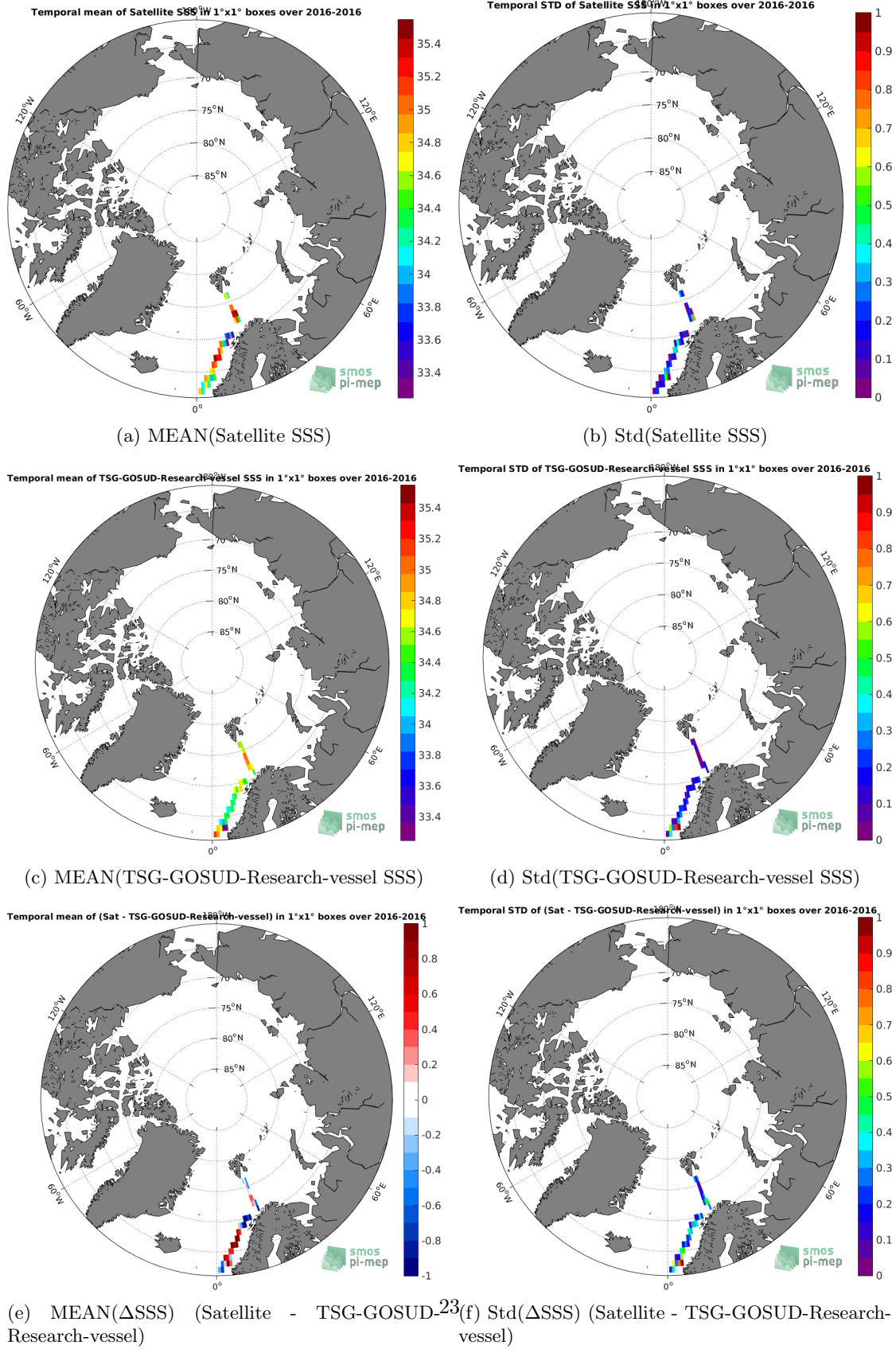
Figure 6: Temporal mean (left) and Std (right) of SSS from SMOS-L3-CATDS-IFREMER-CECOS-V2-MONTHLY-0.25DEG (top), TSG-GOSUD-Research-vessel (middle), and of \Delta SSS (Satellite - TSG-GOSUD-Research-vessel). Only match-up pairs are used to generate these maps.
