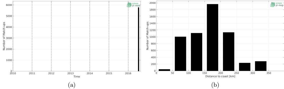
Figure 1: Number of match-ups between TSG-GOSUD-Research-vessel and SMOS-L3-CATDS-IFREMER-CECOS-V2-MONTHLY-0.25DEG SSS as a function of time (a) and as function of the distance to coast (b) over the Arctic Ocean Pi-MEP region and for the full satellite product period.
