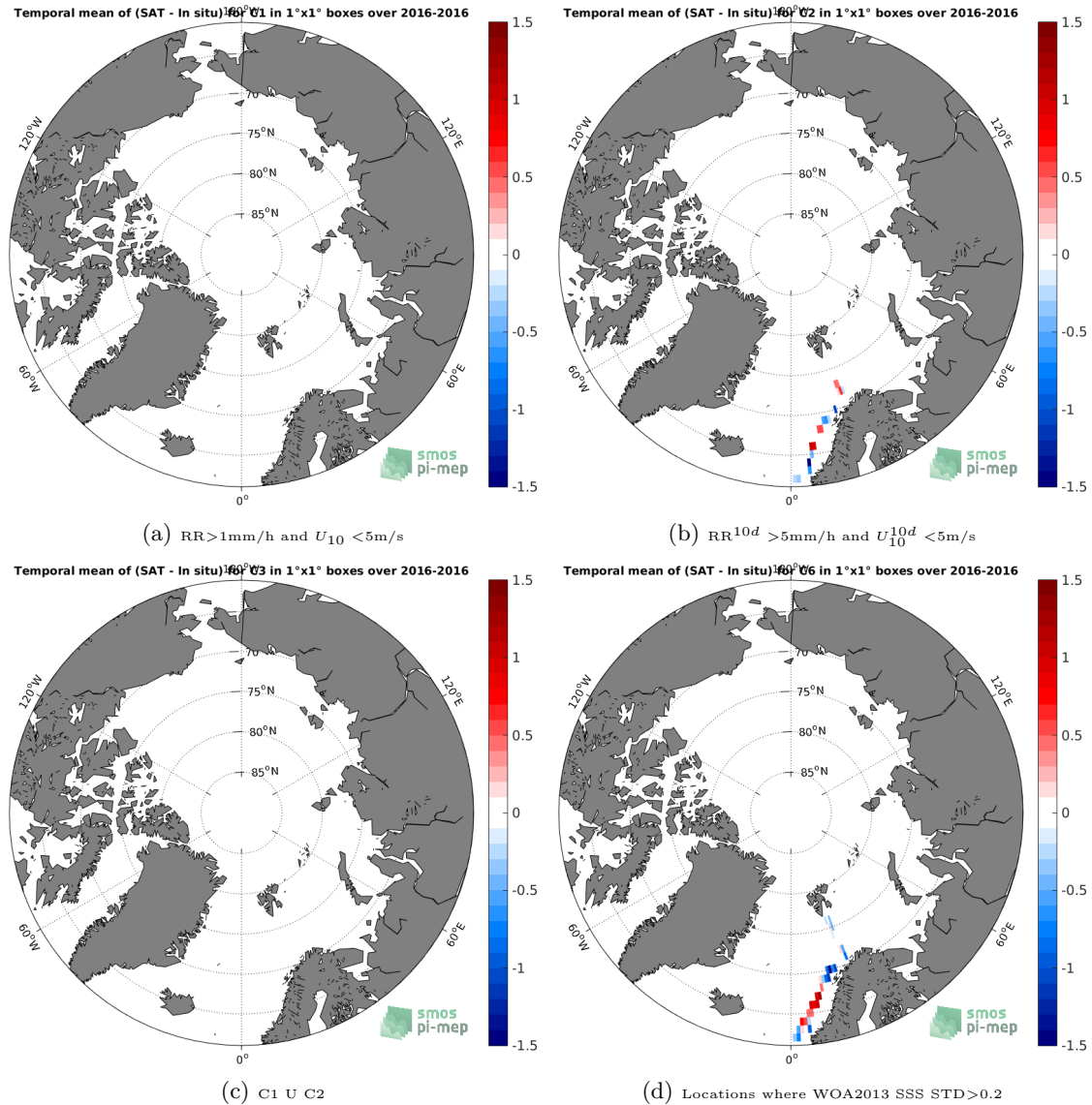
Figure 12: Temporal mean gridded over spatial boxes of size 1^\circ \times 1^\circ of \Delta SSS (SMOS-L3-CATDS-IFREMER-CECOS-V2-MONTHLY-0.25DEG - TSG-GOSUD-Research-vessel) for 4 different subdatasets corresponding to: RR > 1\text{mm/h} and U_{10} < 5\text{m/s} (a), RR^{10d} > 5\text{mm/h} and U_{10}^{10d} < 5\text{m/s} (b), C1 U C2 (c), Locations where WOA2013 SSS STD > 0.2 (d).
