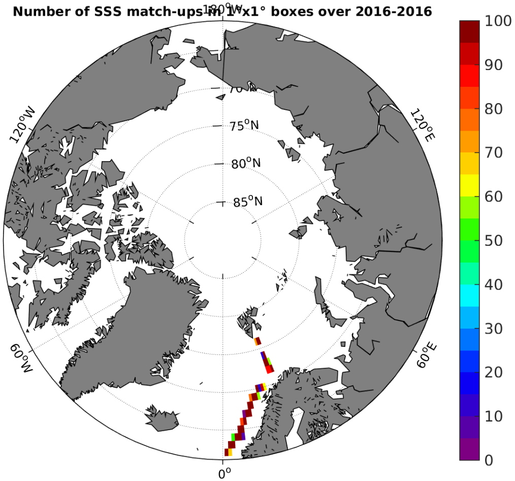
Figure 4: Number of SSS match-ups between TSG-GOSUD-Research-vessel SSS and the SMOS-L3-CATDS-IFREMER-CECOS-V2-MONTHLY-0.25DEG SSS product for the Arctic Ocean Pi-MEP region over 1°x1° boxes and for the full satellite product period.
