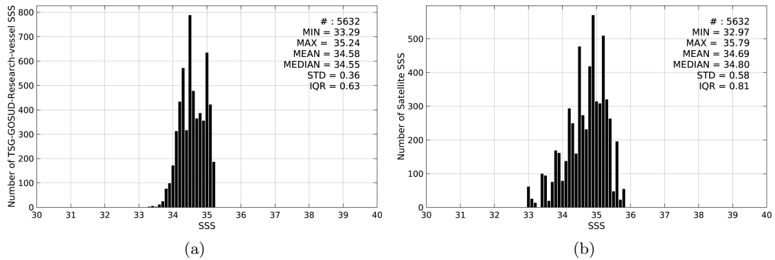
Figure 2: Histograms of SSS from TSG-GOSUD-Research-vessel (a) and SMOS-L3-CATDS-IFREMER-CECOS-V2-MONTHLY-0.25DEG (b) considering all match-up pairs per bins of 0.1 over the Arctic Ocean Pi-MEP region and for the full satellite product period.
