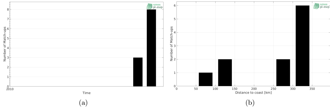
Figure 1: Number of match-ups between Sea mammals and SMOS SSS L3 v2 - Monthly - 0.25 Deg (CATDS-CECOS-IFREMER) SSS as a function of time (a) and as function of the distance to coast (b) over the Arctic Ocean Pi-MEP region and for the full satellite product period.
