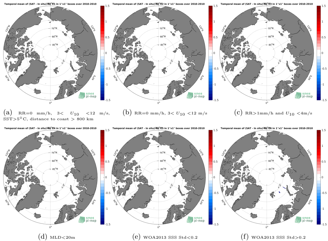
Figure 12: Temporal mean gridded over spatial boxes of size 1^\circ \times 1^\circ of \Delta SSS (SMOS-L3-CATDS-IFREMER-CECOS-V2-MONTHLY-0.25DEG - Sea mammals) for 6 different subdatasets corresponding to:RR=0 mm/h, 3 < U_{10} < 12 m/s, SST >5^\circ C, distance to coast > 800 km (a), RR=0 mm/h, 3 < U_{10} < 12 m/s (b), RR >1 mm/h and U_{10} < 4 m/s (c),MLD <20 m (d),WOA2013 SSS Std <0.2 (e),WOA2013 SSS Std >0.2 (f).
