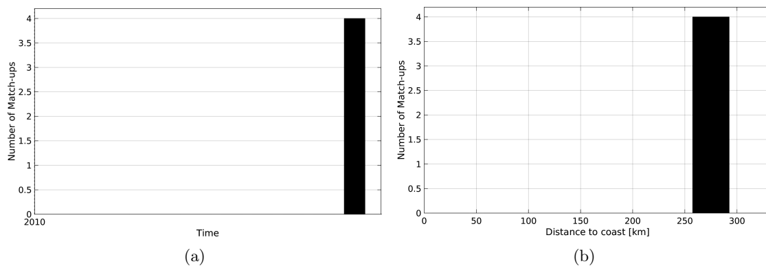
Figure 1: Number of match-ups between Sea mammals and SMOS-L3-CATDS-IFREMER-CECOS-V2-MONTHLY-0.25DEG SSS as a function of time (a) and as function of the distance to coast (b) over the Arctic Ocean Pi-MEP region and for the full satellite product period.
