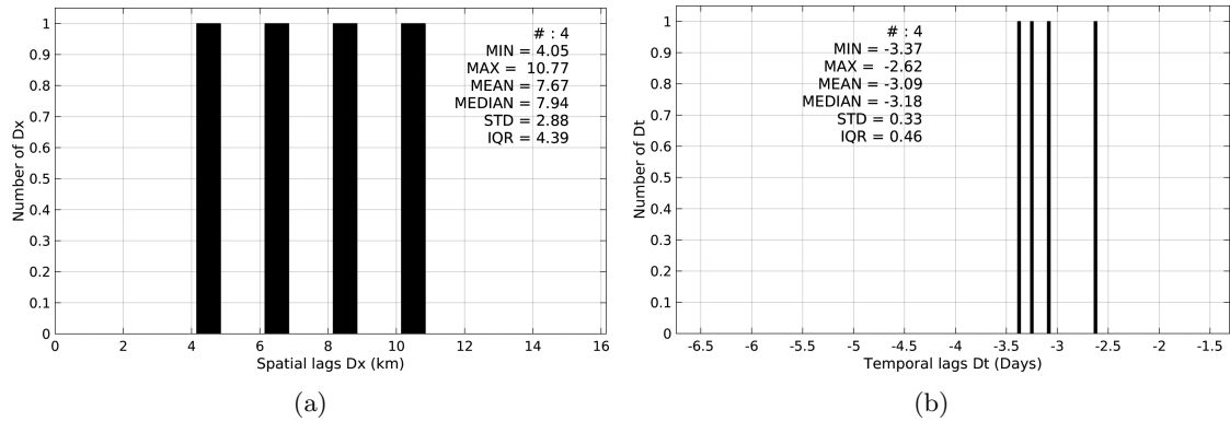
Figure 5: Histograms of the spatial (a) and temporal (b) lags between the time of the Sea mammals measurements and the date of the corresponding SMOS-L3-CATDS-IFREMER-CECOS-V2-MONTHLY-0.25DEG SSS product.
