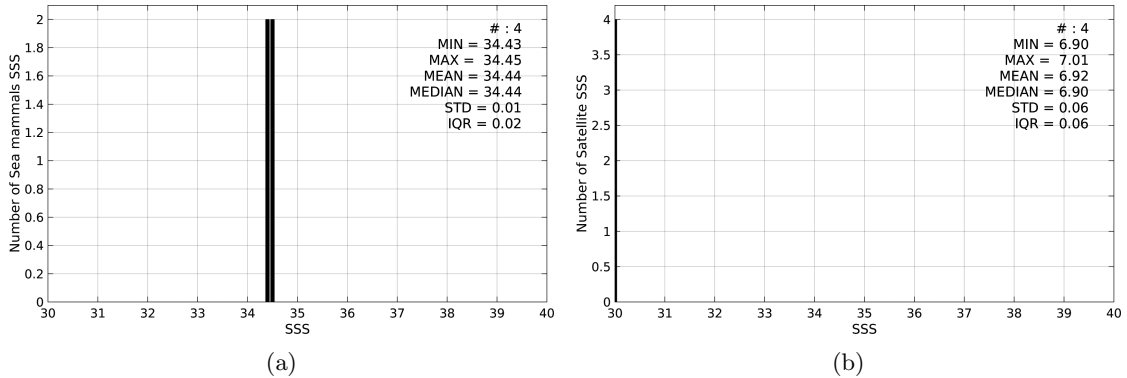
Figure 2: Histograms of SSS from Sea mammals (a) and SMOS-L3-CATDS-IFREMER-CECOS-V2-MONTHLY-0.25DEG (b) considering all match-up pairs per bins of 0.1 over the Arctic Ocean Pi-MEP region and for the full satellite product period.
