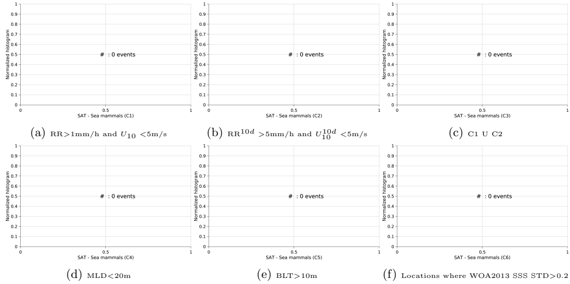
Figure 13: Normalized histogram of \Delta\text{SSS} (SMOS-L3-CATDS-IFREMER-CECOS-V2-MONTHLY-0.25DEG - Sea mammals) for 6 different subdatasets corresponding to: RR > 1\text{mm/h} and U_{10} < 5\text{m/s} (a), RR^{10d} > 5\text{mm/h} and U_{10}^{10d} < 5\text{m/s} (b), C1 \cup C2 (c), MLD < 20\text{m} (d), BLT > 10\text{m} (e), Locations where WOA2013 SSS STD > 0.2 (f).
