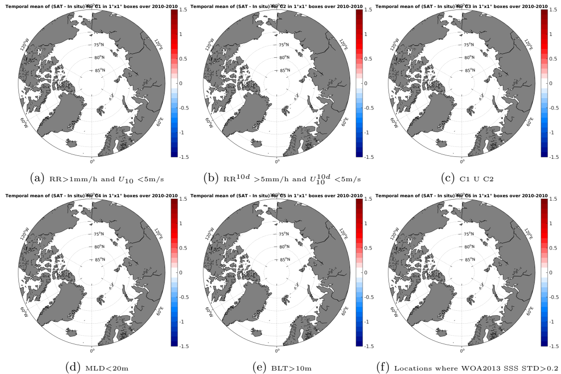
Figure 12: Temporal mean gridded over spatial boxes of size 1°x1° of \Delta SSS (SMOS-L3-CATDS-IFREMER-CECOS-V2-MONTHLY-0.25DEG - Sea mammals) for 6 different subdatasets corresponding to:RR>1mm/h and U_{10} <5m/s (a), RR^{10d} >5mm/h and U_{10}^{10d} <5m/s (b), C1 U C2 (c),MLD<20m (d),BLT>10m (e),Locations where WOA2013 SSS STD>0.2 (f).
