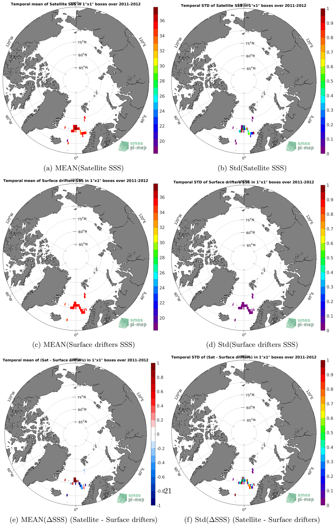
Figure 5: Temporal mean (left) and Std (right) of SSS from SMOS SSS L3 v2 - Monthly - 0.25 Deg (CATDS-CECOS-IFREMER) (top), Surface drifters (middle), and of \Delta SSS (Satellite - Surface drifters). Only match-up pairs are used to generate these maps.
