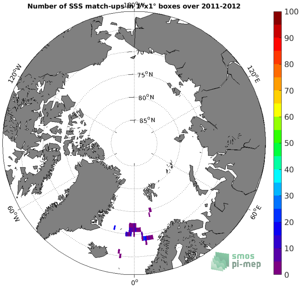
Figure 3: Number of SSS match-ups between Surface drifters SSS and the SMOS SSS L3 v2 - Monthly - 0.25 Deg (CATDS-CECOS-IFREMER) SSS product for the Arctic Ocean Pi-MEP region over 1°x1° boxes and for the full satellite product period.
