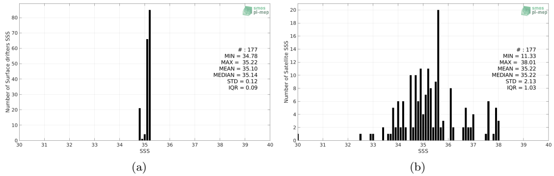
Figure 2: Histograms of SSS from Surface drifters (a) and SMOS SSS L3 v2 - Monthly - 0.25 Deg (CATDS-CECOS-IFREMER) (b) considering all match-up pairs per bins of 0.1 over the Arctic Ocean Pi-MEP region and for the full satellite product period.
