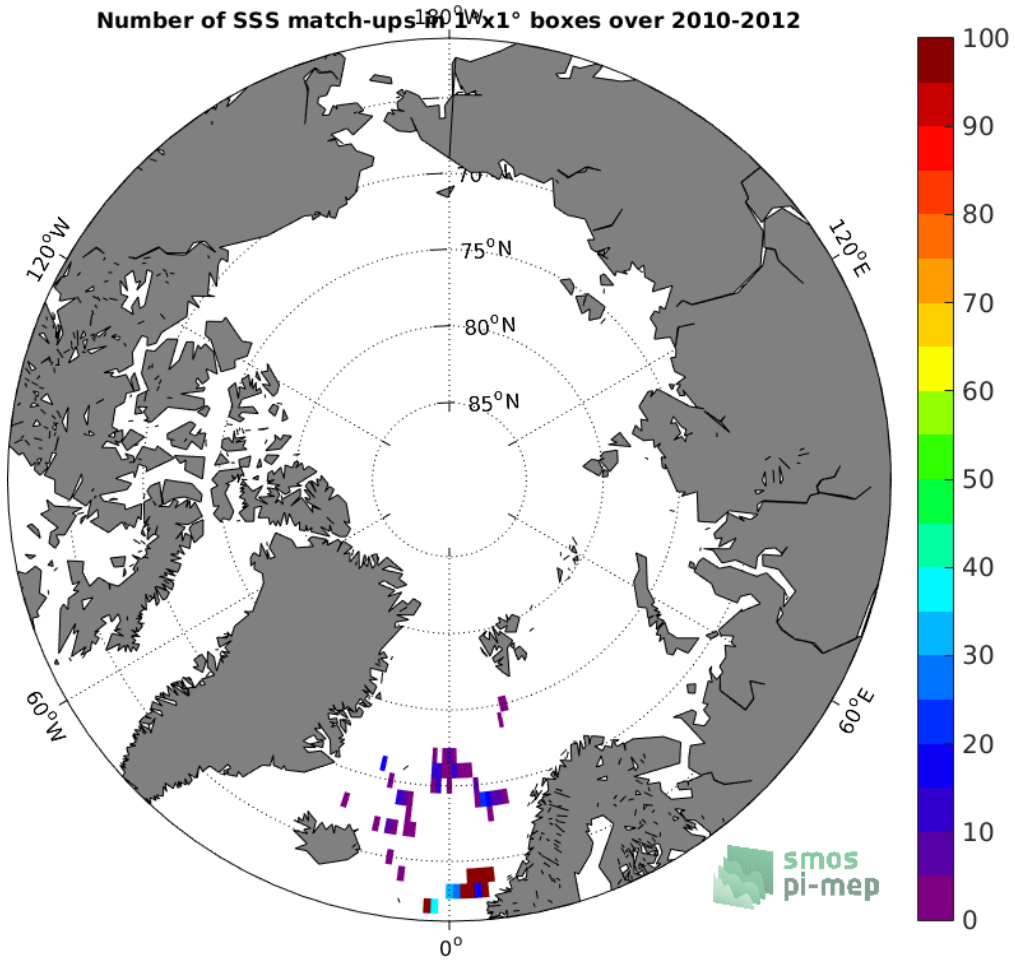
Figure 3: Number of SSS match-ups between Surface drifters SSS and the SMOS L3 v2 - Monthly - 0.25 Deg (CATDS-CECOS-IFREMER) SSS product for the Arctic Ocean Pi-MEP region over 1°x1° boxes and for the full satellite product period.
