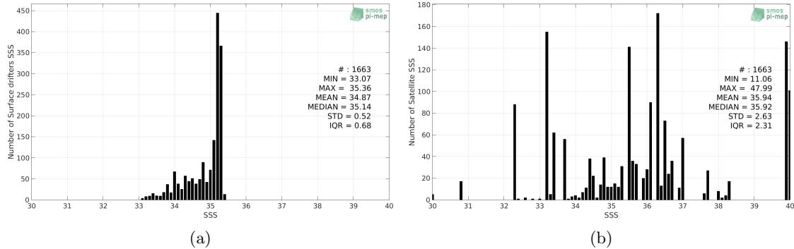
Figure 2: Histograms of SSS from Surface drifters (a) and SMOS L3 v2 - Monthly - 0.25 Deg (CATDS-CECOS-IFREMER) (b) considering all match-up pairs per bins of 0.1 over the Arctic Ocean Pi-MEP region and for the full satellite product period.
