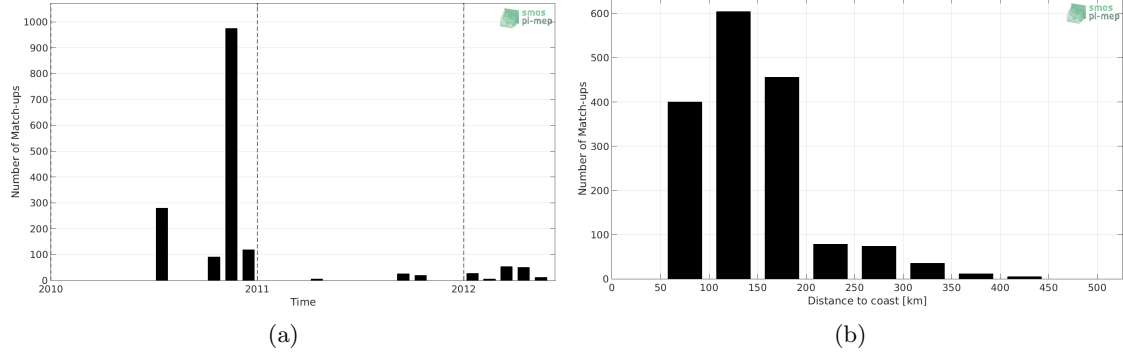
Figure 1: Number of match-ups between Surface drifters and SMOS L3 v2 - Monthly - 0.25 Deg (CATDS-CECOS-IFREMER) SSS as a function of time (a) and as function of the distance to coast (b) over the Arctic Ocean Pi-MEP region and for the full satellite product period.
