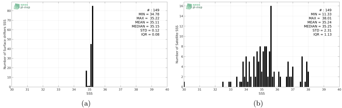
Figure 2: Histograms of SSS from Surface drifters (a) and SMOS-L3-CATDS-IFREMER-CECOS-V2-MONTHLY-0.25DEG (b) considering all match-up pairs per bins of 0.1 over the Arctic Ocean Pi-MEP region and for the full satellite product period.
