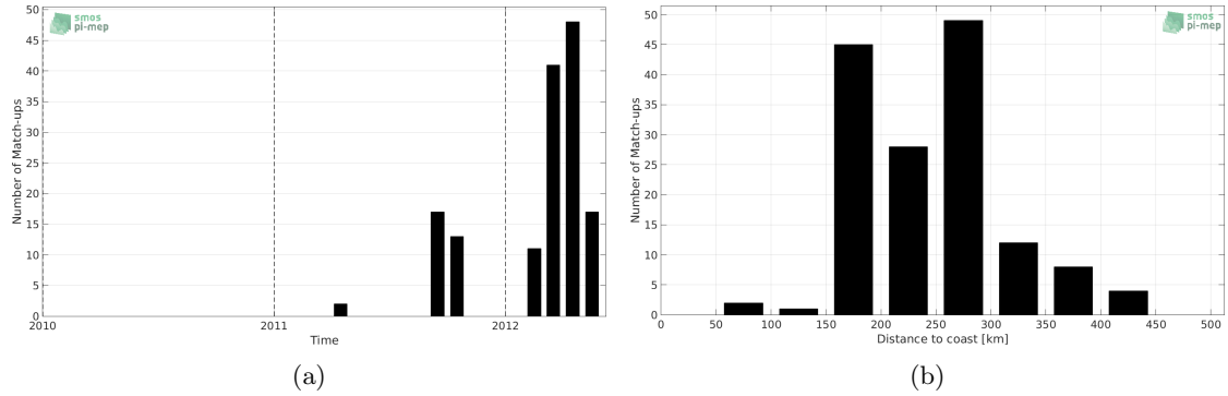
Figure 1: Number of match-ups between Surface drifters and SMOS-L3-CATDS-IFREMER-CECOS-V2-MONTHLY-0.25DEG SSS as a function of time (a) and as function of the distance to coast (b) over the Arctic Ocean Pi-MEP region and for the full satellite product period.
