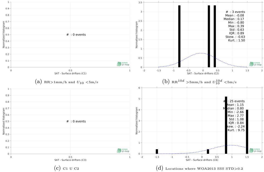
Figure 12: Normalized histogram of \Delta\text{SSS} (SMOS-L3-CATDS-IFREMER-CECOS-V2-MONTHLY-0.25DEG - Surface drifters) for 6 different subdatasets corresponding to: RR > 1\text{mm/h} and U_{10} < 5\text{m/s} (a), RR^{10d} > 5\text{mm/h} and U_{10}^{10d} < 5\text{m/s} (b), C1 U C2 (c), Locations where WOA2013 SSS STD > 0.2 (d).
