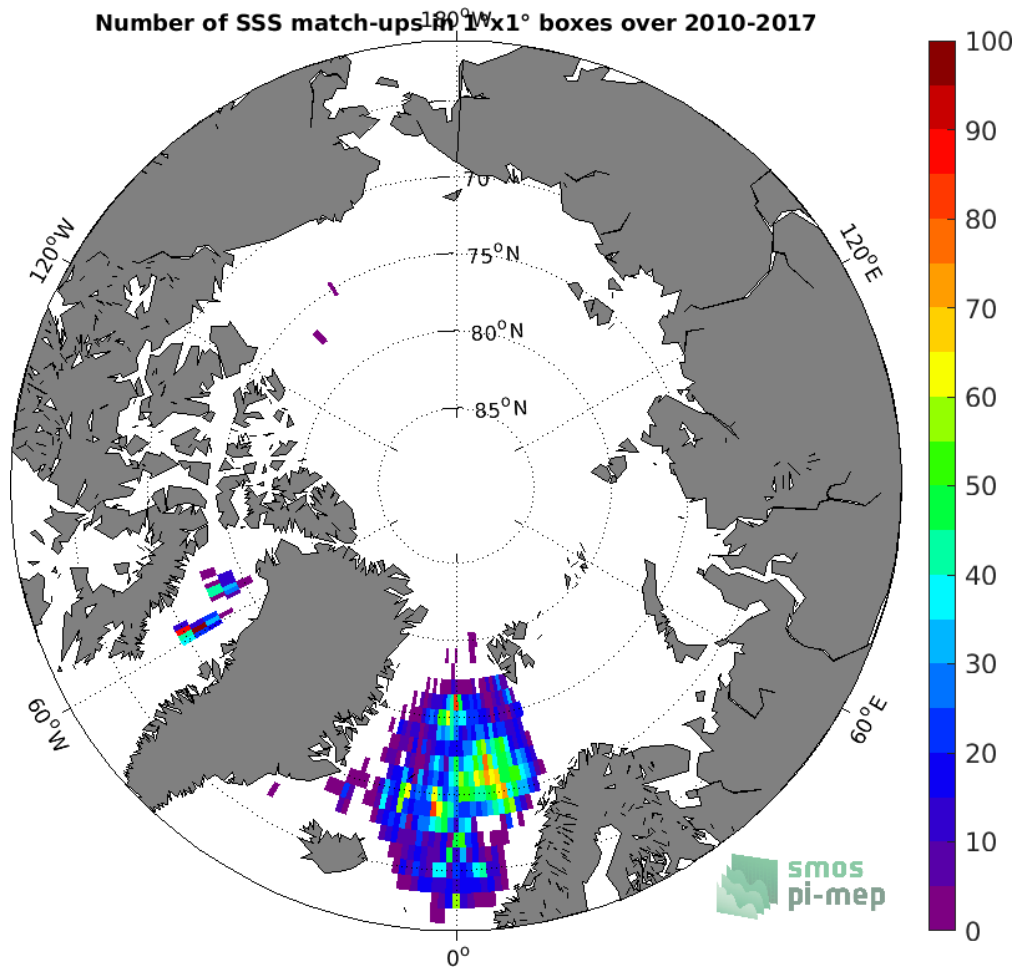
Figure 4: Number of SSS match-ups between Argo SSS and the SMOS SSS L3 v2 - Monthly - 0.25 Deg (CATDS-CECOS-IFREMER) SSS product for the Arctic Ocean Pi-MEP region over 1°x1° boxes and for the full satellite product period.
