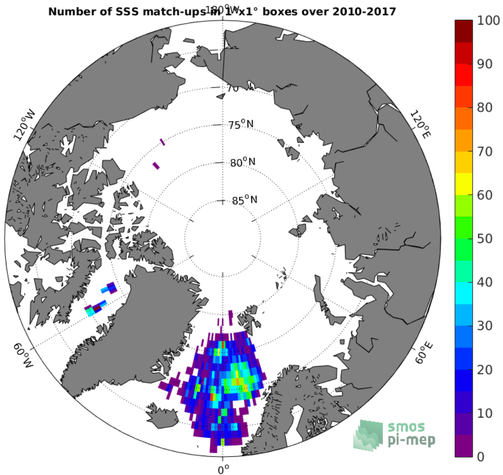
Figure 4: Number of SSS match-ups between Argo SSS and the SMOS-L3-CATDS-IFREMER-CECOS-V2-MONTHLY-0.25DEG SSS product for the Arctic Ocean Pi-MEP region over 1^\circ \times 1^\circ boxes and for the full satellite product period.
