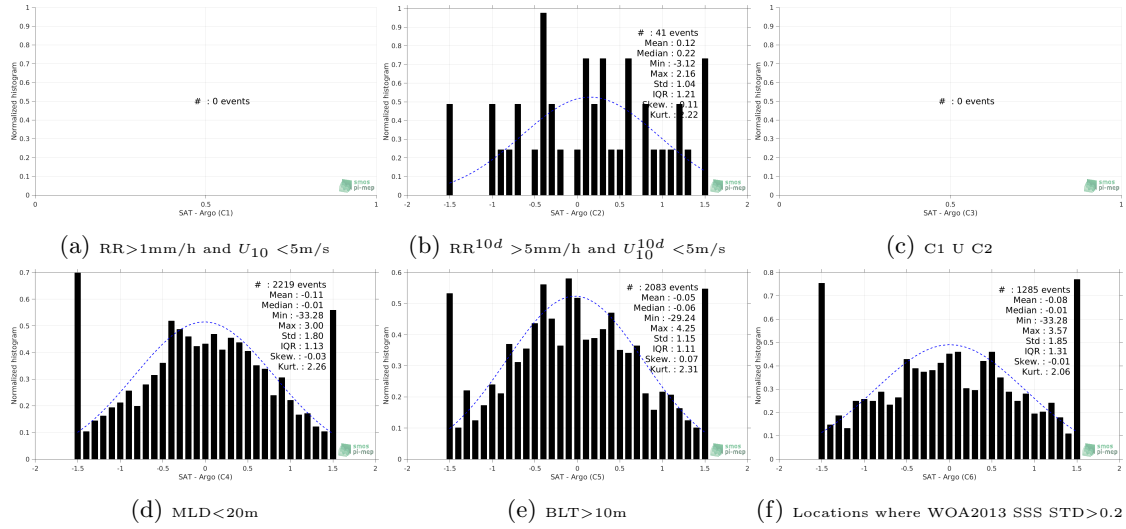
Figure 13: Normalized histogram of \Delta SSS (SMOS-L3-CATDS-IFREMER-CECOS-V2-MONTHLY-0.25DEG - Argo) for 6 different subdatasets corresponding to: RR>1mm/h and U_{10} < 5\text{m/s} (a), RR^{10d} > 5\text{mm/h} and U_{10}^{10d} < 5\text{m/s} (b), C1 U C2 (c),MLD<20m (d),BLT>10m (e),Locations where WOA2013 SSS STD>0.2 (f).
