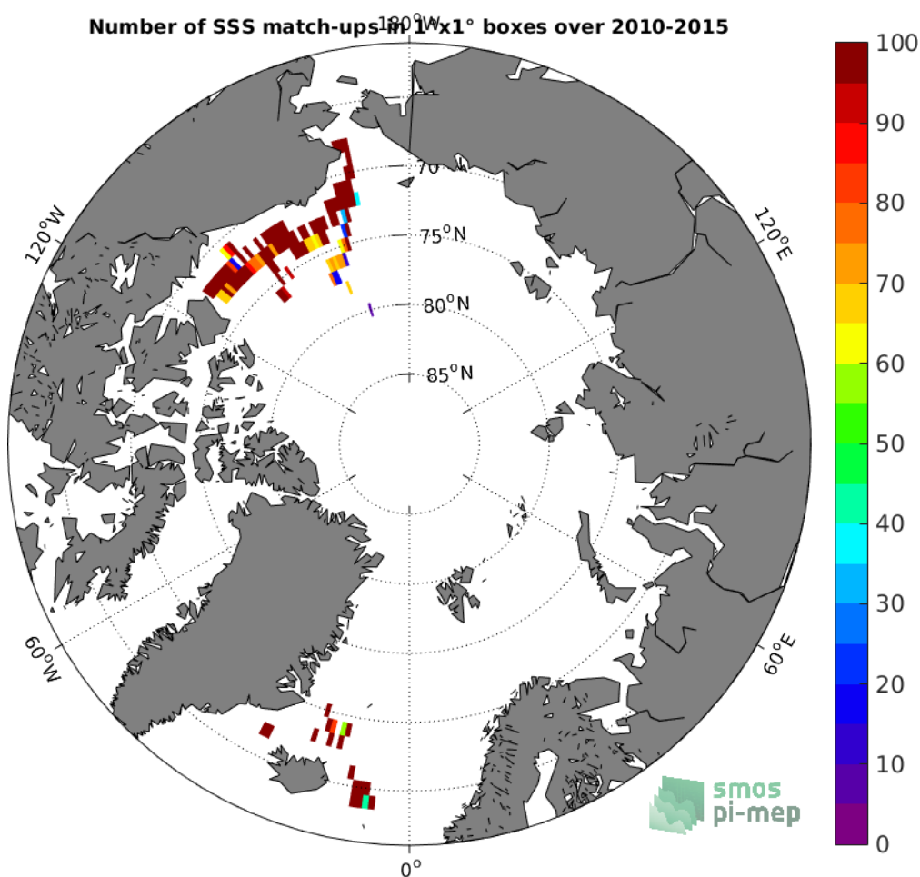
Figure 4: Number of SSS match-ups between TSG-SAMOS SSS and the SMOS-L3-CATDS-CECOS-IFREMER-V2-1DAY-0.5DEG SSS product for the Arctic Ocean Pi-MEP region over 1°x1° boxes and for the full satellite product period.
