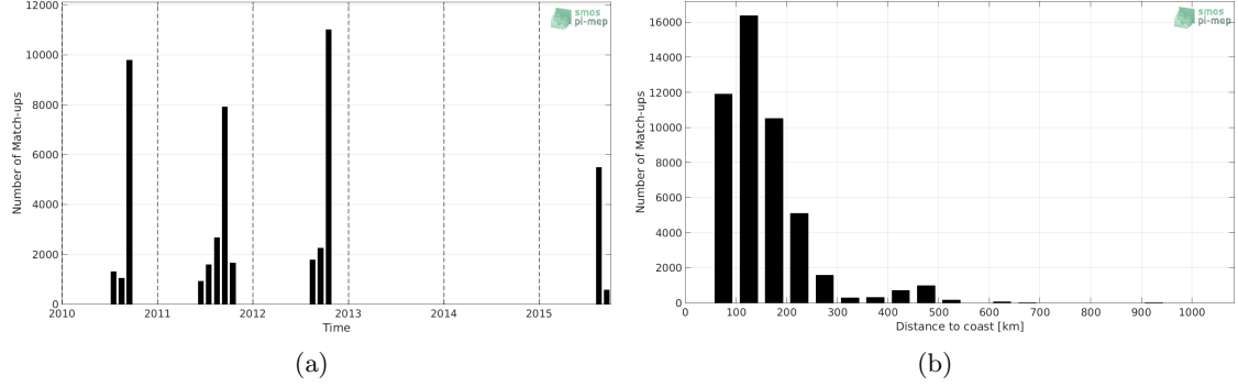
Figure 1: Number of match-ups between TSG-SAMOS and SMOS-L3-CATDS-CECOS-IFREMER-V2-1DAY-0.5DEG SSS as a function of time (a) and as function of the distance to coast (b) over the Arctic Ocean Pi-MEP region and for the full satellite product period.
