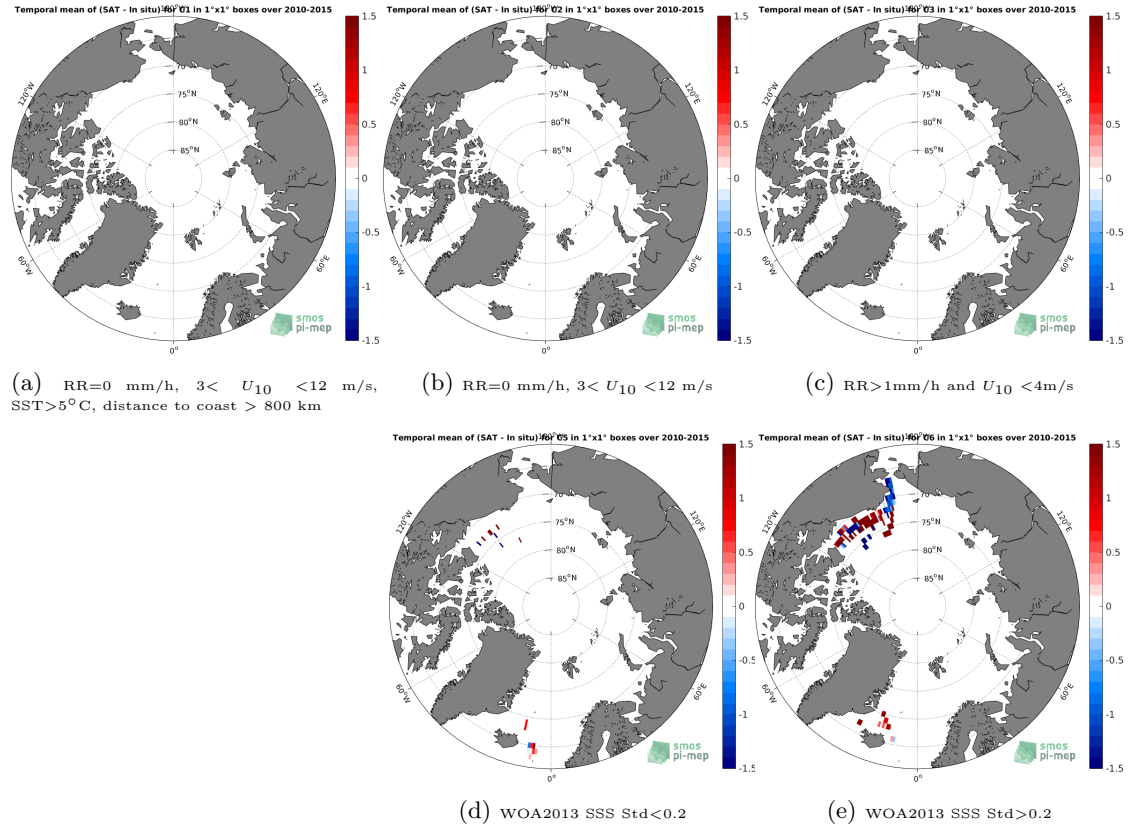
Figure 12: Temporal mean gridded over spatial boxes of size 1^\circ \times 1^\circ of \Delta SSS (SMOS-L3-CATDS-CECOS-IFREMER-V2-1DAY-0.5DEG - TSG-SAMOS) for 5 different subdatasets corresponding to: RR=0 mm/h, 3 < U_{10} < 12 m/s, SST >5^\circ\text{C} , distance to coast > 800 km (a), RR=0 mm/h, 3 < U_{10} < 12 m/s (b), RR >1 mm/h and U_{10} < 4 m/s (c), WOA2013 SSS Std <0.2 (d), WOA2013 SSS Std >0.2 (e).
