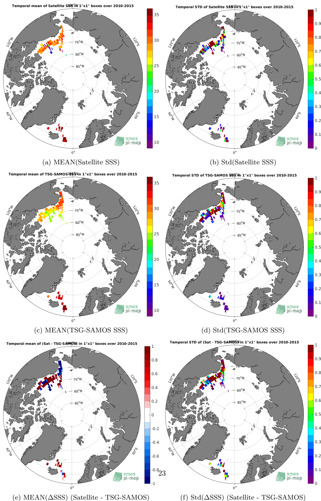
Figure 6: Temporal mean (left) and Std (right) of SSS from SMOS-L3-CATDS-CECOS-IFREMER-V2-1DAY-0.5DEG (top), TSG-SAMOS (middle), and of \Delta SSS (Satellite - TSG-SAMOS). Only match-up pairs are used to generate these maps.
