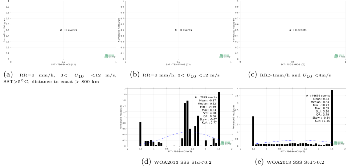
Figure 13: Normalized histogram of \Delta\text{SSS} (SMOS-L3-CATDS-CECOS-IFREMER-V2-1DAY-0.5DEG - TSG-SAMOS) for 5 different subdatasets corresponding to: RR=0 mm/h, 3 < U_{10} < 12 m/s, SST >5^{\circ}\text{C} , distance to coast > 800 km (a), RR=0 mm/h, 3 < U_{10} < 12 m/s (b), RR>1\text{mm/h} and U_{10} < 4\text{m/s} (c), WOA2013 SSS Std <0.2 (d), WOA2013 SSS Std >0.2 (e).
