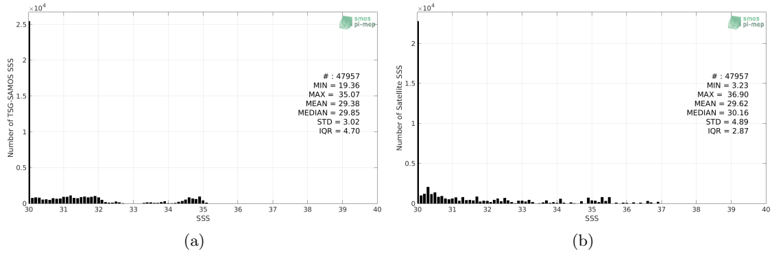
Figure 2: Histograms of SSS from TSG-SAMOS (a) and SMOS-L3-CATDS-CECOS-IFREMER-V2-1DAY-0.5DEG (b) considering all match-up pairs per bins of 0.1 over the Arctic Ocean Pi-MEP region and for the full satellite product period.
