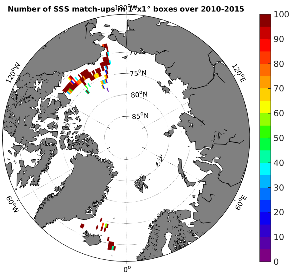
Figure 4: Number of SSS match-ups between TSG-SAMOS SSS and the SMOS-L3-CATDS-CECOS-IFREMER-V2-1DAY-0.5deg SSS product for the Arctic Ocean Pi-MEP region over 1^\circ \times 1^\circ boxes and for the full satellite product period.
