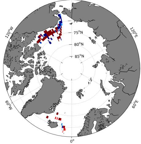
(e) MEAN( \Delta SSS) (Satellite - TSG-SAMOS)
