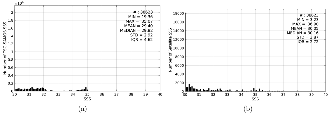
Figure 2: Histograms of SSS from TSG-SAMOS (a) and SMOS-L3-CATDS-CECOS-IFREMER-V2-1DAY-0.5deg (b) considering all match-up pairs per bins of 0.1 over the Arctic Ocean Pi-MEP region and for the full satellite product period.
