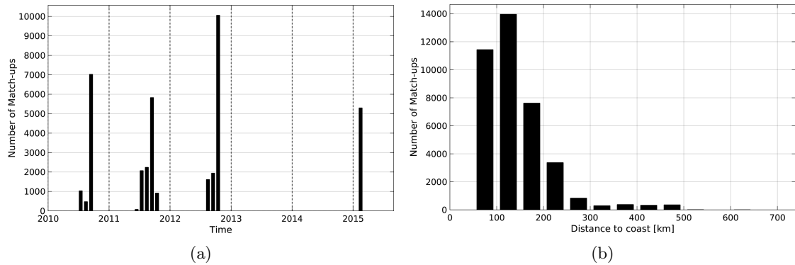
Figure 1: Number of match-ups between TSG-SAMOS and SMOS-L3-CATDS-CECOS-IFREMER-V2-1DAY-0.5deg SSS as a function of time (a) and as function of the distance to coast (b) over the Arctic Ocean Pi-MEP region and for the full satellite product period.
