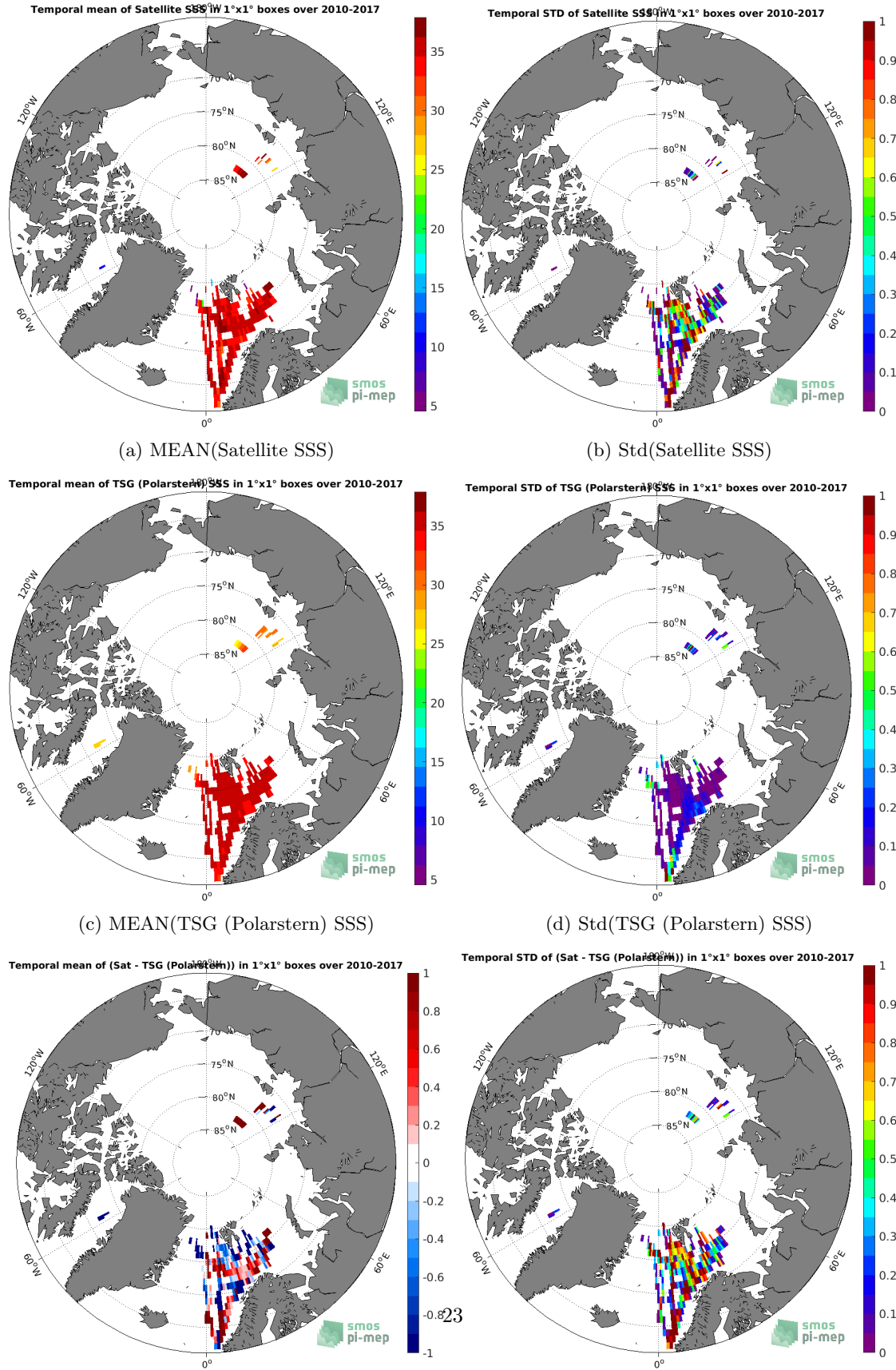
Figure 6: Temporal mean (left) and Std (right) of SSS from SMOS SSS L3 v2 - Daily - 0.5 Deg (CATDS-CECOS-IFREMER) (top), TSG (Polarstern) (middle), and of \Delta SSS (Satellite - TSG (Polarstern)). Only match-up pairs are used to generate these maps.
