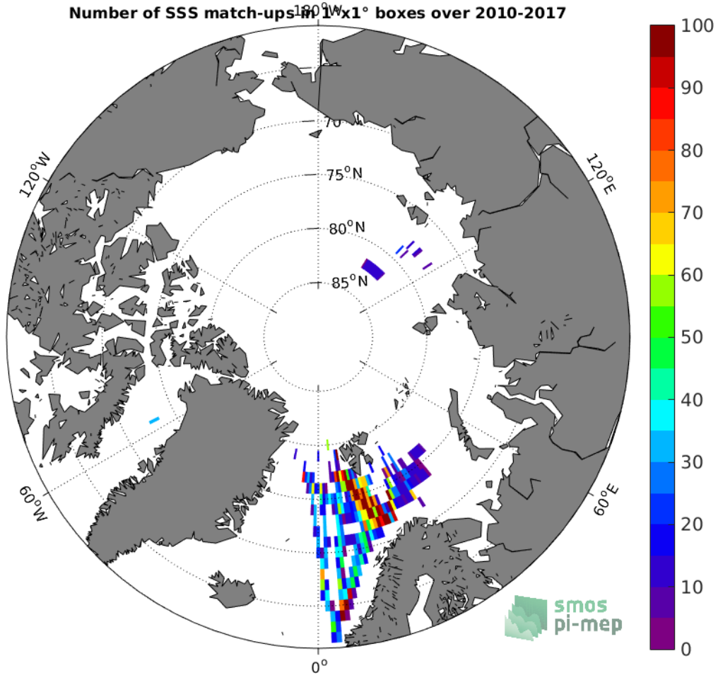
Figure 4: Number of SSS match-ups between TSG (Polarstern) SSS and the SMOS SSS L3 v2 - Daily - 0.5 Deg (CATDS-CECOS-IFREMER) SSS product for the Arctic Ocean Pi-MEP region over 1°x1° boxes and for the full satellite product period.
