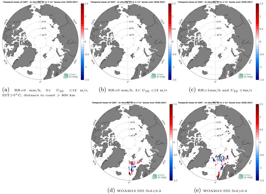
Figure 12: Temporal mean gridded over spatial boxes of size 1^{\circ}\times 1^{\circ} of \Delta\text{SSS} (SMOS SSS L3 v2 - Daily - 0.5 Deg (CATDS-CECOS-IFREMER) - TSG (Polarstern)) for 5 different subdatasets corresponding to: RR=0 mm/h, 3 < U_{10} < 12 m/s, SST >5^{\circ}\text{C} , distance to coast > 800 km (a), RR=0 mm/h, 3 < U_{10} < 12 m/s (b), RR >1 mm/h and U_{10} < 4 m/s (c), WOA2013 SSS Std <0.2 (d), WOA2013 SSS Std >0.2 (e).
