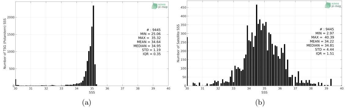
Figure 2: Histograms of SSS from TSG (Polarstern) (a) and SMOS SSS L3 v2 - Daily - 0.5 Deg (CATDS-CECOS-IFREMER) (b) considering all match-up pairs per bins of 0.1 over the Arctic Ocean Pi-MEP region and for the full satellite product period.
