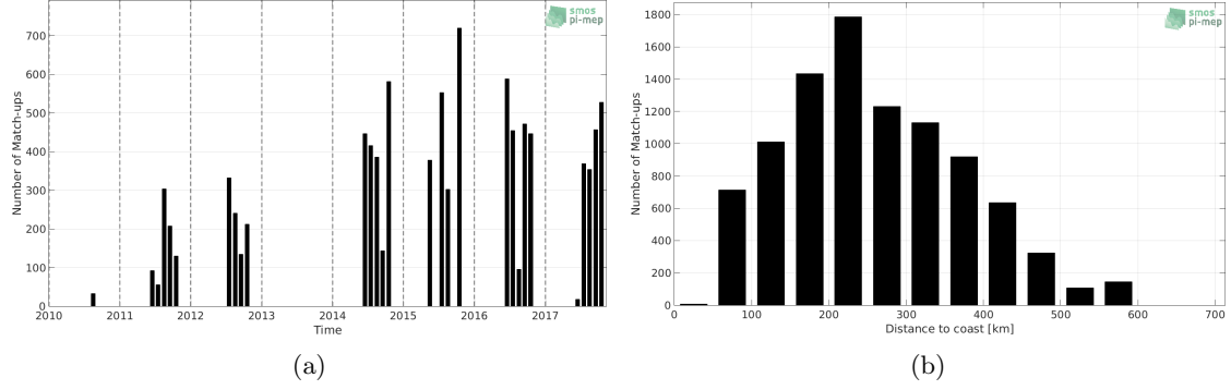
Figure 1: Number of match-ups between TSG (Polarstern) and SMOS SSS L3 v2 - Daily - 0.5 Deg (CATDS-CECOS-IFREMER) SSS as a function of time (a) and as function of the distance to coast (b) over the Arctic Ocean Pi-MEP region and for the full satellite product period.
