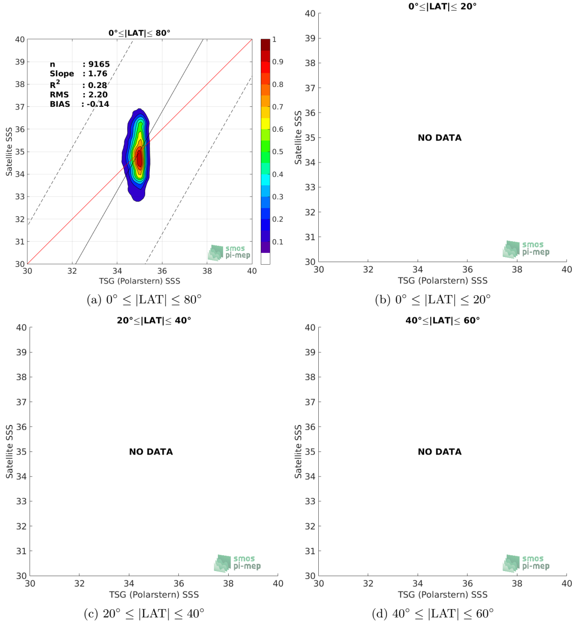
Figure 9: Contour maps of the concentration of SMOS SSS L3 v2 - Daily - 0.5 Deg (CATDS-CECOS-IFREMER) SSS (y-axis) versus TSG (Polarstern) SSS (x-axis) at match-up pairs for different latitude bands. For each plot, the red line shows x=y . The black thin and dashed lines indicate a linear fit through the data cloud and the \pm 95\% confidence levels, respectively. The number match-up pairs n , the slope and R^2 coefficient of the linear fit, the root mean square (RMS) and the mean bias between satellite and in situ data are indicated for each latitude band in each plots.
