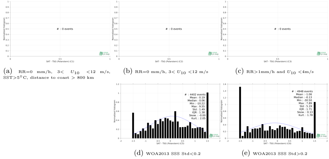
Figure 13: Normalized histogram of \Delta\text{SSS} (SMOS SSS L3 v2 - Daily - 0.5 Deg (CATDS-CECOS-IFREMER) - TSG (Polarstern)) for 5 different subdatasets corresponding to: RR=0 mm/h, 3 < U_{10} < 12 m/s, SST > 5^\circ\text{C} , distance to coast > 800 km (a), RR=0 mm/h, 3 < U_{10} < 12 m/s (b), RR > 1\text{mm/h} and U_{10} < 4\text{m/s} (c), WOA2013 SSS Std<0.2 (d), WOA2013 SSS Std>0.2 (e).
