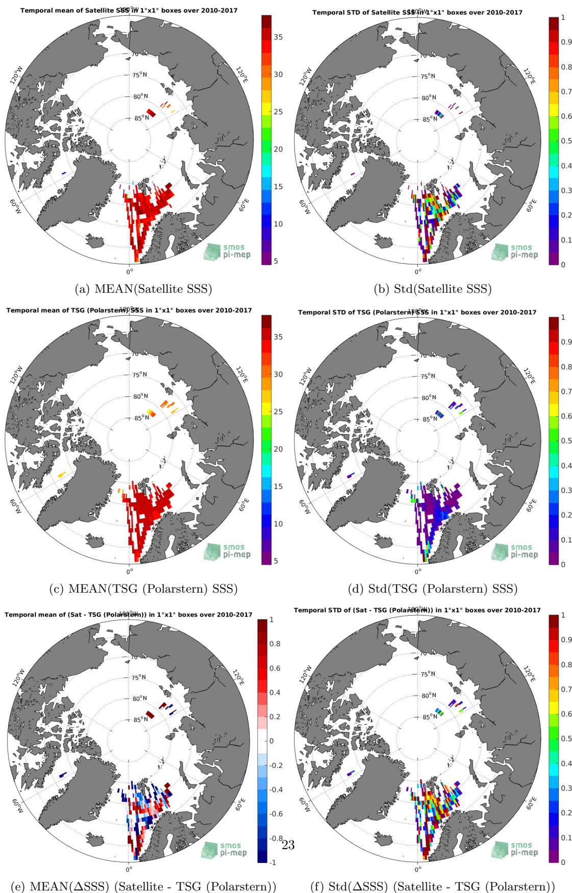
Figure 6: Temporal mean (left) and Std (right) of SSS from SMOS SSS L3 v2 - Daily - 0.5 Deg (CATDS-CECOS-IFREMER) (top), TSG (Polarstern) (middle), and of \Delta SSS (Satellite - TSG (Polarstern)). Only match-up pairs are used to generate these maps.
