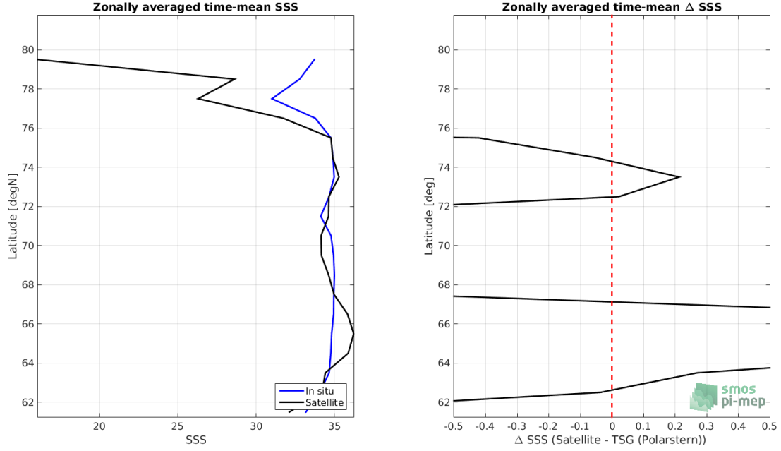
Figure 8: Left panel: Zonal mean SSS from SMOS SSS L3 v2 - Daily - 0.5 Deg (CATDS-CECOS-IFREMER) satellite product (black) and from TSG (Polarstern) (blue). Right panel: Zonal mean of \Delta SSS (Satellite - TSG (Polarstern)) for all the collected Pi-MEP match-up pairs estimated over the full satellite product period.
