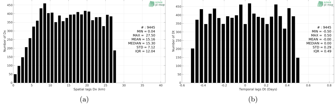
Figure 5: Histograms of the spatial (a) and temporal (b) lags between the time of the TSG (Polarstern) measurements and the date of the corresponding SMOS SSS L3 v2 - Daily - 0.5 Deg (CATDS-CECOS-IFREMER) SSS product.
