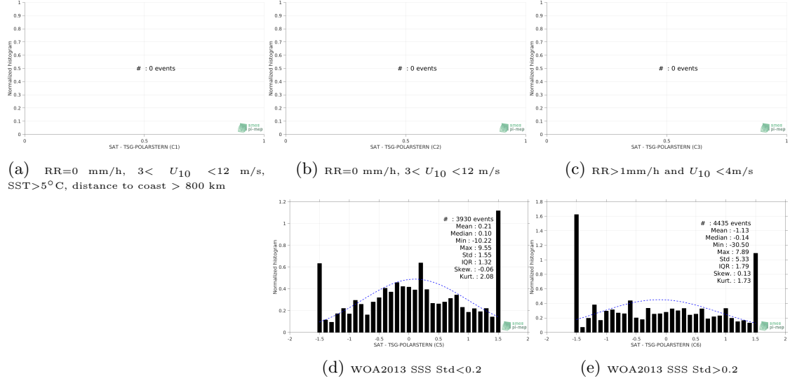
Figure 13: Normalized histogram of \Delta\text{SSS} (SMOS L3 v2 - Daily - 0.5 Deg (CATDS-CECOS-IFREMER) - TSG-POLARSTERN) for 5 different subdatasets corresponding to: RR=0 mm/h, 3 < U_{10} < 12 m/s, SST > 5^\circ\text{C} , distance to coast > 800 km (a), RR=0 mm/h, 3 < U_{10} < 12 m/s (b), RR > 1\text{mm/h} and U_{10} < 4\text{m/s} (c), WOA2013 SSS Std < 0.2 (d), WOA2013 SSS Std > 0.2 (e).
