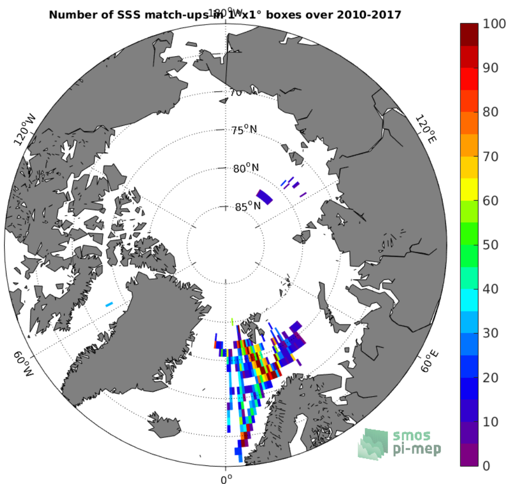
Figure 4: Number of SSS match-ups between TSG-POLARSTERN SSS and the SMOS L3 v2 - Daily - 0.5 Deg (CATDS-CECOS-IFREMER) SSS product for the Arctic Ocean Pi-MEP region over 1^\circ \times 1^\circ boxes and for the full satellite product period.
