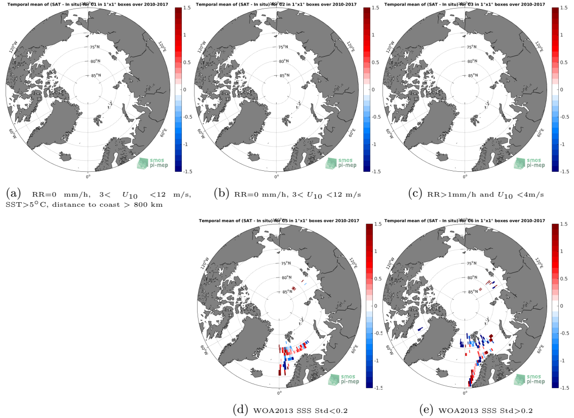
Figure 12: Temporal mean gridded over spatial boxes of size 1^{\circ}\times 1^{\circ} of \Delta\text{SSS} (SMOS L3 v2 - Daily - 0.5 Deg (CATDS-CECOS-IFREMER) - TSG-POLARSTERN) for 5 different subdatasets corresponding to: \text{RR}=0 mm/h, 3 < U_{10} < 12 m/s, \text{SST} > 5^{\circ}\text{C} , distance to coast > 800 km (a), \text{RR}=0 mm/h, 3 < U_{10} < 12 m/s (b), \text{RR} > 1 mm/h and U_{10} < 4 m/s (c), WOA2013 SSS Std < 0.2 (d), WOA2013 SSS Std > 0.2 (e).
