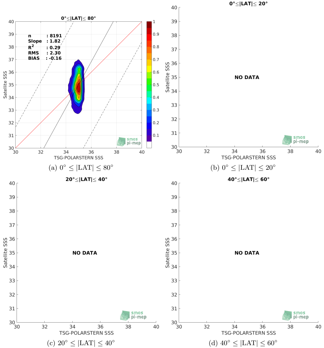
Figure 9: Contour maps of the concentration of SMOS L3 v2 - Daily - 0.5 Deg (CATDS-CECOS-IFREMER) SSS (y-axis) versus TSG-POLARSTERN SSS (x-axis) at match-up pairs for different latitude bands. For each plot, the red line shows x=y . The black thin and dashed lines indicate a linear fit through the data cloud and the \pm 95\% confidence levels, respectively. The number match-up pairs n , the slope and R^2 coefficient of the linear fit, the root mean square (RMS) and the mean bias between satellite and in situ data are indicated for each latitude band in each plots.
