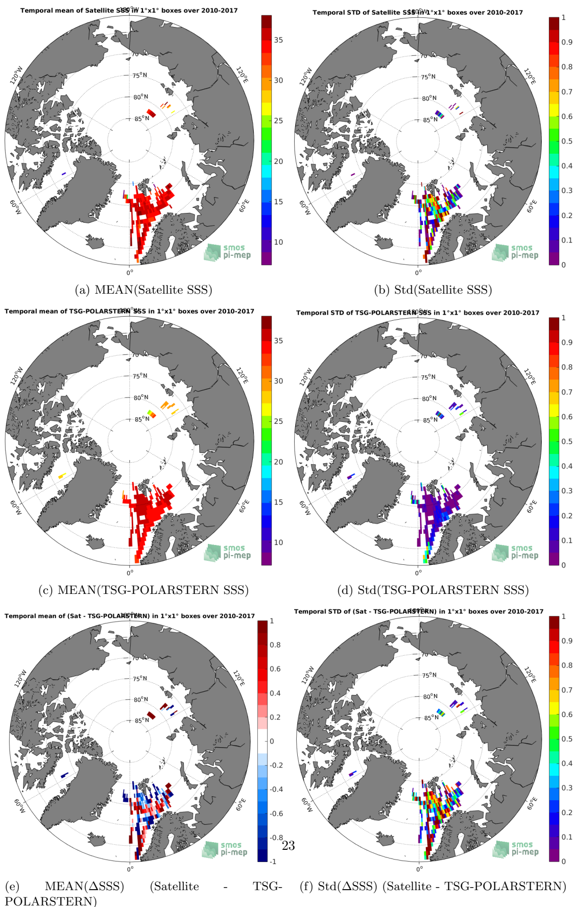
Figure 6: Temporal mean (left) and Std (right) of SSS from SMOS L3 v2 - Daily - 0.5 Deg (CATDS-CECOS-IFREMER) (top), TSG-POLARSTERN (middle), and of \Delta SSS (Satellite - TSG-POLARSTERN). Only match-up pairs are used to generate these maps.
