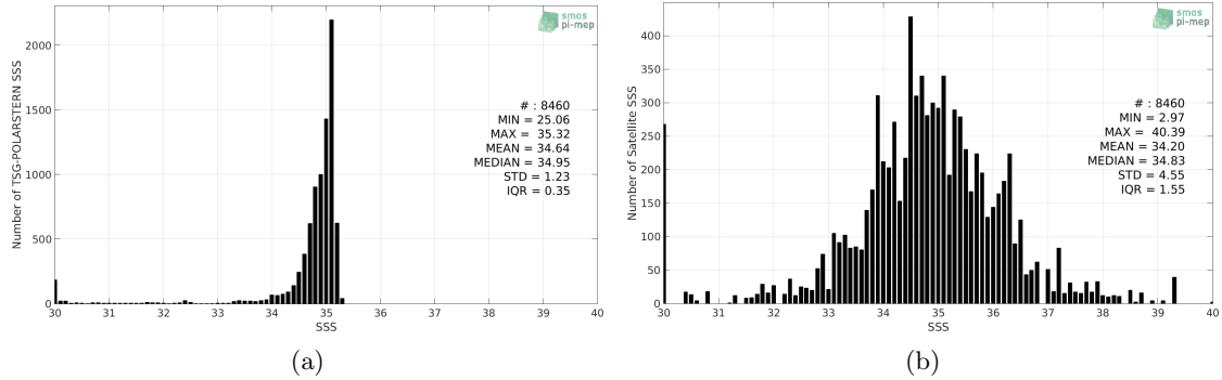
Figure 2: Histograms of SSS from TSG-POLARSTERN (a) and SMOS L3 v2 - Daily - 0.5 Deg (CATDS-CECOS-IFREMER) (b) considering all match-up pairs per bins of 0.1 over the Arctic Ocean Pi-MEP region and for the full satellite product period.
