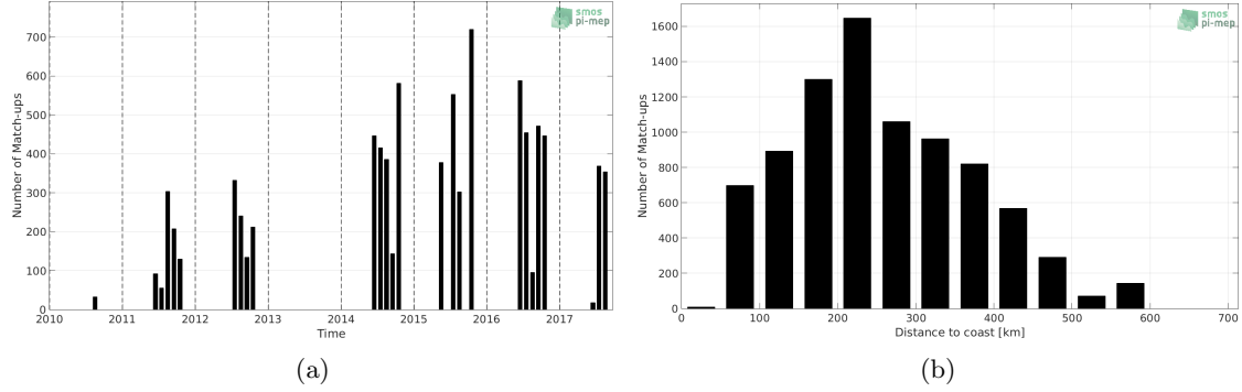
Figure 1: Number of match-ups between TSG-POLARSTERN and SMOS L3 v2 - Daily - 0.5 Deg (CATDS-CECOS-IFREMER) SSS as a function of time (a) and as function of the distance to coast (b) over the Arctic Ocean Pi-MEP region and for the full satellite product period.
