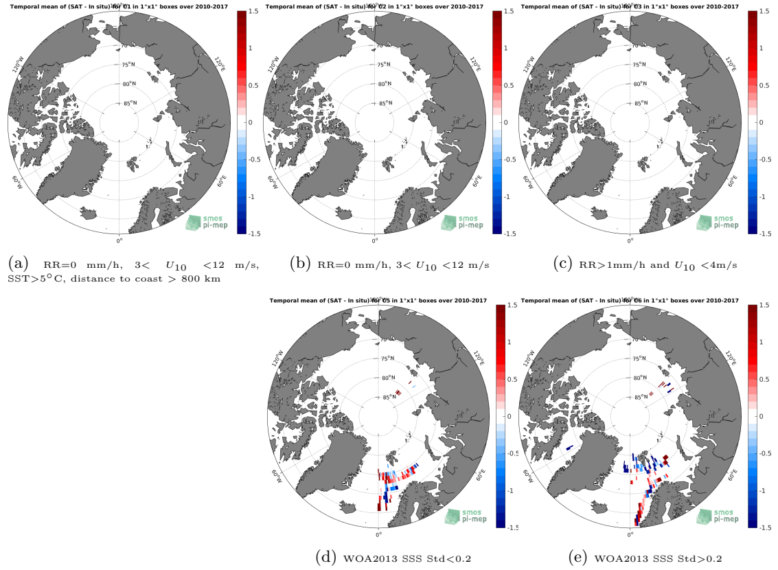
Figure 12: Temporal mean gridded over spatial boxes of size 1^\circ \times 1^\circ of \Delta SSS (SMOS-L3-CATDS-CECOS-IFREMER-V2-1DAY-0.5DEG - TSG-POLARSTERN) for 5 different subdatasets corresponding to: RR=0 mm/h, 3 < U_{10} < 12 m/s, SST > 5^\circ C , distance to coast > 800 km (a), RR=0 mm/h, 3 < U_{10} < 12 m/s (b), RR > 1 mm/h and U_{10} < 4 m/s (c), WOA2013 SSS Std < 0.2 (d), WOA2013 SSS Std > 0.2 (e).
