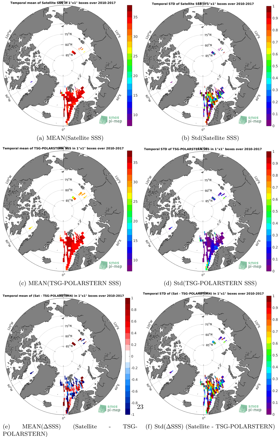
Figure 6: Temporal mean (left) and Std (right) of SSS from SMOS-L3-CATDS-CECOS-IFREMER-V2-1DAY-0.5DEG (top), TSG-POLARSTERN (middle), and of \Delta SSS (Satellite - TSG-POLARSTERN). Only match-up pairs are used to generate these maps.
