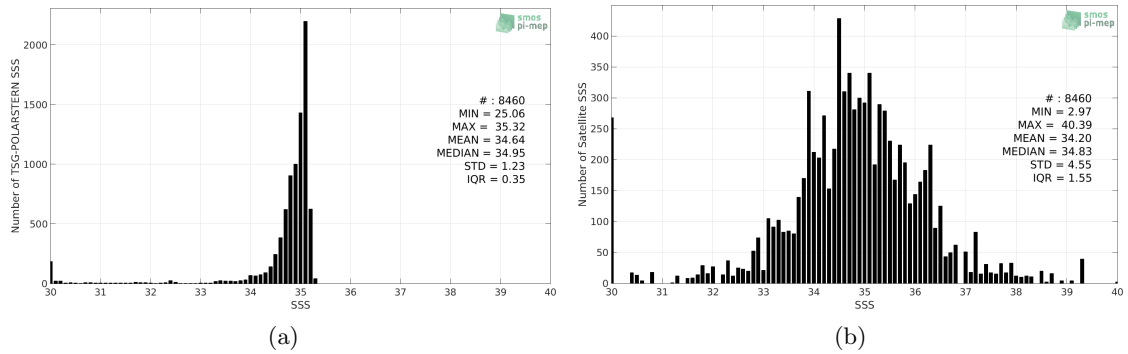
Figure 2: Histograms of SSS from TSG-POLARSTERN (a) and SMOS-L3-CATDS-CECOS-IFREMER-V2-1DAY-0.5DEG (b) considering all match-up pairs per bins of 0.1 over the Arctic Ocean Pi-MEP region and for the full satellite product period.
