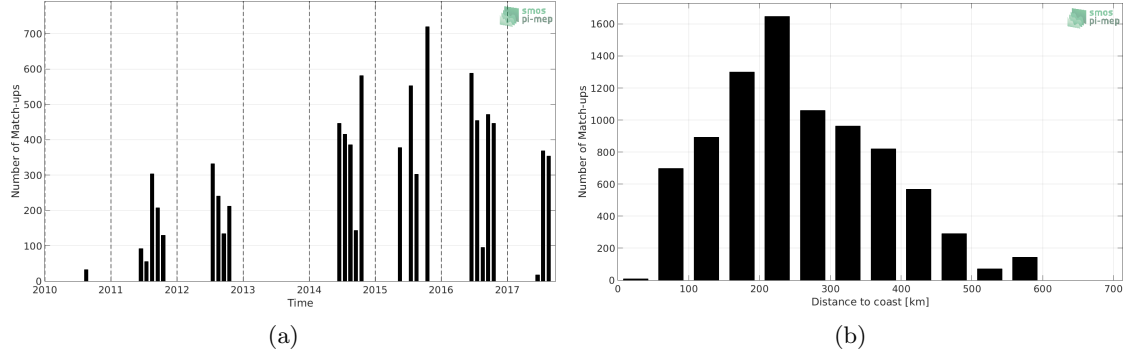
Figure 1: Number of match-ups between TSG-POLARSTERN and SMOS-L3-CATDS-CECOS-IFREMER-V2-1DAY-0.5DEG SSS as a function of time (a) and as function of the distance to coast (b) over the Arctic Ocean Pi-MEP region and for the full satellite product period.
