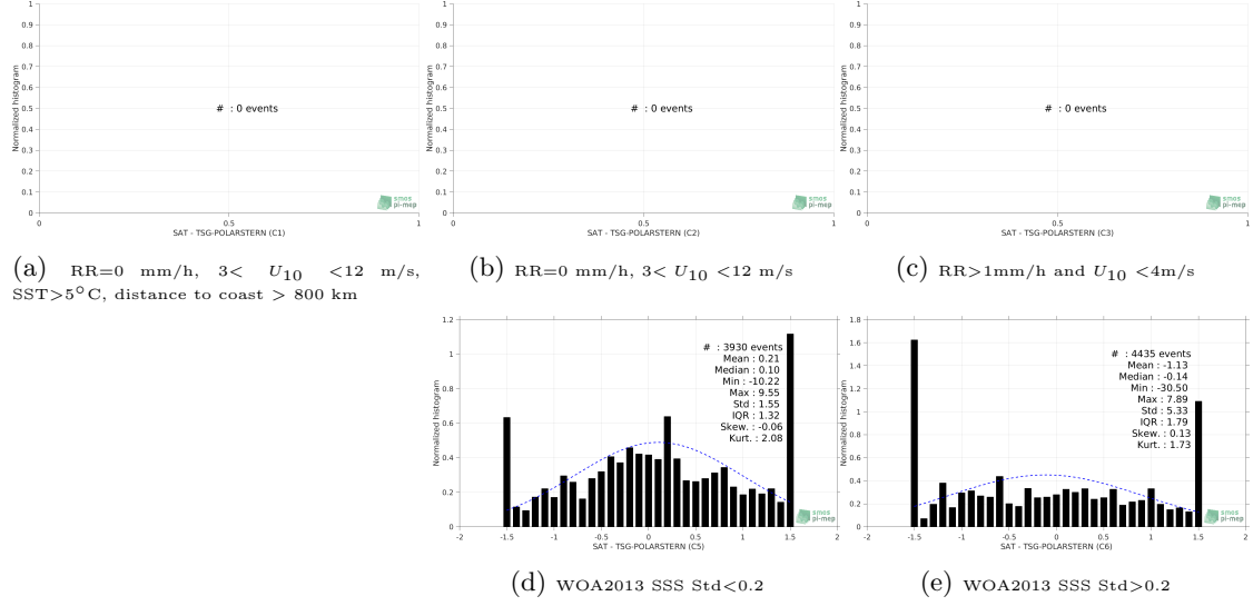
Figure 13: Normalized histogram of \Delta\text{SSS} (SMOS-L3-CATDS-CECOS-IFREMER-V2-1DAY-0.5DEG - TSG-POLARSTERN) for 5 different subdatasets corresponding to: RR=0 mm/h, 3 < U_{10} < 12 m/s, SST > 5^\circ\text{C} , distance to coast > 800 km (a), RR=0 mm/h, 3 < U_{10} < 12 m/s (b), RR > 1\text{mm/h} and U_{10} < 4\text{m/s} (c), WOA2013 SSS Std <0.2 (d), WOA2013 SSS Std >0.2 (e).
