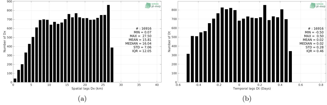
Figure 5: Histograms of the spatial (a) and temporal (b) lags between the location/time of the TSG (LEGOS-DM) measurement and the date of the corresponding SMOS SSS L3 v2 - Daily - 0.5 Deg (CATDS-CECOS-IFREMER) SSS pixel.
