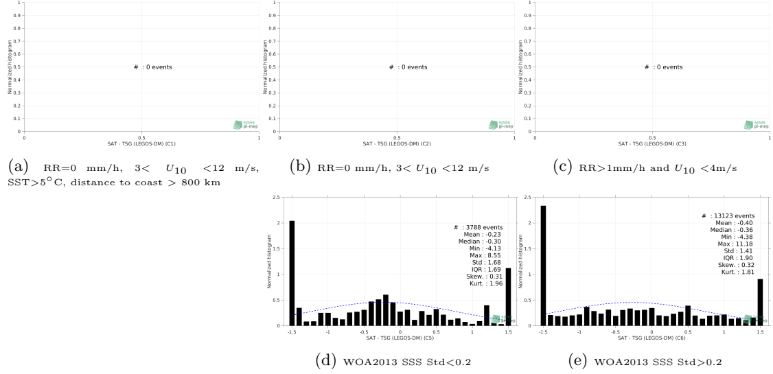
Figure 13: Normalized histogram of \Delta\text{SSS} (SMOS SSS L3 v2 - Daily - 0.5 Deg (CATDS-CECOS-IFREMER) - TSG (LEGOS-DM)) for 5 different subdatasets corresponding to: RR=0 mm/h, 3 < U_{10} < 12 m/s, SST > 5^\circ\text{C} , distance to coast > 800 km (a), RR=0 mm/h, 3 < U_{10} < 12 m/s (b), RR > 1\text{mm/h} and U_{10} < 4\text{m/s} (c), WOA2013 SSS Std<0.2 (d), WOA2013 SSS Std>0.2 (e).
