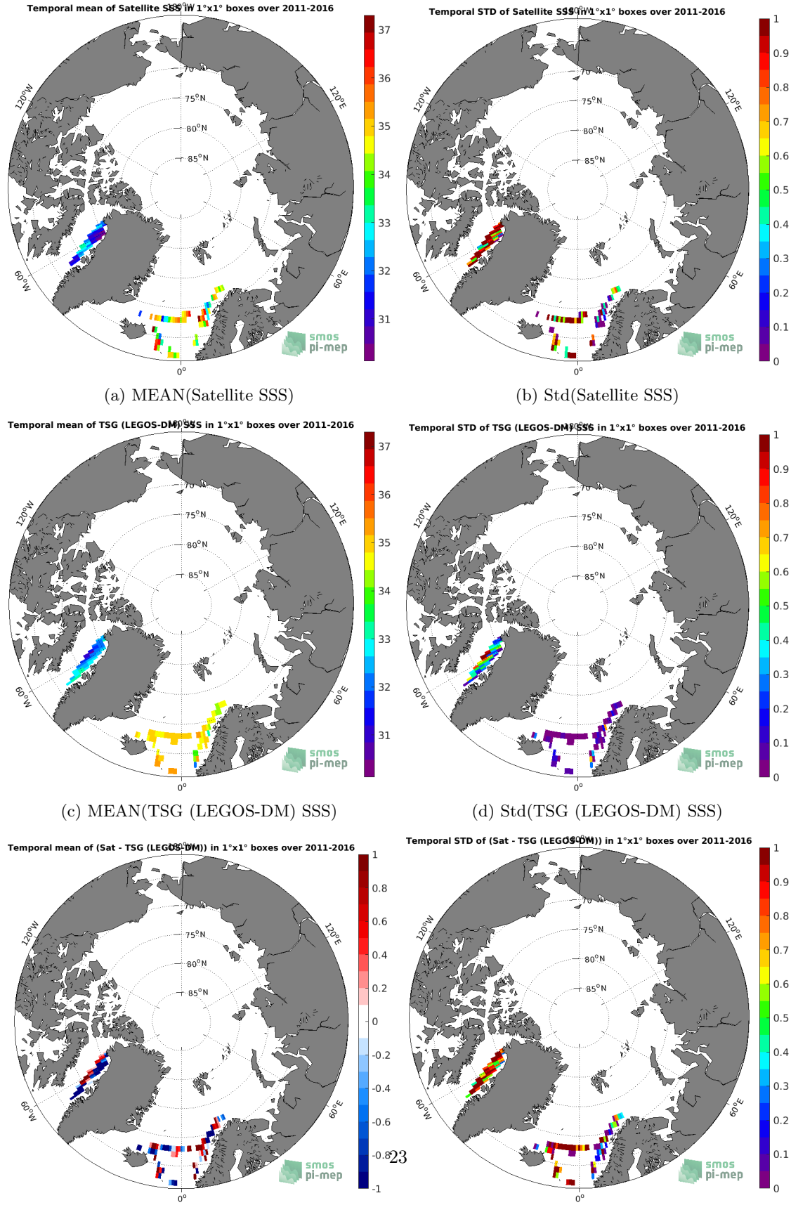
Figure 6: Temporal mean (left) and Std (right) of SSS from SMOS SSS L3 v2 - Daily - 0.5 Deg (CATDS-CECOS-IFREMER) (top), TSG (LEGOS-DM) (middle), and of \Delta SSS (Satellite - TSG (LEGOS-DM)). Only match-up pairs are used to generate these maps.
