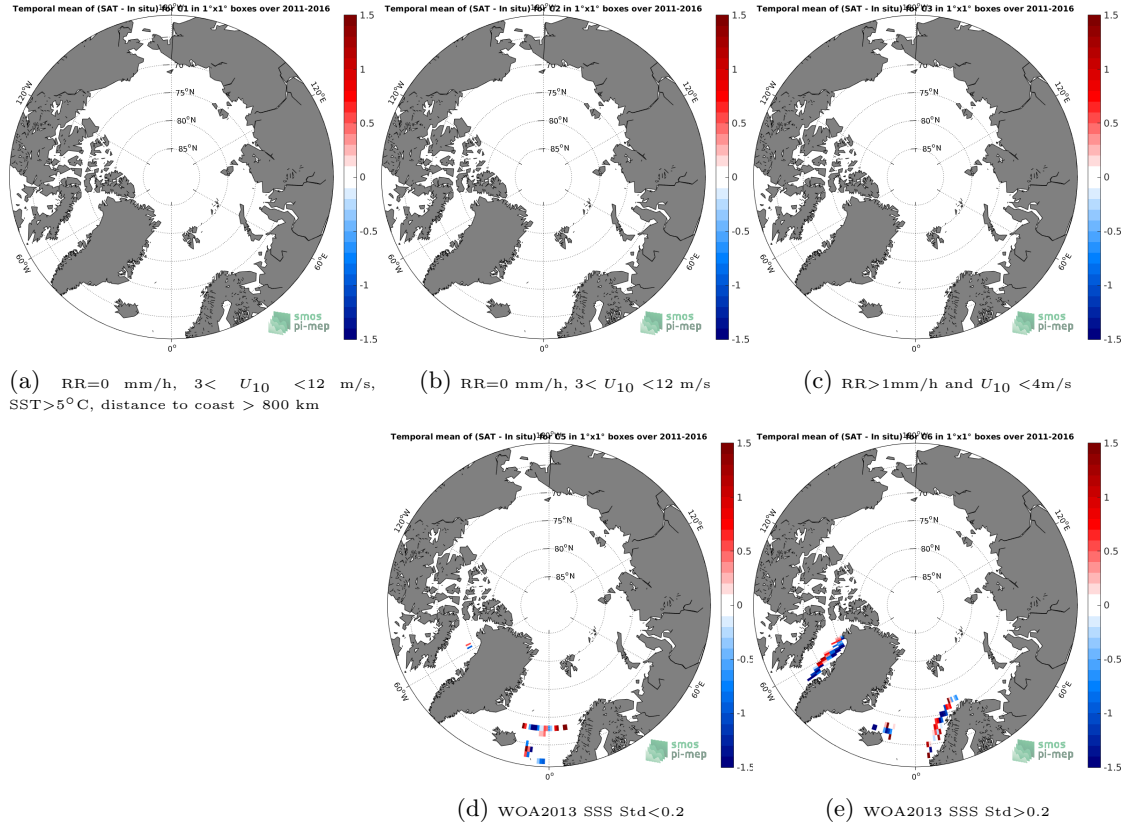
Figure 12: Temporal mean gridded over spatial boxes of size 1^{\circ}\times 1^{\circ} of \Delta\text{SSS} (SMOS SSS L3 v2 - Daily - 0.5 Deg (CATDS-CECOS-IFREMER) - TSG (LEGOS-DM)) for 5 different subdatasets corresponding to: RR=0 mm/h, 3 < U_{10} < 12 m/s, SST >5^{\circ}\text{C} , distance to coast > 800 km (a), RR=0 mm/h, 3 < U_{10} < 12 m/s (b), RR >1 mm/h and U_{10} < 4 m/s (c), WOA2013 SSS Std <0.2 (d), WOA2013 SSS Std >0.2 (e).
