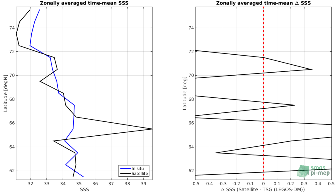
Figure 8: Left panel: Zonal mean SSS from SMOS SSS L3 v2 - Daily - 0.5 Deg (CATDS-CECOS-IFREMER) satellite product (black) and from TSG (LEGOS-DM) (blue). Right panel: Zonal mean of \Delta SSS (Satellite - TSG (LEGOS-DM)) for all the collected Pi-MEP match-up pairs estimated over the full satellite product period.
