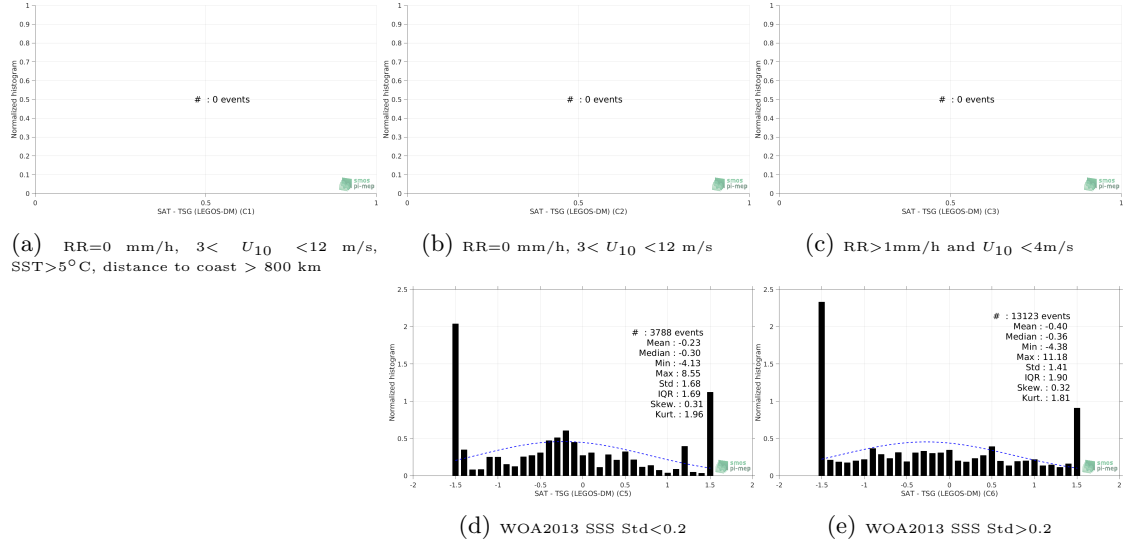
Figure 13: Normalized histogram of \Delta\text{SSS} (SMOS SSS L3 v2 - Daily - 0.5 Deg (CATDS-CECOS-IFREMER) - TSG (LEGOS-DM)) for 5 different subdatasets corresponding to: RR=0 mm/h, 3 < U_{10} < 12 m/s, SST > 5^\circ\text{C} , distance to coast > 800 km (a), RR=0 mm/h, 3 < U_{10} < 12 m/s (b), RR > 1\text{mm/h} and U_{10} < 4\text{m/s} (c), WOA2013 SSS Std<0.2 (d), WOA2013 SSS Std>0.2 (e).
