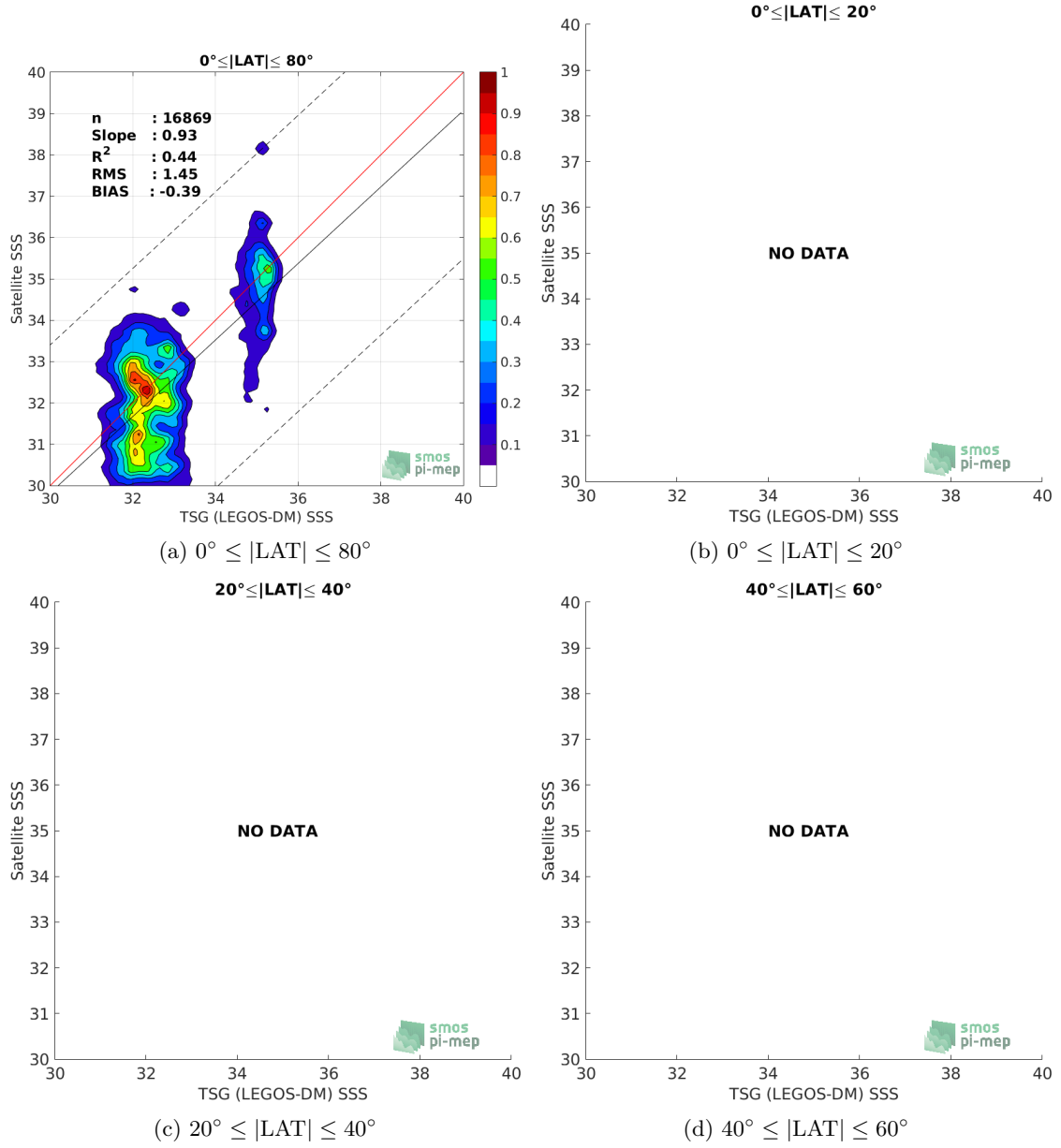
Figure 9: Contour maps of the concentration of SMOS SSS L3 v2 - Daily - 0.5 Deg (CATDS-CECOS-IFREMER) SSS (y-axis) versus TSG (LEGOS-DM) SSS (x-axis) at match-up pairs for different latitude bands. For each plot, the red line shows x=y . The black thin and dashed lines indicate a linear fit through the data cloud and the \pm 95\% confidence levels, respectively. The number match-up pairs n , the slope and R^2 coefficient of the linear fit, the root mean square (RMS) and the mean bias between satellite and in situ data are indicated for each latitude band in each plots.
