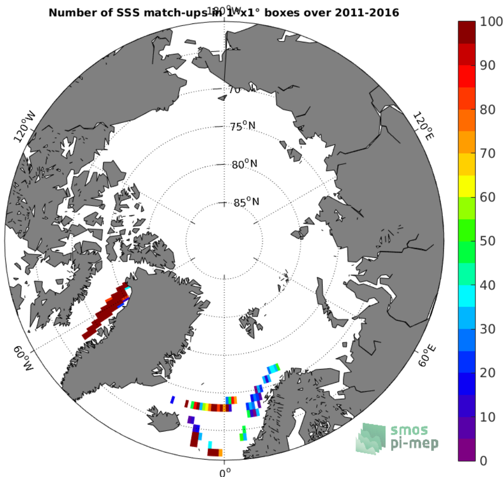
Figure 4: Number of SSS match-ups between TSG (LEGOS-DM) SSS and the SMOS SSS L3 v2 - Daily - 0.5 Deg (CATDS-CECOS-IFREMER) SSS product for the Arctic Ocean Pi-MEP region over 1°x1° boxes and for the full satellite product period.
