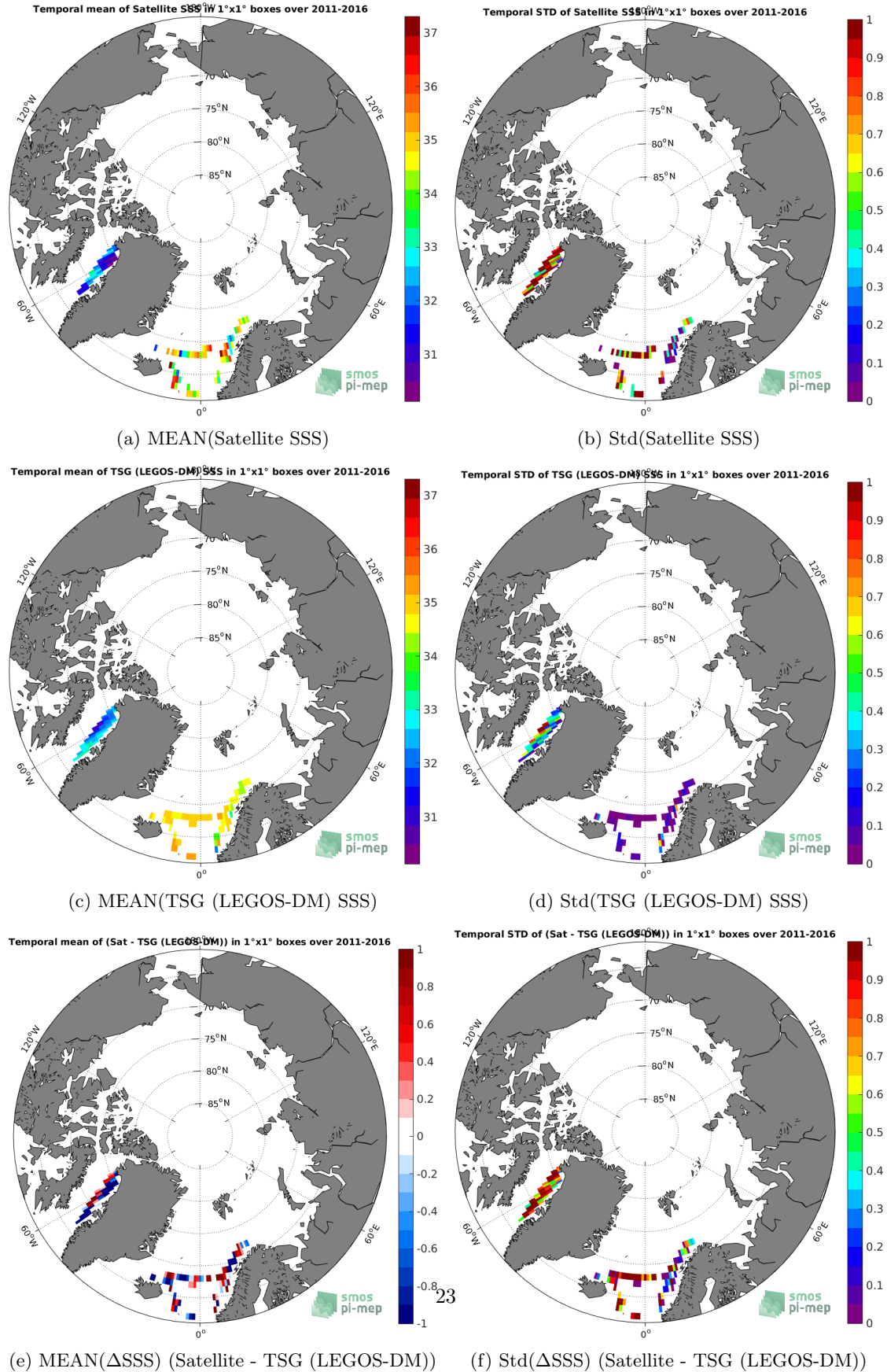
Figure 6: Temporal mean (left) and Std (right) of SSS from SMOS SSS L3 v2 - Daily - 0.5 Deg (CATDS-CECOS-IFREMER) (top), TSG (LEGOS-DM) (middle), and of \Delta SSS (Satellite - TSG (LEGOS-DM)). Only match-up pairs are used to generate these maps.
