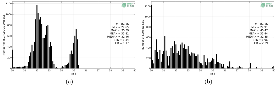
Figure 2: Histograms of SSS from TSG (LEGOS-DM) (a) and SMOS SSS L3 v2 - Daily - 0.5 Deg (CATDS-CECOS-IFREMER) (b) considering all match-up pairs per bins of 0.1 over the Arctic Ocean Pi-MEP region and for the full satellite product period.
