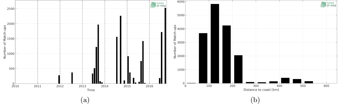
Figure 1: Number of match-ups between TSG (LEGOS-DM) and SMOS SSS L3 v2 - Daily - 0.5 Deg (CATDS-CECOS-IFREMER) SSS as a function of time (a) and as function of the distance to coast (b) over the Arctic Ocean Pi-MEP region and for the full satellite product period.
