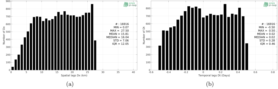
Figure 5: Histograms of the spatial (a) and temporal (b) lags between the time of the TSG (LEGOS-DM) measurements and the date of the corresponding SMOS SSS L3 v2 - Daily - 0.5 Deg (CATDS-CECOS-IFREMER) SSS product.
