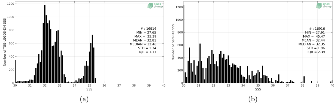
Figure 2: Histograms of SSS from TSG-LEGOS-DM (a) and SMOS L3 v2 - Daily - 0.5 Deg (CATDS-CECOS-IFREMER) (b) considering all match-up pairs per bins of 0.1 over the Arctic Ocean Pi-MEP region and for the full satellite product period.
