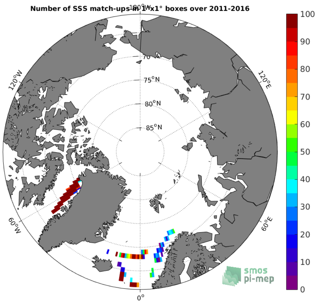
Figure 4: Number of SSS match-ups between TSG-LEGOS-DM SSS and the SMOS L3 v2 - Daily - 0.5 Deg (CATDS-CECOS-IFREMER) SSS product for the Arctic Ocean Pi-MEP region over 1°x1° boxes and for the full satellite product period.
