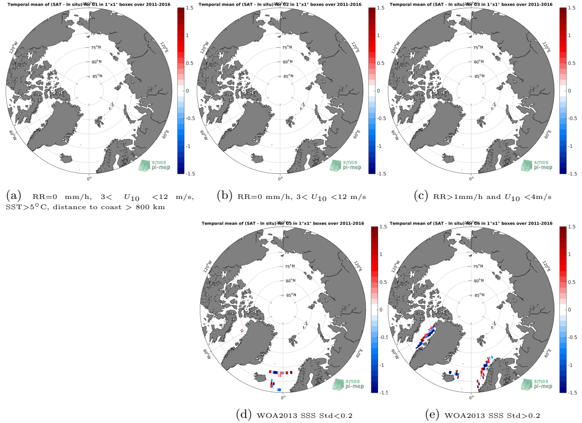
Figure 12: Temporal mean gridded over spatial boxes of size 1^{\circ}\times 1^{\circ} of \Delta\text{SSS} (SMOS L3 v2 - Daily - 0.5 Deg (CATDS-CECOS-IFREMER) - TSG-LEGOS-DM) for 5 different subdatasets corresponding to: \text{RR}=0 mm/h, 3 < U_{10} < 12 m/s, \text{SST} > 5^{\circ}\text{C} , distance to coast > 800 km (a), \text{RR}=0 mm/h, 3 < U_{10} < 12 m/s (b), \text{RR} > 1 mm/h and U_{10} < 4 m/s (c), WOA2013 SSS Std < 0.2 (d), WOA2013 SSS Std > 0.2 (e).
