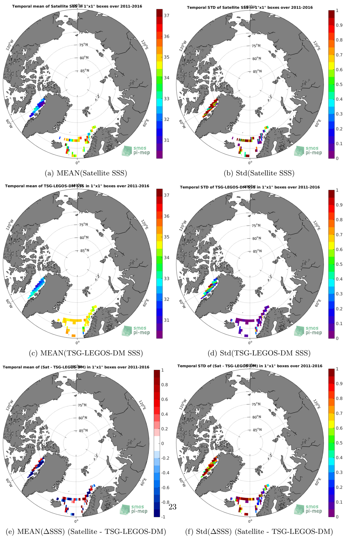
Figure 6: Temporal mean (left) and Std (right) of SSS from SMOS L3 v2 - Daily - 0.5 Deg (CATDS-CECOS-IFREMER) (top), TSG-LEGOS-DM (middle), and of \Delta SSS (Satellite - TSG-LEGOS-DM). Only match-up pairs are used to generate these maps.
