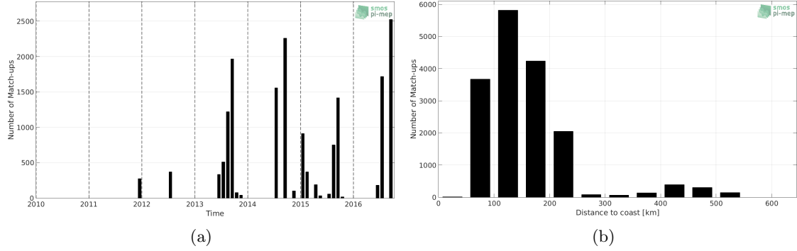
Figure 1: Number of match-ups between TSG-LEGOS-DM and SMOS L3 v2 - Daily - 0.5 Deg (CATDS-CECOS-IFREMER) SSS as a function of time (a) and as function of the distance to coast (b) over the Arctic Ocean Pi-MEP region and for the full satellite product period.
