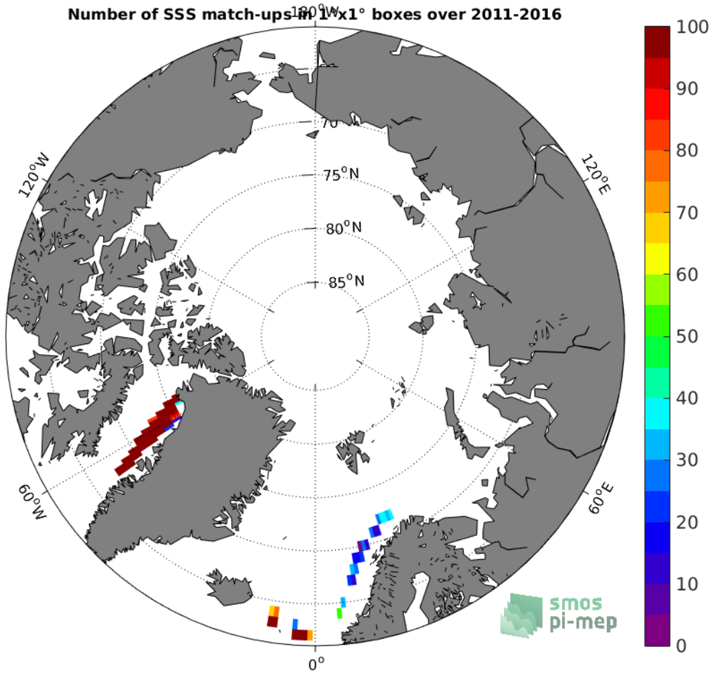
Figure 4: Number of SSS match-ups between TSG-LEGOS-DM SSS and the SMOS-L3-CATDS-CECOS-IFREMER-V2-1DAY-0.5DEG SSS product for the Arctic Ocean Pi-MEP region over 1^\circ \times 1^\circ boxes and for the full satellite product period.
