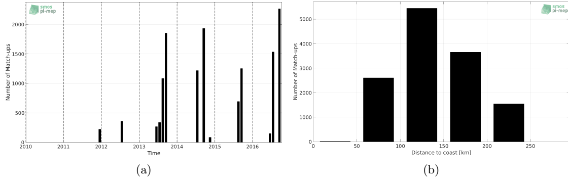
Figure 1: Number of match-ups between TSG-LEGOS-DM and SMOS-L3-CATDS-CECOS-IFREMER-V2-1DAY-0.5DEG SSS as a function of time (a) and as function of the distance to coast (b) over the Arctic Ocean Pi-MEP region and for the full satellite product period.
