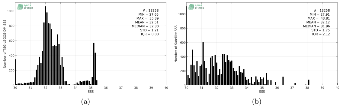
Figure 2: Histograms of SSS from TSG-LEGOS-DM (a) and SMOS-L3-CATDS-CECOS-IFREMER-V2-1DAY-0.5DEG (b) considering all match-up pairs per bins of 0.1 over the Arctic Ocean Pi-MEP region and for the full satellite product period.
