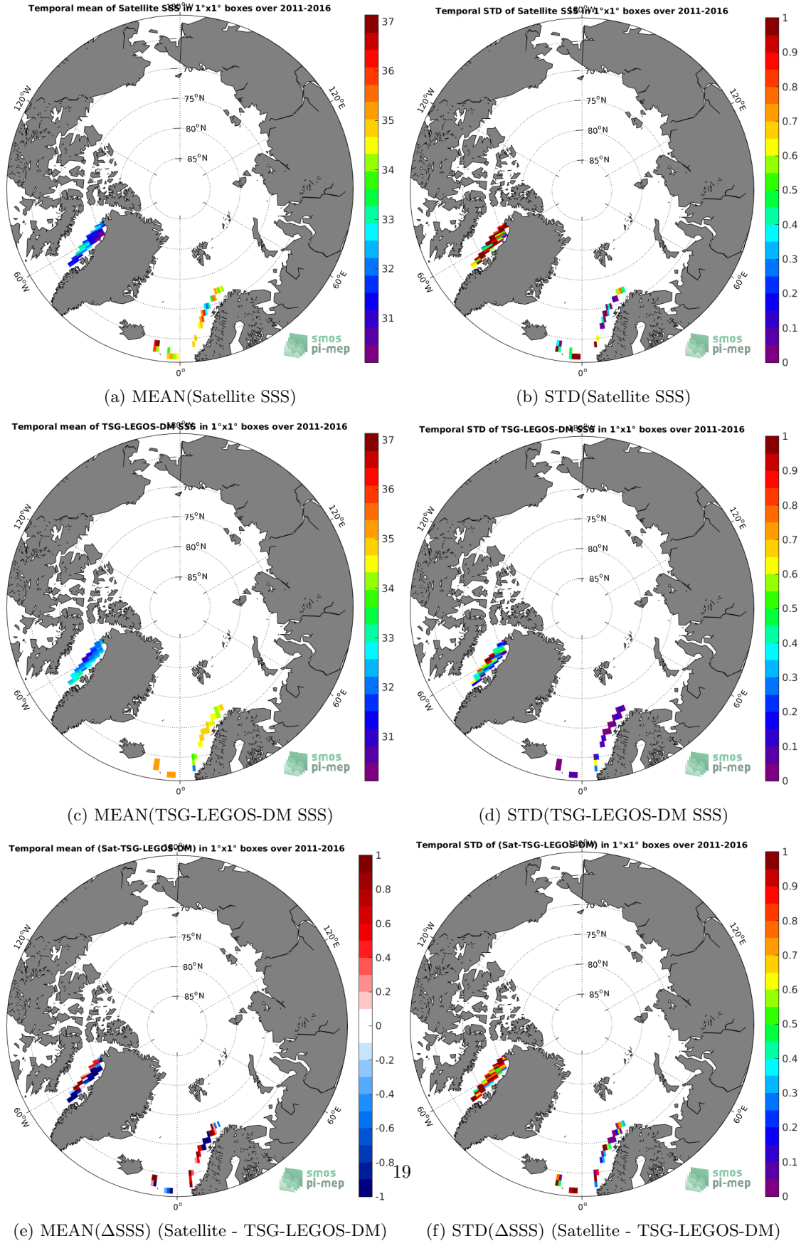
Figure 6: Temporal mean (left) and STD (right) of SSS from SMOS-L3-CATDS-CECOS-IFREMER-V2-1DAY-0.5DEG (top), TSG-LEGOS-DM (middle), and of \Delta SSS (Satellite - TSG-LEGOS-DM). Only match-up pairs are used to generate these maps.
