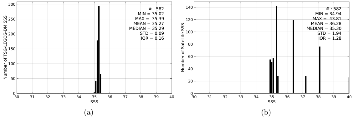
Figure 2: Histograms of SSS from TSG-LEGOS-DM (a) and SMOS-L3-CATDS-CECOS-IFREMER-V2-1DAY-0.5deg (b) considering all match-up pairs per bins of 0.1 over the Arctic Ocean Pi-MEP region and for the full satellite product period.
