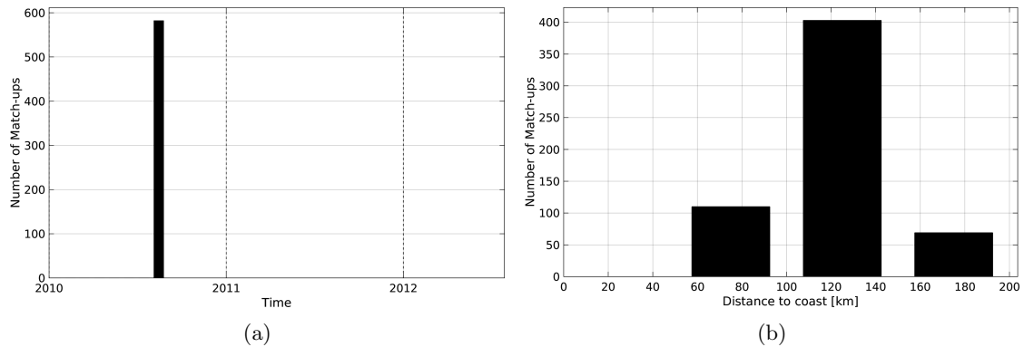
Figure 1: Number of match-ups between TSG-LEGOS-DM and SMOS-L3-CATDS-CECOS-IFREMER-V2-1DAY-0.5deg SSS as a function of time (a) and as function of the distance to coast (b) over the Arctic Ocean Pi-MEP region and for the full satellite product period.
