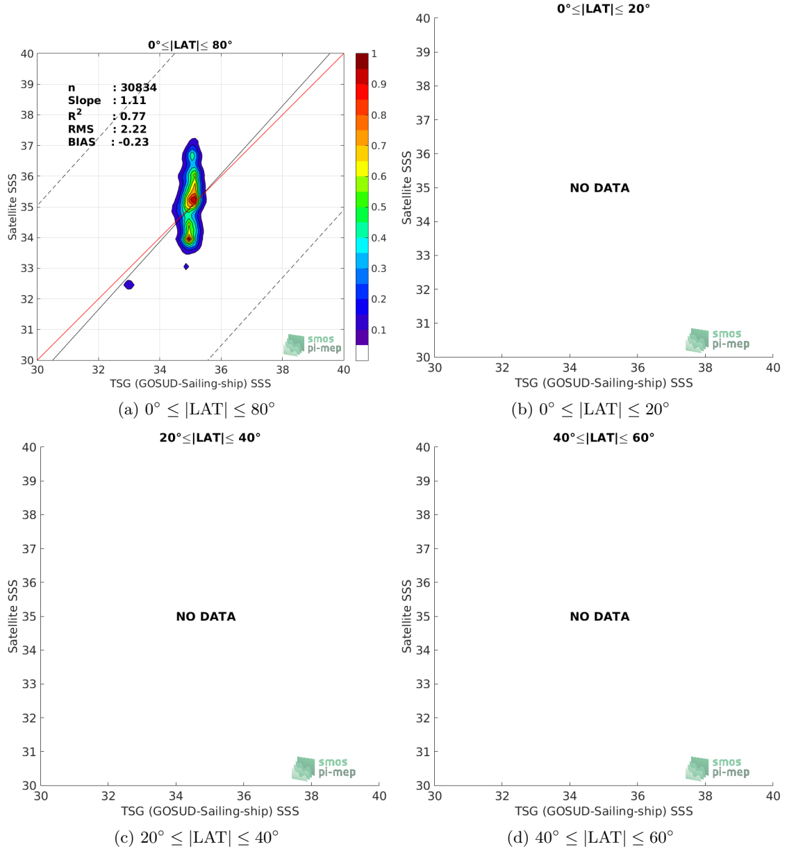
Figure 9: Contour maps of the concentration of SMOS SSS L3 v2 - Daily - 0.5 Deg (CATDS-CECOS-IFREMER) SSS (y-axis) versus TSG (GOSUD-Sailing-ship) SSS (x-axis) at match-up pairs for different latitude bands. For each plot, the red line shows x=y . The black thin and dashed lines indicate a linear fit through the data cloud and the \pm 95\% confidence levels, respectively. The number match-up pairs n , the slope and R^2 coefficient of the linear fit, the root mean square (RMS) and the mean bias between satellite and in situ data are indicated for each latitude band in each plots.
