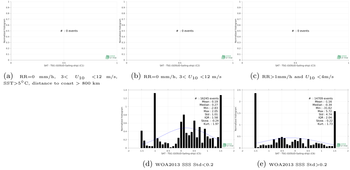
Figure 13: Normalized histogram of \Delta\text{SSS} (SMOS SSS L3 v2 - Daily - 0.5 Deg (CATDS-CECOS-IFREMER) - TSG (GOSUD-Sailing-ship)) for 5 different subdatasets corresponding to: RR=0 mm/h, 3 < U_{10} < 12 m/s, SST > 5^\circ\text{C} , distance to coast > 800 km (a), RR=0 mm/h, 3 < U_{10} < 12 m/s (b), RR > 1\text{mm/h} and U_{10} < 4\text{m/s} (c), WOA2013 SSS Std<0.2 (d), WOA2013 SSS Std>0.2 (e).
