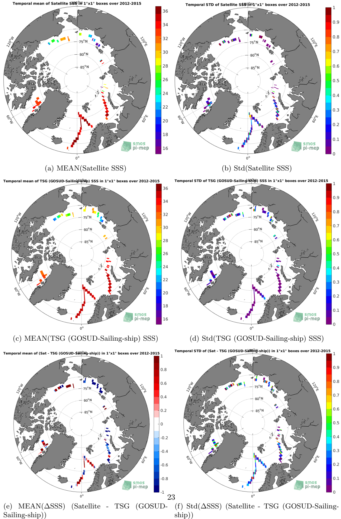
Figure 6: Temporal mean (left) and Std (right) of SSS from SMOS SSS L3 v2 - Daily - 0.5 Deg (CATDS-CECOS-IFREMER) (top), TSG (GOSUD-Sailing-ship) (middle), and of \Delta SSS (Satellite - TSG (GOSUD-Sailing-ship)). Only match-up pairs are used to generate these maps.
