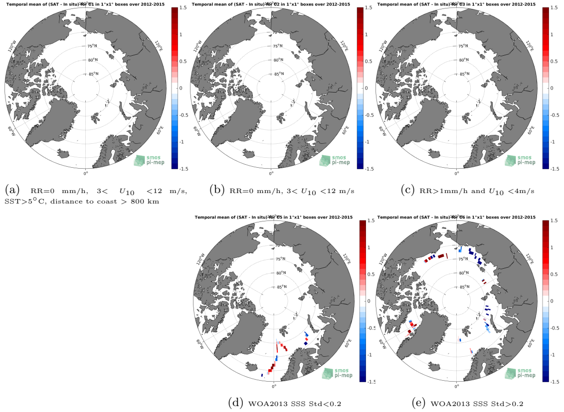
Figure 12: Temporal mean gridded over spatial boxes of size 1°x1° of \Delta SSS (SMOS SSS L3 v2 - Daily - 0.5 Deg (CATDS-CECOS-IFREMER) - TSG (GOSUD-Sailing-ship)) for 5 different subdatasets corresponding to:RR=0 mm/h, 3 < U_{10} < 12 m/s, SST>5°C, distance to coast > 800 km (a), RR=0 mm/h, 3 < U_{10} < 12 m/s (b), RR>1mm/h and U_{10} < 4 m/s (c), WOA2013 SSS Std<0.2 (d), WOA2013 SSS Std>0.2 (e).
