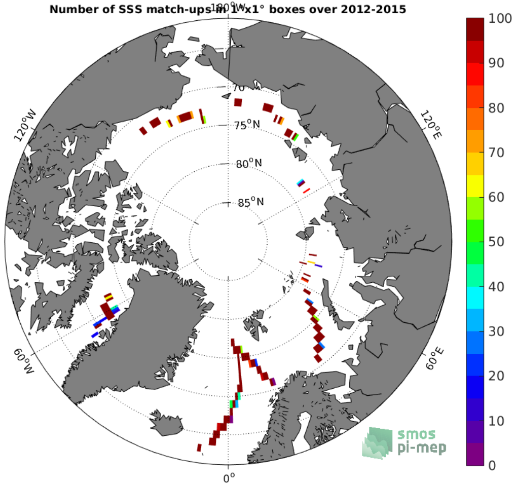
Figure 4: Number of SSS match-ups between TSG (GOSUD-Sailing-ship) SSS and the SMOS SSS L3 v2 - Daily - 0.5 Deg (CATDS-CECOS-IFREMER) SSS product for the Arctic Ocean Pi-MEP region over 1°x1° boxes and for the full satellite product period.
