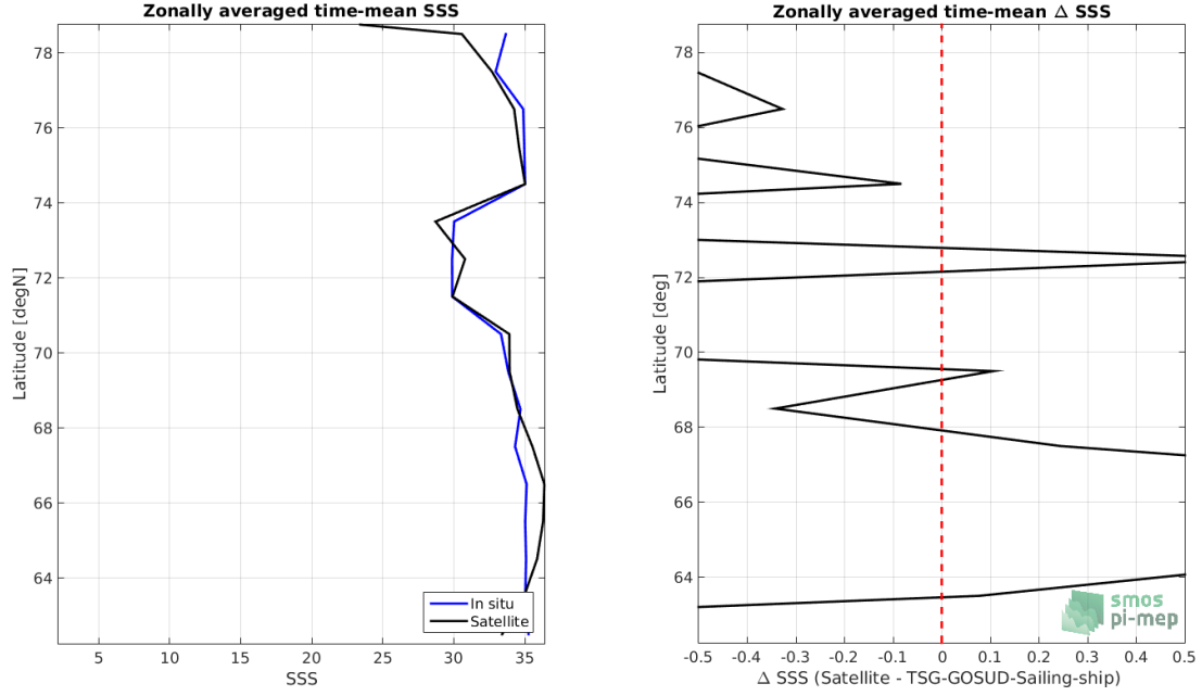
Figure 8: Left panel: Zonal mean SSS from SMOS L3 v2 - Daily - 0.5 Deg (CATDS-CECOS-IFREMER) satellite product (black) and from TSG-GOSUD-Sailing-ship (blue). Right panel: Zonal mean of \Delta SSS (Satellite - TSG-GOSUD-Sailing-ship) for all the collected Pi-MEP match-up pairs estimated over the full satellite product period.
