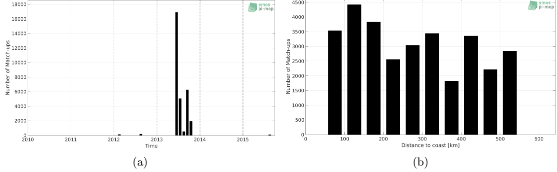
Figure 1: Number of match-ups between TSG-GOSUD-Sailing-ship and SMOS L3 v2 - Daily - 0.5 Deg (CATDS-CECOS-IFREMER) SSS as a function of time (a) and as function of the distance to coast (b) over the Arctic Ocean Pi-MEP region and for the full satellite product period.
