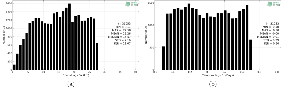
Figure 5: Histograms of the spatial (a) and temporal (b) lags between the time of the TSG-GOSUD-Sailing-ship measurements and the date of the corresponding SMOS L3 v2 - Daily - 0.5 Deg (CATDS-CECOS-IFREMER) SSS product.
