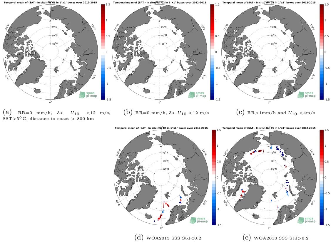
Figure 12: Temporal mean gridded over spatial boxes of size 1^\circ \times 1^\circ of \Delta SSS (SMOS L3 v2 - Daily - 0.5 Deg (CATDS-CECOS-IFREMER) - TSG-GOSUD-Sailing-ship) for 5 different subdatasets corresponding to: RR=0 mm/h, 3 < U_{10} < 12 m/s, SST>5°C, distance to coast > 800 km (a), RR=0 mm/h, 3 < U_{10} < 12 m/s (b), RR>1mm/h and U_{10} < 4 m/s (c), WOA2013 SSS Std<0.2 (d), WOA2013 SSS Std>0.2 (e).
