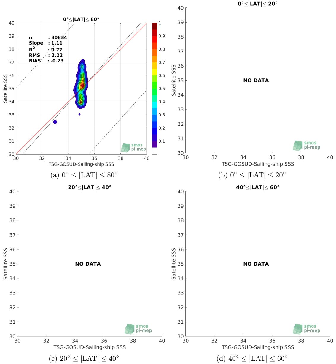
Figure 9: Contour maps of the concentration of SMOS L3 v2 - Daily - 0.5 Deg (CATDS-CECOS-IFREMER) SSS (y-axis) versus TSG-GOSUD-Sailing-ship SSS (x-axis) at match-up pairs for different latitude bands. For each plot, the red line shows x=y . The black thin and dashed lines indicate a linear fit through the data cloud and the \pm 95\% confidence levels, respectively. The number match-up pairs n , the slope and R^2 coefficient of the linear fit, the root mean square (RMS) and the mean bias between satellite and in situ data are indicated for each latitude band in each plots.
