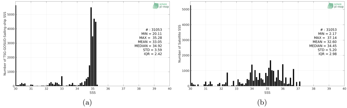
Figure 2: Histograms of SSS from TSG-GOSUD-Sailing-ship (a) and SMOS L3 v2 - Daily - 0.5 Deg (CATDS-CECOS-IFREMER) (b) considering all match-up pairs per bins of 0.1 over the Arctic Ocean Pi-MEP region and for the full satellite product period.
