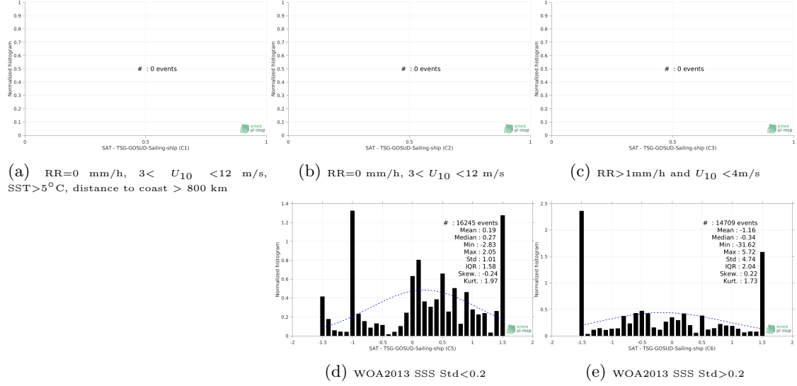
Figure 13: Normalized histogram of \Delta\text{SSS} (SMOS L3 v2 - Daily - 0.5 Deg (CATDS-CECOS-IFREMER) - TSG-GOSUD-Sailing-ship) for 5 different subdatasets corresponding to: RR=0 mm/h, 3 < U_{10} < 12 m/s, SST > 5^\circ\text{C} , distance to coast > 800 km (a), RR=0 mm/h, 3 < U_{10} < 12 m/s (b), RR > 1\text{mm/h} and U_{10} < 4\text{m/s} (c), WOA2013 SSS Std < 0.2 (d), WOA2013 SSS Std > 0.2 (e).
