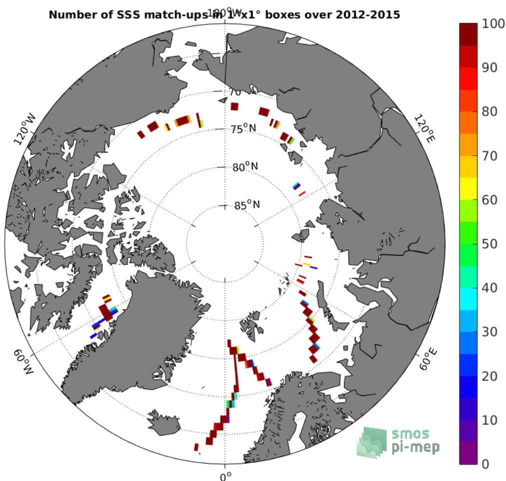
Figure 4: Number of SSS match-ups between TSG-GOSUD-Sailing-ship SSS and the SMOS L3 v2 - Daily - 0.5 Deg (CATDS-CECOS-IFREMER) SSS product for the Arctic Ocean Pi-MEP region over 1°x1° boxes and for the full satellite product period.
