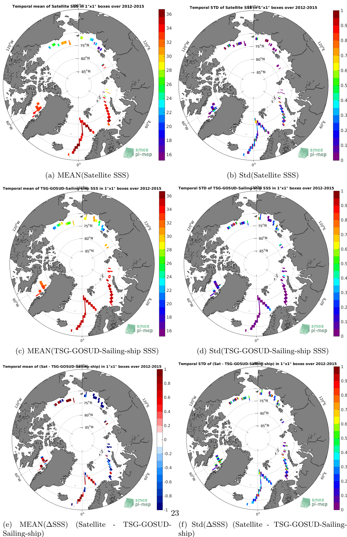
Figure 6: Temporal mean (left) and Std (right) of SSS from SMOS L3 v2 - Daily - 0.5 Deg (CATDS-CECOS-IFREMER) (top), TSG-GOSUD-Sailing-ship (middle), and of \Delta SSS (Satellite - TSG-GOSUD-Sailing-ship). Only match-up pairs are used to generate these maps.
