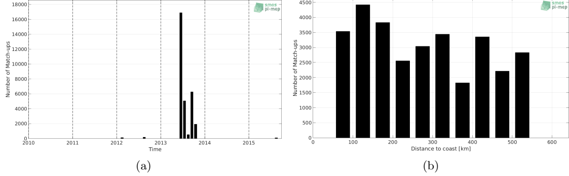
Figure 1: Number of match-ups between TSG-GOSUD-Sailing-ship and SMOS-L3-CATDS-CECOS-IFREMER-V2-1DAY-0.5DEG SSS as a function of time (a) and as function of the distance to coast (b) over the Arctic Ocean Pi-MEP region and for the full satellite product period.
