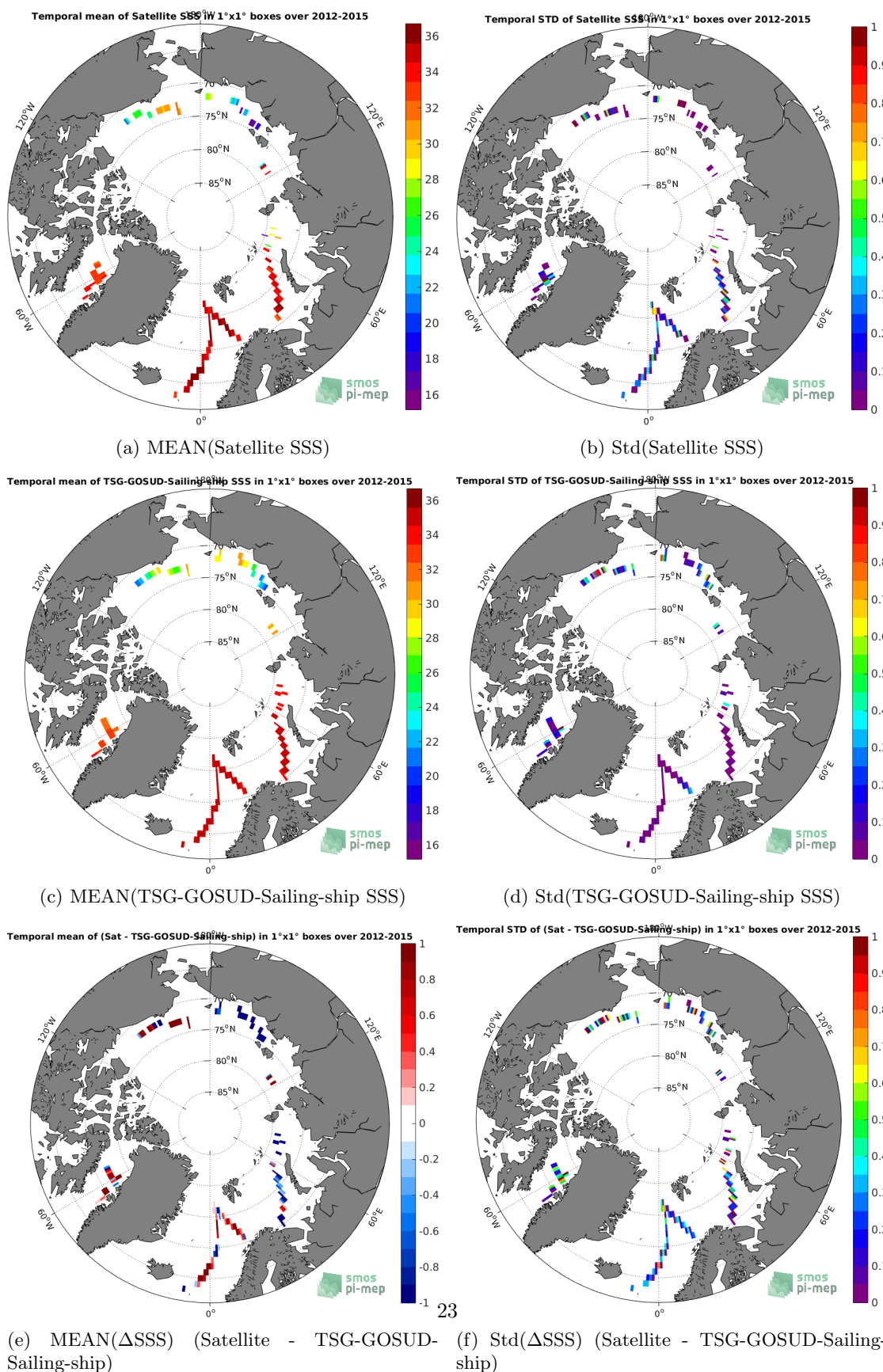
Figure 6: Temporal mean (left) and Std (right) of SSS from SMOS-L3-CATDS-CECOS-IFREMER-V2-1DAY-0.5DEG (top), TSG-GOSUD-Sailing-ship (middle), and of \Delta SSS (Satellite - TSG-GOSUD-Sailing-ship). Only match-up pairs are used to generate these maps.
