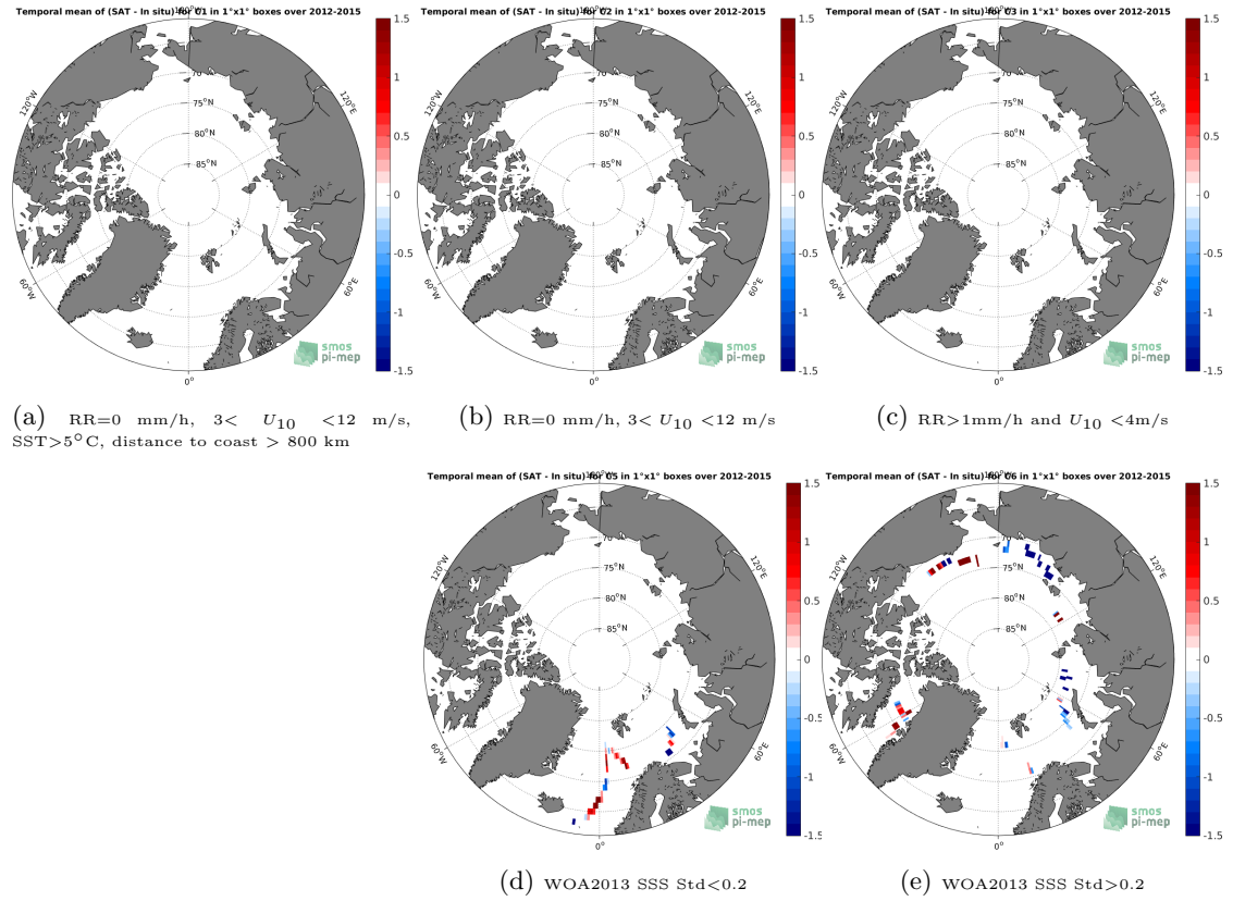
Figure 12: Temporal mean gridded over spatial boxes of size 1^\circ \times 1^\circ of \Delta SSS (SMOS-L3-CATDS-CECOS-IFREMER-V2-1DAY-0.5DEG - TSG-GOSUD-Sailing-ship) for 5 different subdatasets corresponding to: RR=0 mm/h, 3 < U_{10} < 12 m/s, SST > 5^\circ C , distance to coast > 800 km (a), RR=0 mm/h, 3 < U_{10} < 12 m/s (b), RR > 1 mm/h and U_{10} < 4 m/s (c), WOA2013 SSS Std < 0.2 (d), WOA2013 SSS Std > 0.2 (e).
