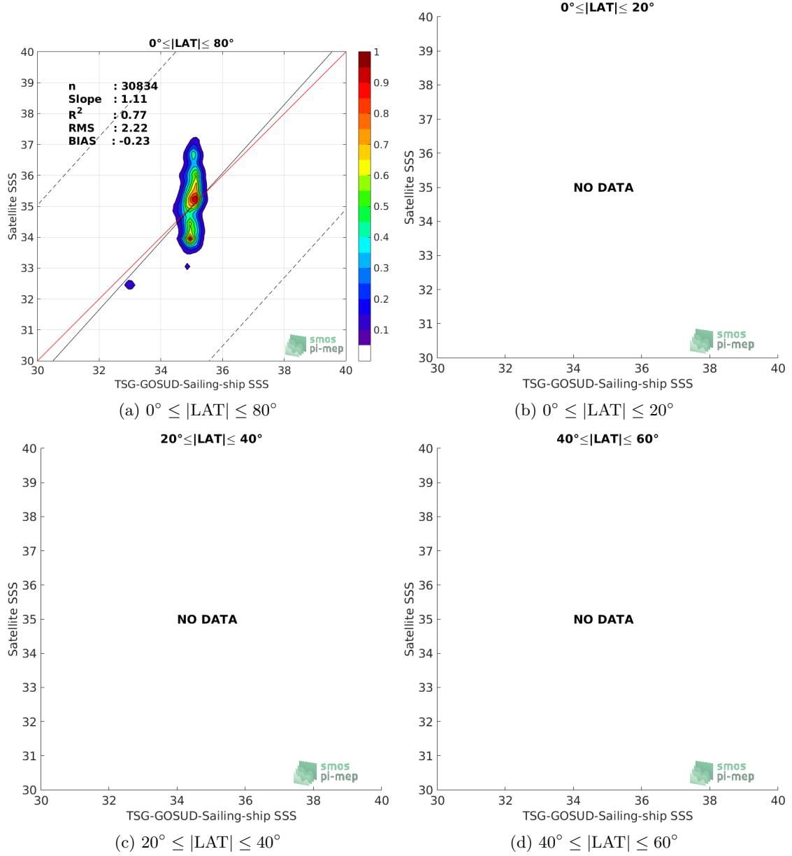
Figure 9: Contour maps of the concentration of SMOS-L3-CATDS-CECOS-IFREMER-V2-1DAY-0.5DEG SSS (y-axis) versus TSG-GOSUD-Sailing-ship SSS (x-axis) at match-up pairs for different latitude bands. For each plot, the red line shows x=y . The black thin and dashed lines indicate a linear fit through the data cloud and the \pm 95\% confidence levels, respectively. The number match-up pairs n , the slope and R^2 coefficient of the linear fit, the root mean square (RMS) and the mean bias between satellite and in situ data are indicated for each latitude band in each plots.
