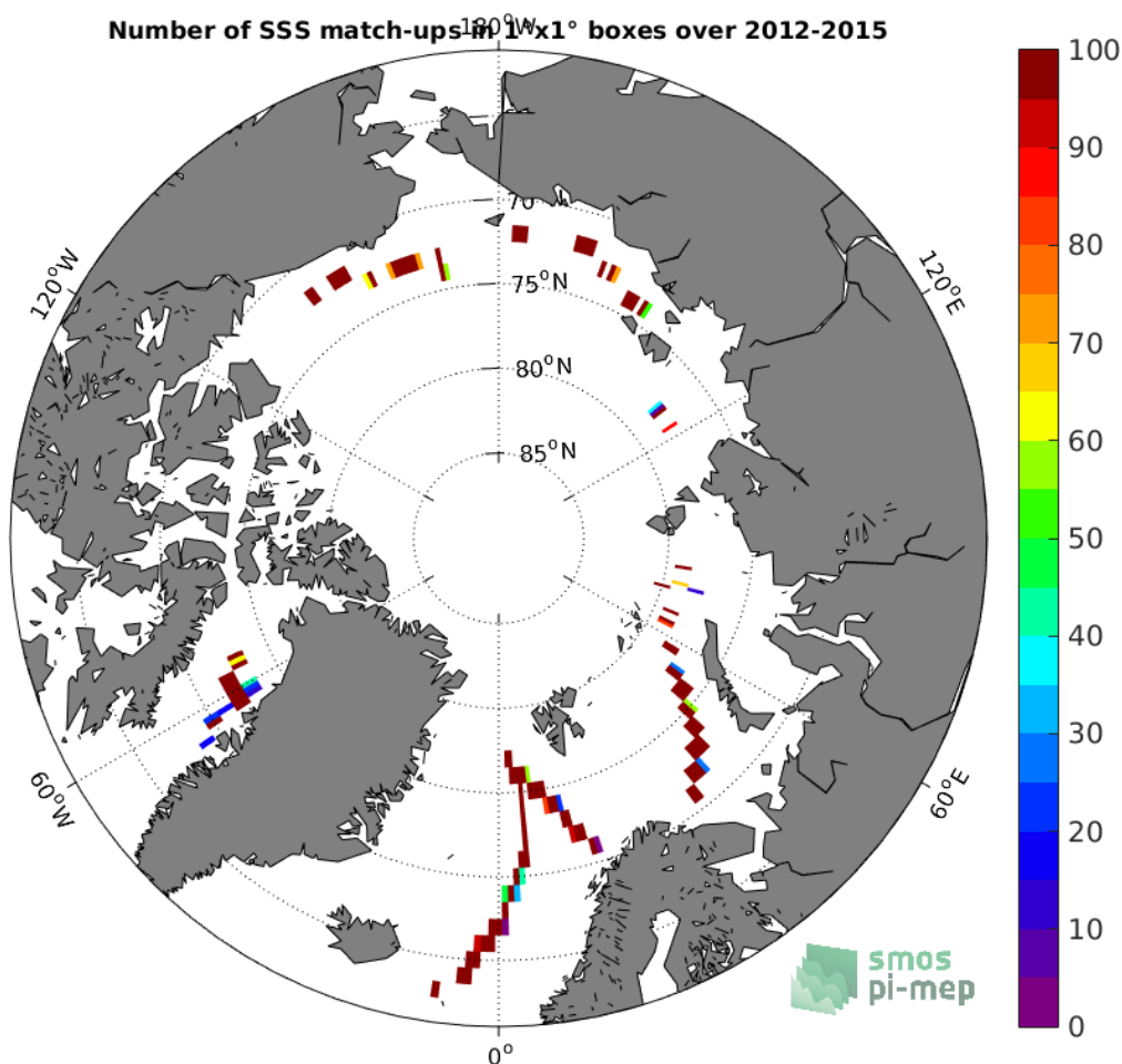
Figure 4: Number of SSS match-ups between TSG-GOSUD-Sailing-ship SSS and the SMOS-L3-CATDS-CECOS-IFREMER-V2-1DAY-0.5DEG SSS product for the Arctic Ocean Pi-MEP region over 1°x1° boxes and for the full satellite product period.
