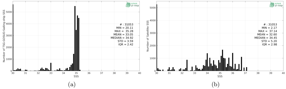
Figure 2: Histograms of SSS from TSG-GOSUD-Sailing-ship (a) and SMOS-L3-CATDS-CECOS-IFREMER-V2-1DAY-0.5DEG (b) considering all match-up pairs per bins of 0.1 over the Arctic Ocean Pi-MEP region and for the full satellite product period.
