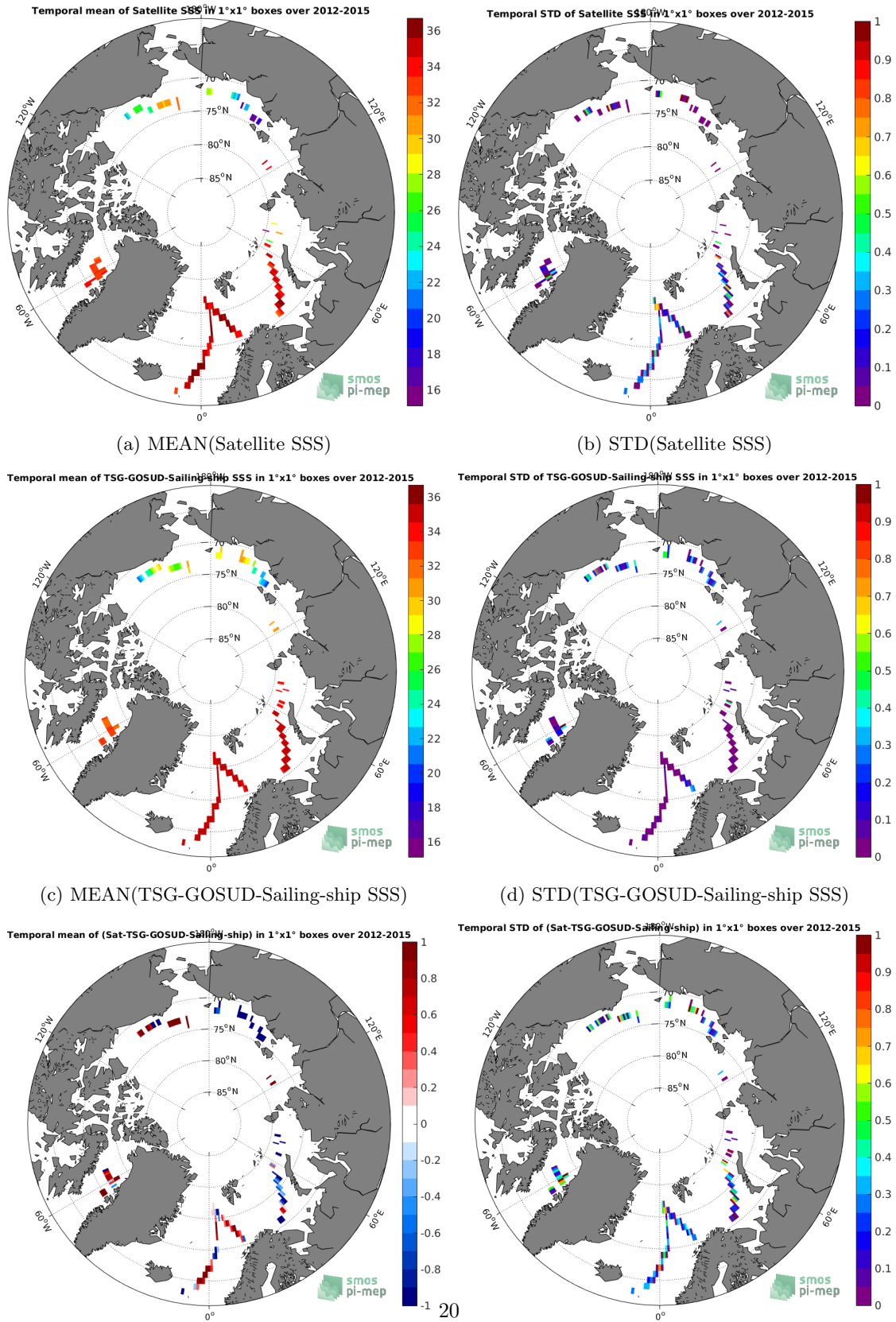
Figure 6: Temporal mean (left) and STD (right) of SSS from SMOS-L3-CATDS-CECOS-IFREMER-V2-1DAY-0.5DEG (top), TSG-GOSUD-Sailing-ship (middle), and of \Delta SSS (Satellite - TSG-GOSUD-Sailing-ship). Only match-up pairs are used to generate these maps.
