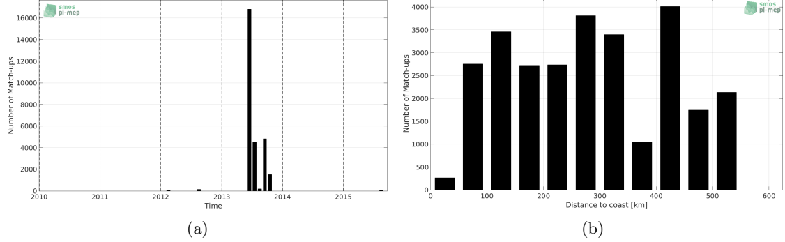
Figure 1: Number of match-ups between TSG-GOSUD-Sailing-ship and SMOS-L3-CATDS-CECOS-IFREMER-V2-1DAY-0.5DEG SSS as a function of time (a) and as function of the distance to coast (b) over the Arctic Ocean Pi-MEP region and for the full satellite product period.
