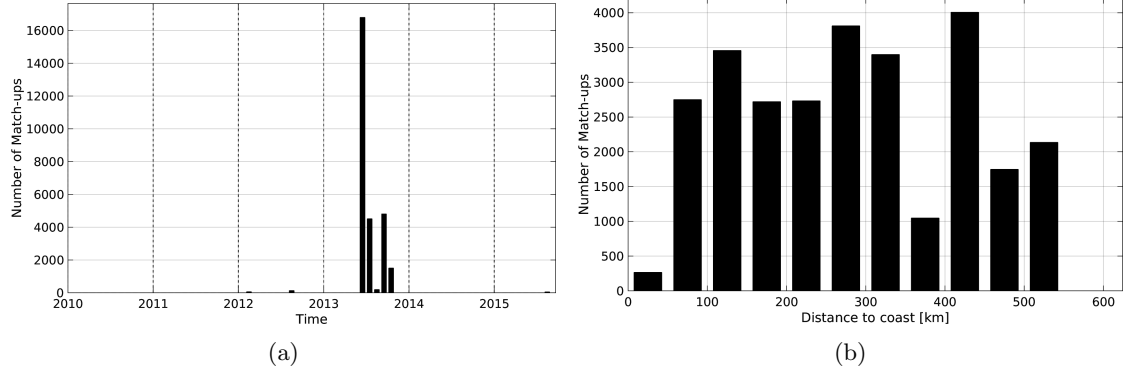
Figure 1: Number of match-ups between TSG-GOSUD-Sailing-ship and SMOS-L3-CATDS-CECOS-IFREMER-V2-1DAY-0.5DEG SSS as a function of time (a) and as function of the distance to coast (b) over the Arctic Ocean Pi-MEP region and for the full satellite product period.
