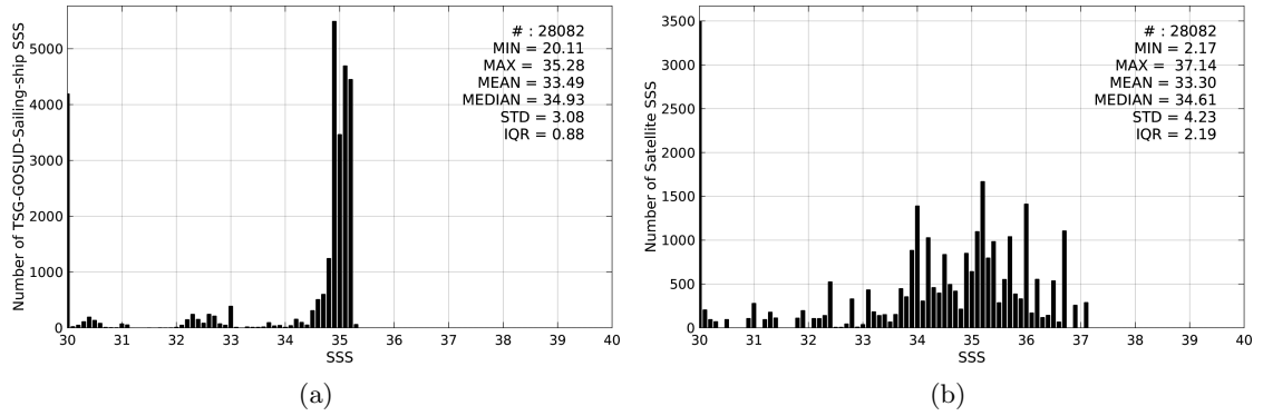
Figure 2: Histograms of SSS from TSG-GOSUD-Sailing-ship (a) and SMOS-L3-CATDS-CECOS-IFREMER-V2-1DAY-0.5DEG (b) considering all match-up pairs per bins of 0.1 over the Arctic Ocean Pi-MEP region and for the full satellite product period.
