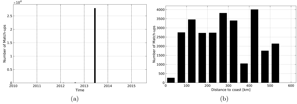
Figure 1: Number of match-ups between TSG-GOSUD-Sailing-ship and SMOS-L3-CATDS-CECOS-IFREMER-V2-1DAY-0.5deg SSS as a function of time (a) and as function of the distance to coast (b) over the Arctic Ocean Pi-MEP region and for the full satellite product period.
