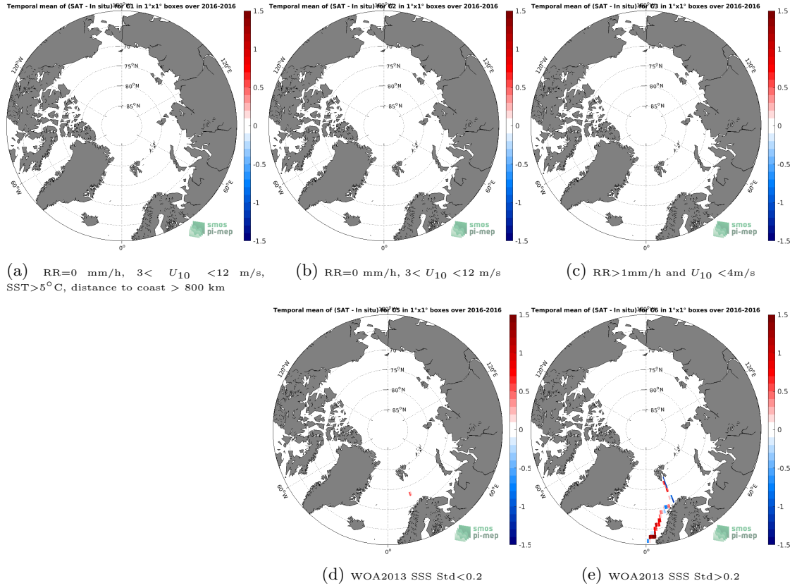
Figure 12: Temporal mean gridded over spatial boxes of size 1°x1° of \Delta SSS (SMOS SSS L3 v2 - Daily - 0.5 Deg (CATDS-CECOS-IFREMER) - TSG (GOSUD-Research-vessel)) for 5 different subdatasets corresponding to: RR=0 mm/h, 3 < U_{10} < 12 m/s, SST>5°C, distance to coast > 800 km (a), RR=0 mm/h, 3 < U_{10} < 12 m/s (b), RR>1mm/h and U_{10} < 4 m/s (c), WOA2013 SSS Std<0.2 (d), WOA2013 SSS Std>0.2 (e).
