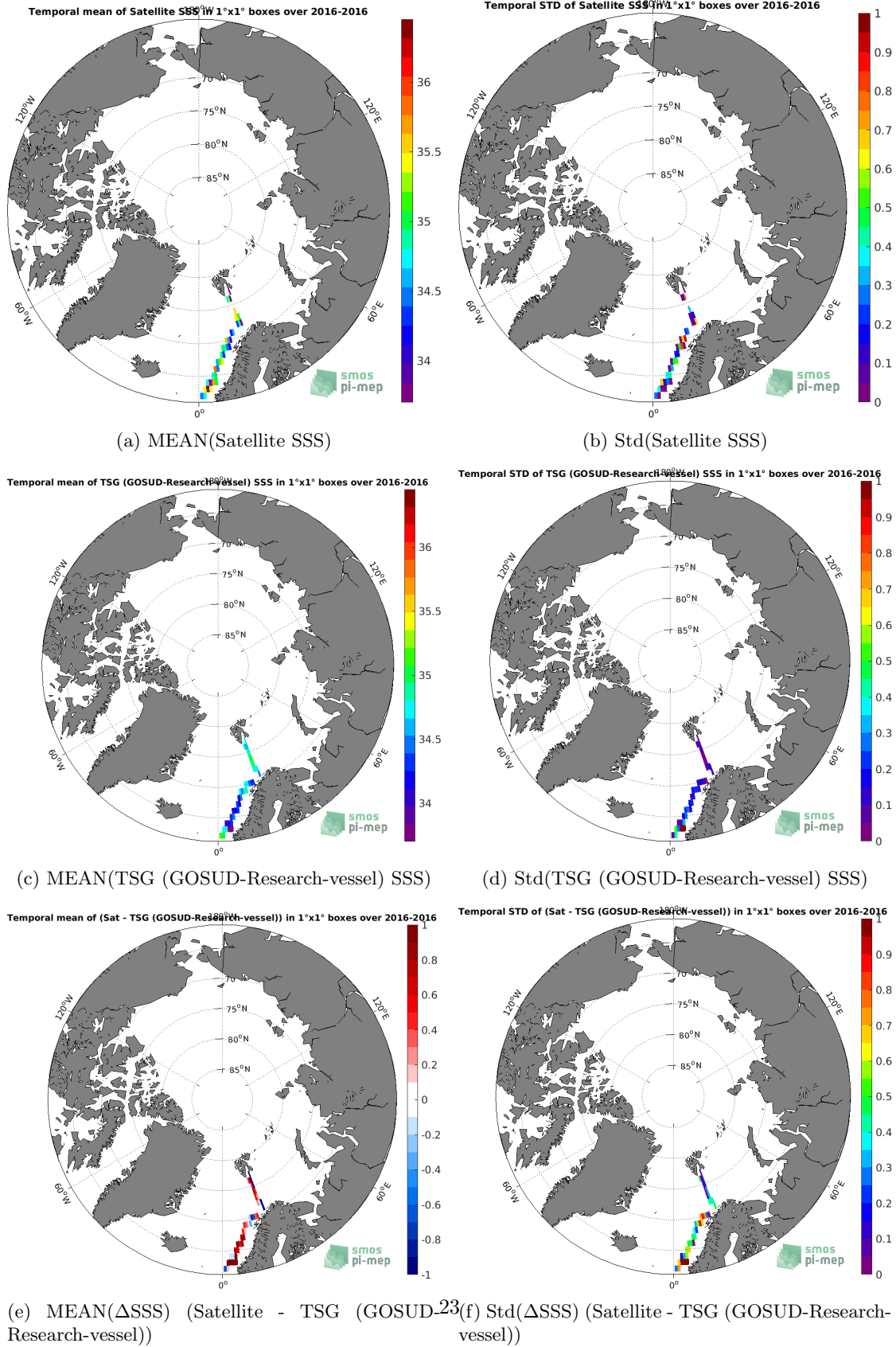
Figure 6: Temporal mean (left) and Std (right) of SSS from SMOS SSS L3 v2 - Daily - 0.5 Deg (CATDS-CECOS-IFREMER) (top), TSG (GOSUD-Research-vessel) (middle), and of \Delta SSS (Satellite - TSG (GOSUD-Research-vessel)). Only match-up pairs are used to generate these maps.
