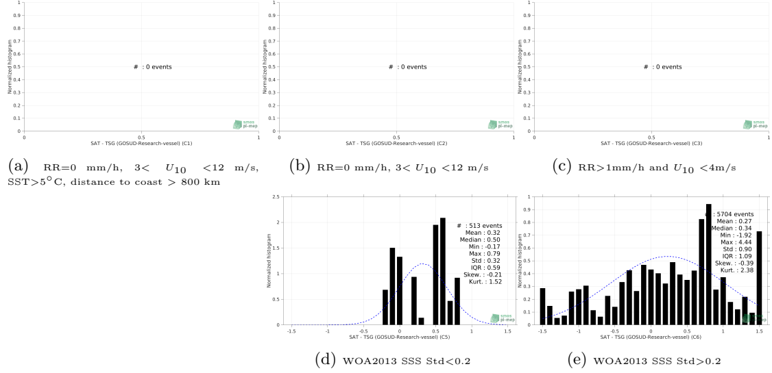
Figure 13: Normalized histogram of \Delta\text{SSS} (SMOS SSS L3 v2 - Daily - 0.5 Deg (CATDS-CECOS-IFREMER) - TSG (GOSUD-Research-vessel)) for 5 different subdatasets corresponding to: RR=0 mm/h, 3 < U_{10} < 12 m/s, SST > 5^{\circ}\text{C} , distance to coast > 800 km (a), RR=0 mm/h, 3 < U_{10} < 12 m/s (b), RR > 1\text{mm/h} and U_{10} < 4\text{m/s} (c), WOA2013 SSS Std < 0.2 (d), WOA2013 SSS Std > 0.2 (e).
