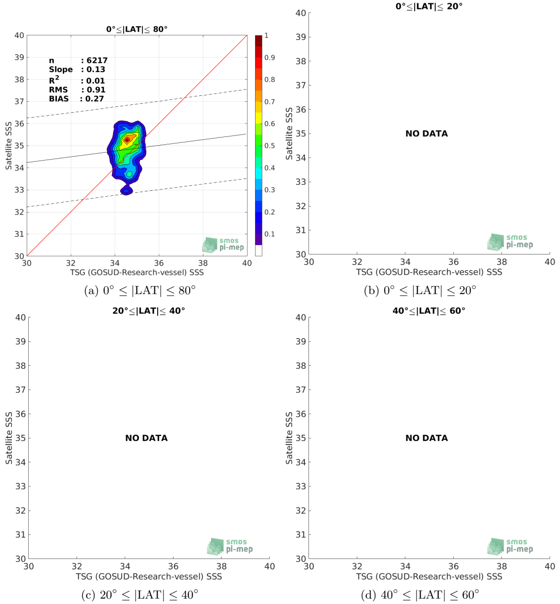
Figure 9: Contour maps of the concentration of SMOS SSS L3 v2 - Daily - 0.5 Deg (CATDS-CECOS-IFREMER) SSS (y-axis) versus TSG (GOSUD-Research-vessel) SSS (x-axis) at match-up pairs for different latitude bands. For each plot, the red line shows x=y . The black thin and dashed lines indicate a linear fit through the data cloud and the \pm 95\% confidence levels, respectively. The number match-up pairs n , the slope and R^2 coefficient of the linear fit, the root mean square (RMS) and the mean bias between satellite and in situ data are indicated for each latitude band in each plots.
