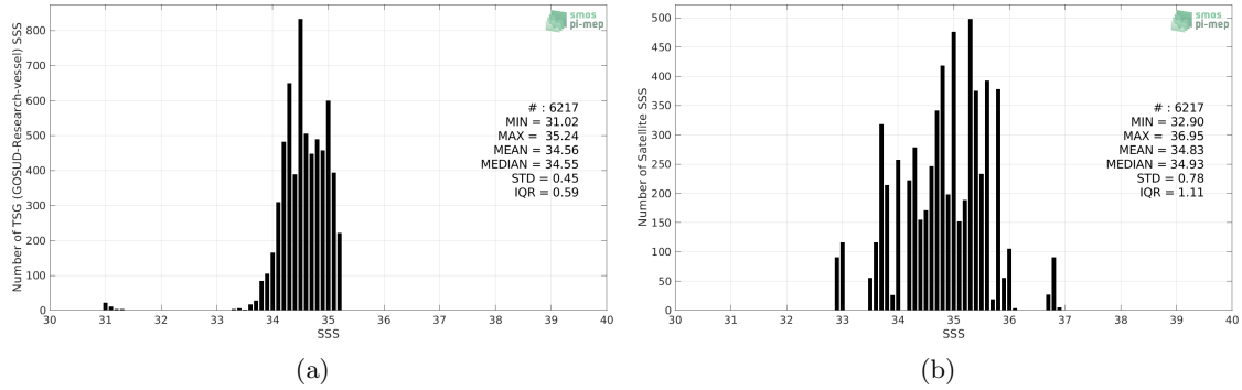
Figure 2: Histograms of SSS from TSG (GOSUD-Research-vessel) (a) and SMOS SSS L3 v2 - Daily - 0.5 Deg (CATDS-CECOS-IFREMER) (b) considering all match-up pairs per bins of 0.1 over the Arctic Ocean Pi-MEP region and for the full satellite product period.
