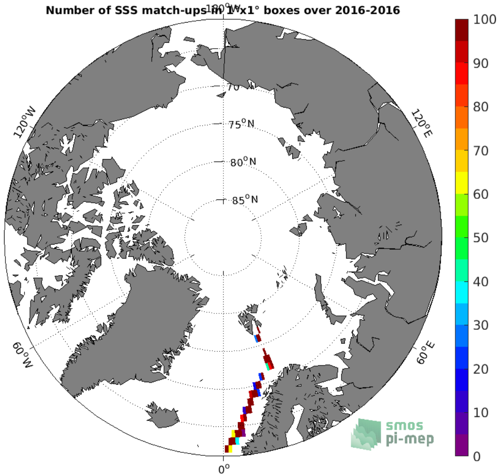
Figure 4: Number of SSS match-ups between TSG (GOSUD-Research-vessel) SSS and the SMOS SSS L3 v2 - Daily - 0.5 Deg (CATDS-CECOS-IFREMER) SSS product for the Arctic Ocean Pi-MEP region over 1^\circ \times 1^\circ boxes and for the full satellite product period.
