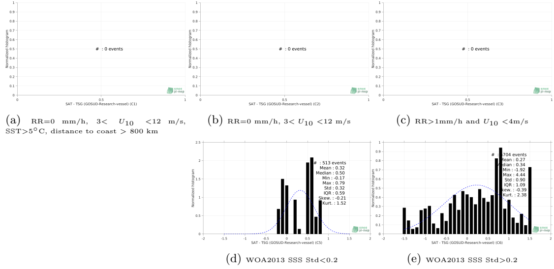
Figure 13: Normalized histogram of \Delta\text{SSS} (SMOS SSS L3 v2 - Daily - 0.5 Deg (CATDS-CECOS-IFREMER) - TSG (GOSUD-Research-vessel)) for 5 different subdatasets corresponding to: RR=0 mm/h, 3 < U_{10} < 12 m/s, SST > 5^\circ\text{C} , distance to coast > 800 km (a), RR=0 mm/h, 3 < U_{10} < 12 m/s (b), RR > 1\text{mm/h} and U_{10} < 4\text{m/s} (c), WOA2013 SSS Std<0.2 (d), WOA2013 SSS Std>0.2 (e).
