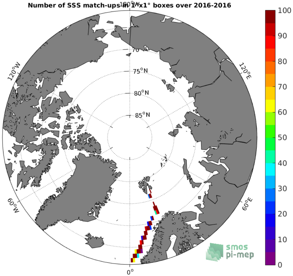
Figure 4: Number of SSS match-ups between TSG (GOSUD-Research-vessel) SSS and the SMOS SSS L3 v2 - Daily - 0.5 Deg (CATDS-CECOS-IFREMER) SSS product for the Arctic Ocean Pi-MEP region over 1°x1° boxes and for the full satellite product period.
