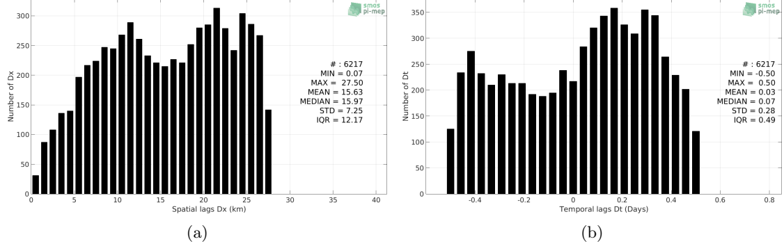
Figure 5: Histograms of the spatial (a) and temporal (b) lags between the time of the TSG (GOSUD-Research-vessel) measurements and the date of the corresponding SMOS SSS L3 v2 - Daily - 0.5 Deg (CATDS-CECOS-IFREMER) SSS product.
