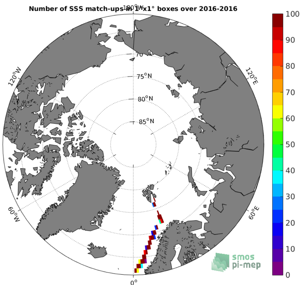
Figure 4: Number of SSS match-ups between TSG-GOSUD-Research-vessel SSS and the SMOS L3 v2 - Daily - 0.5 Deg (CATDS-CECOS-IFREMER) SSS product for the Arctic Ocean Pi-MEP region over 1°x1° boxes and for the full satellite product period.
