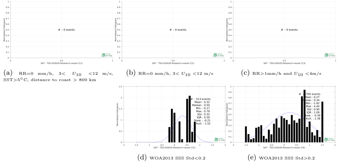
Figure 13: Normalized histogram of \Delta\text{SSS} (SMOS L3 v2 - Daily - 0.5 Deg (CATDS-CECOS-IFREMER) - TSG-GOSUD-Research-vessel) for 5 different subdatasets corresponding to: RR=0 mm/h, 3 < U_{10} < 12 m/s, SST >5^{\circ}\text{C} , distance to coast > 800 km (a), RR=0 mm/h, 3 < U_{10} < 12 m/s (b), RR>1\text{mm/h} and U_{10} < 4\text{m/s} (c), WOA2013 SSS Std <0.2 (d), WOA2013 SSS Std >0.2 (e).
