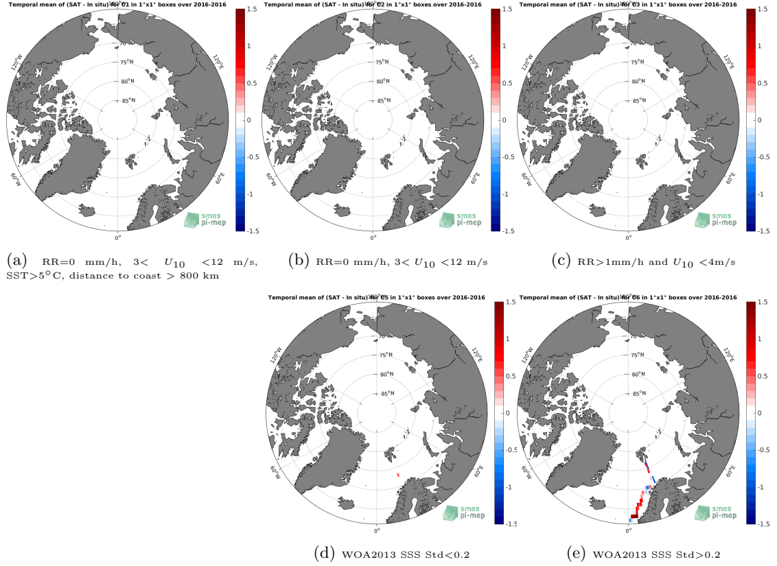
Figure 12: Temporal mean gridded over spatial boxes of size 1^\circ \times 1^\circ of \Delta SSS (SMOS L3 v2 - Daily - 0.5 Deg (CATDS-CECOS-IFREMER) - TSG-GOSUD-Research-vessel) for 5 different subdatasets corresponding to: RR=0 mm/h, 3 < U_{10} < 12 m/s, SST > 5^\circ\text{C} , distance to coast > 800 km (a), RR=0 mm/h, 3 < U_{10} < 12 m/s (b), RR > 1 mm/h and U_{10} < 4 m/s (c), WOA2013 SSS Std < 0.2 (d), WOA2013 SSS Std > 0.2 (e).
