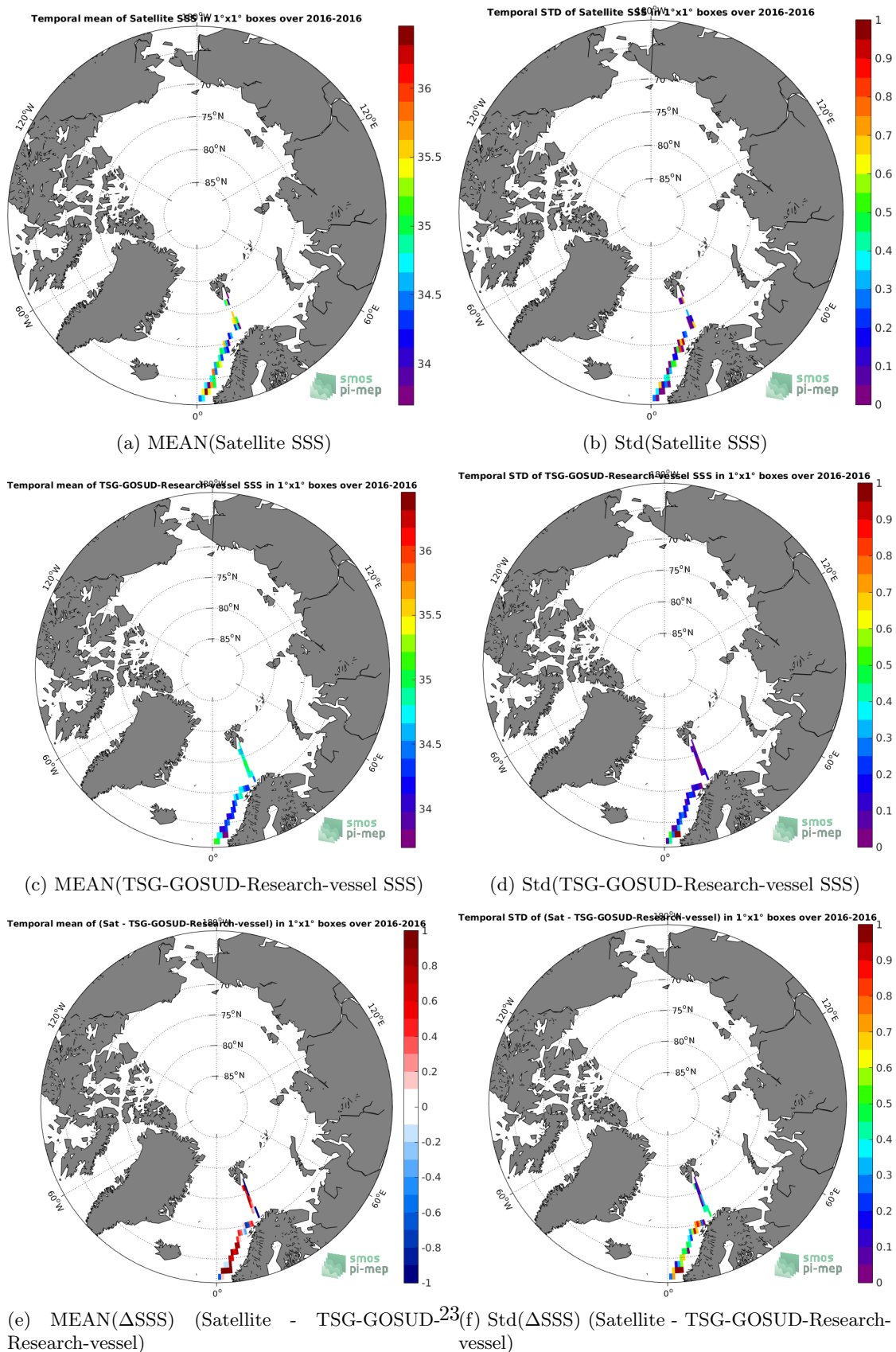
Figure 6: Temporal mean (left) and Std (right) of SSS from SMOS L3 v2 - Daily - 0.5 Deg (CATDS-CECOS-IFREMER) (top), TSG-GOSUD-Research-vessel (middle), and of \Delta SSS (Satellite - TSG-GOSUD-Research-vessel). Only match-up pairs are used to generate these maps.
