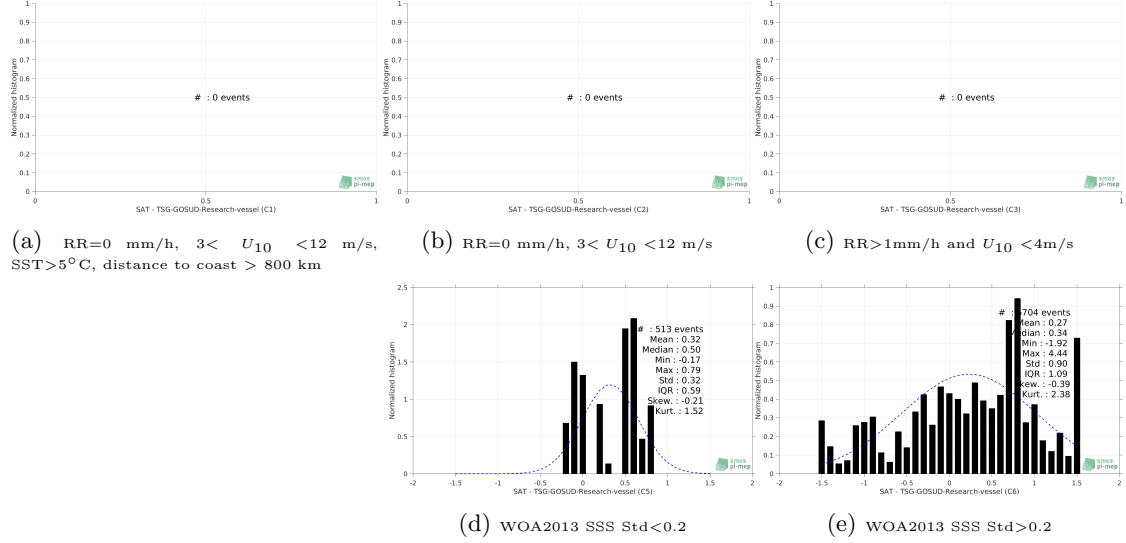
Figure 13: Normalized histogram of \Delta\text{SSS} (SMOS-L3-CATDS-CECOS-IFREMER-V2-1DAY-0.5DEG - TSG-GOSUD-Research-vessel) for 5 different subdatasets corresponding to: RR=0 mm/h, 3 < U_{10} < 12 m/s, SST > 5^{\circ}\text{C} , distance to coast > 800 km (a), RR=0 mm/h, 3 < U_{10} < 12 m/s (b), RR > 1\text{mm/h} and U_{10} < 4\text{m/s} (c), WOA2013 SSS Std < 0.2 (d), WOA2013 SSS Std > 0.2 (e).
