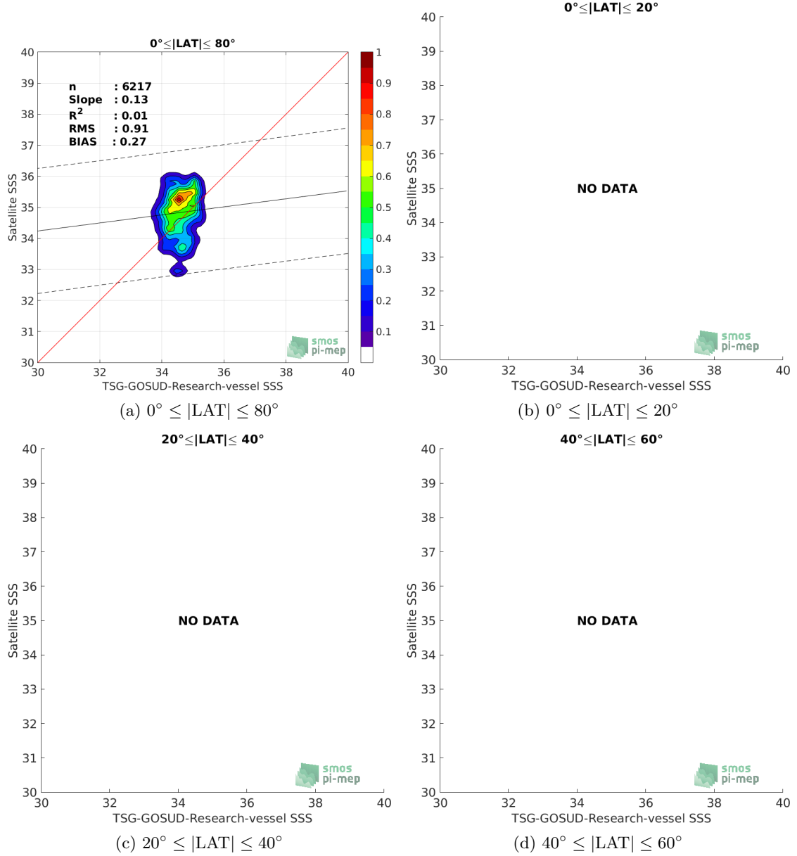
Figure 9: Contour maps of the concentration of SMOS-L3-CATDS-CECOS-IFREMER-V2-1DAY-0.5DEG SSS (y-axis) versus TSG-GOSUD-Research-vessel SSS (x-axis) at match-up pairs for different latitude bands. For each plot, the red line shows x=y . The black thin and dashed lines indicate a linear fit through the data cloud and the \pm 95\% confidence levels, respectively. The number match-up pairs n , the slope and R^2 coefficient of the linear fit, the root mean square (RMS) and the mean bias between satellite and in situ data are indicated for each latitude band in each plots.
