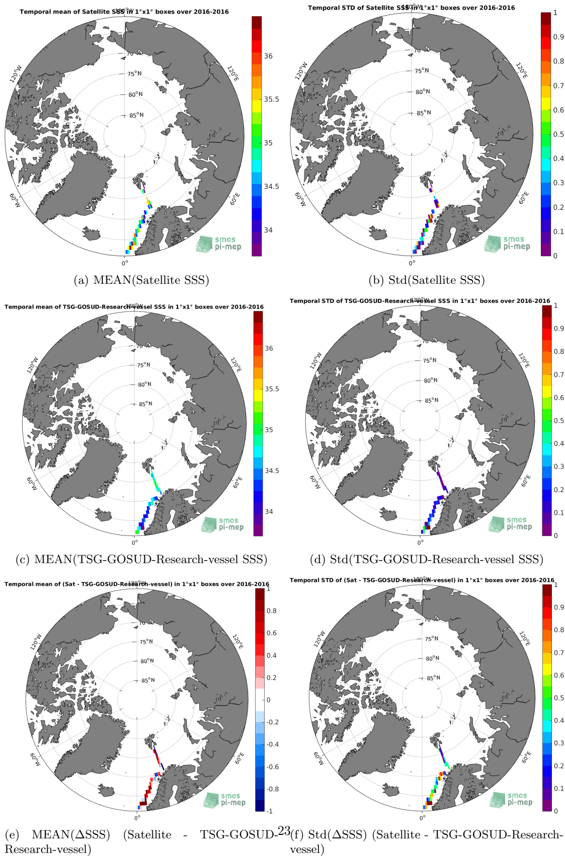
Figure 6: Temporal mean (left) and Std (right) of SSS from SMOS-L3-CATDS-CECOS-IFREMER-V2-1DAY-0.5DEG (top), TSG-GOSUD-Research-vessel (middle), and of \Delta SSS (Satellite - TSG-GOSUD-Research-vessel). Only match-up pairs are used to generate these maps.
