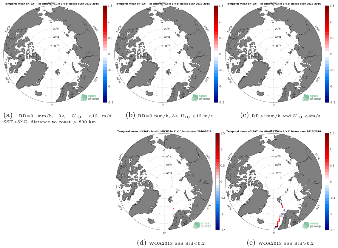
Figure 12: Temporal mean gridded over spatial boxes of size 1^\circ \times 1^\circ of \Delta SSS (SMOS-L3-CATDS-CECOS-IFREMER-V2-1DAY-0.5DEG - TSG-GOSUD-Research-vessel) for 5 different subdatasets corresponding to: RR=0 mm/h, 3 < U_{10} < 12 m/s, SST >5^\circ\text{C} , distance to coast > 800 km (a), RR=0 mm/h, 3 < U_{10} < 12 m/s (b), RR >1 mm/h and U_{10} < 4 m/s (c), WOA2013 SSS Std <0.2 (d), WOA2013 SSS Std >0.2 (e).
