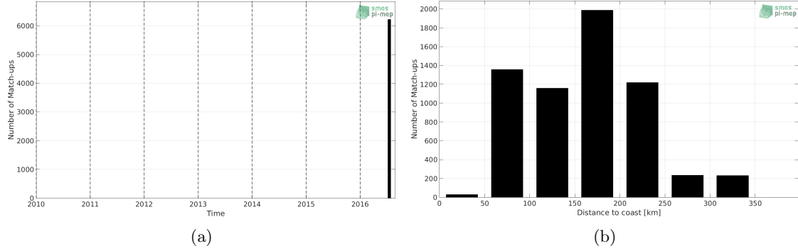
Figure 1: Number of match-ups between TSG-GOSUD-Research-vessel and SMOS-L3-CATDS-CECOS-IFREMER-V2-1DAY-0.5DEG SSS as a function of time (a) and as function of the distance to coast (b) over the Arctic Ocean Pi-MEP region and for the full satellite product period.
