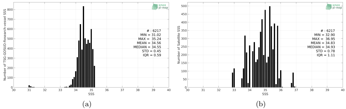
Figure 2: Histograms of SSS from TSG-GOSUD-Research-vessel (a) and SMOS-L3-CATDS-CECOS-IFREMER-V2-1DAY-0.5DEG (b) considering all match-up pairs per bins of 0.1 over the Arctic Ocean Pi-MEP region and for the full satellite product period.
