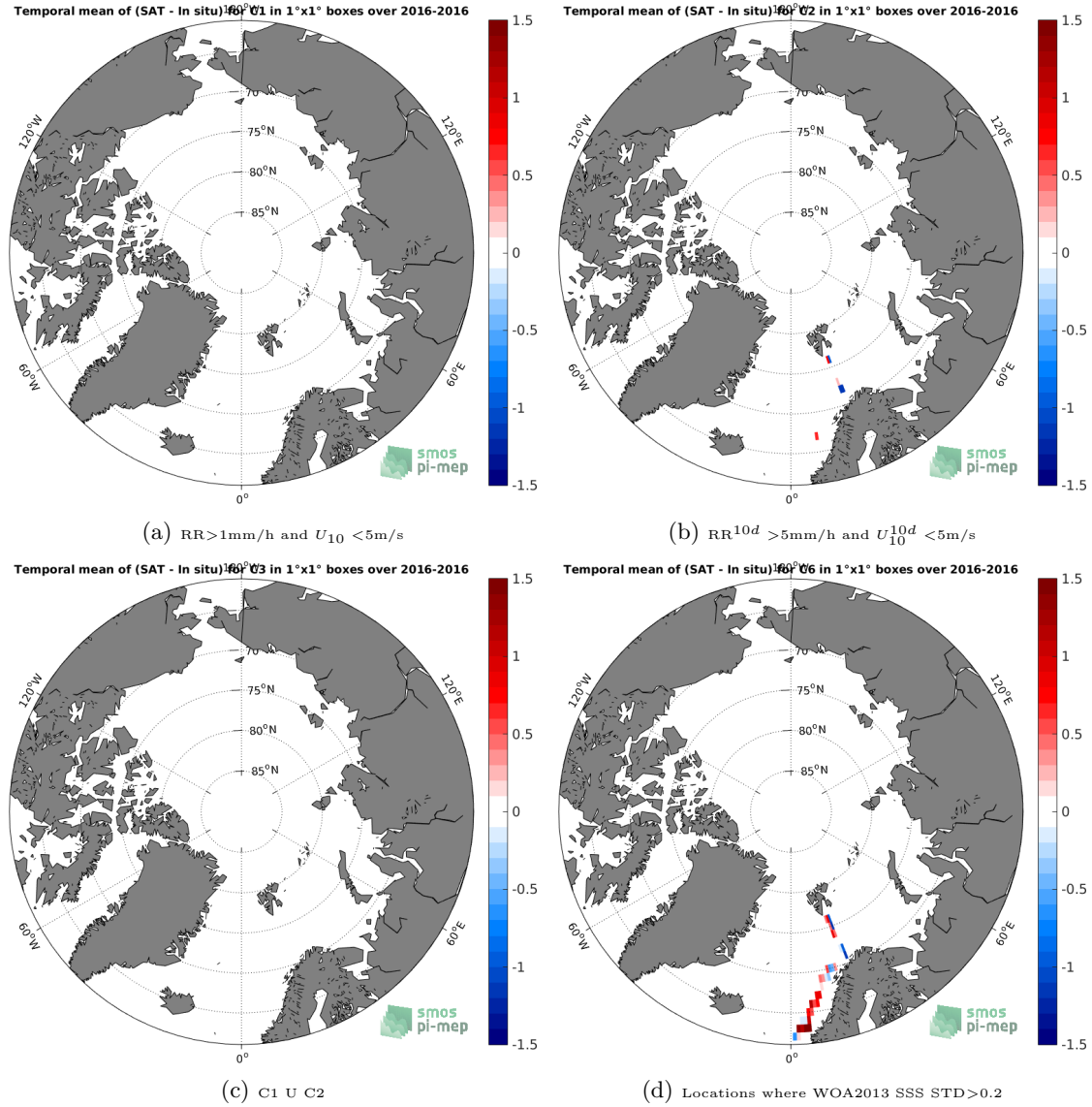
Figure 12: Temporal mean gridded over spatial boxes of size 1^\circ \times 1^\circ of \Delta SSS (SMOS-L3-CATDS-CECOS-IFREMER-V2-1DAY-0.5DEG - TSG-GOSUD-Research-vessel) for 4 different subdatasets corresponding to: RR > 1\text{mm/h} and U_{10} < 5\text{m/s} (a), RR^{10d} > 5\text{mm/h} and U_{10}^{10d} < 5\text{m/s} (b), C1 U C2 (c), Locations where WOA2013 SSS STD > 0.2 (d).
