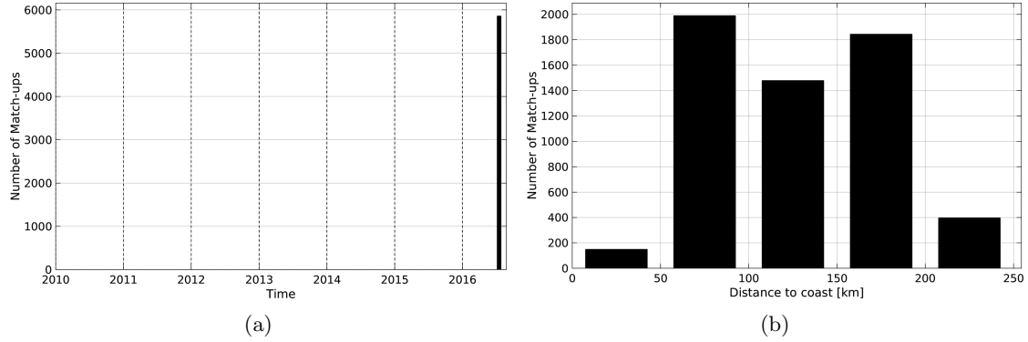
Figure 1: Number of match-ups between TSG-GOSUD-Research-vessel and SMOS-L3-CATDS-CECOS-IFREMER-V2-1DAY-0.5DEG SSS as a function of time (a) and as function of the distance to coast (b) over the Arctic Ocean Pi-MEP region and for the full satellite product period.
