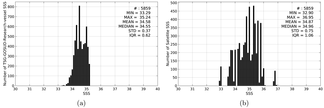
Figure 2: Histograms of SSS from TSG-GOSUD-Research-vessel (a) and SMOS-L3-CATDS-CECOS-IFREMER-V2-1DAY-0.5DEG (b) considering all match-up pairs per bins of 0.1 over the Arctic Ocean Pi-MEP region and for the full satellite product period.
