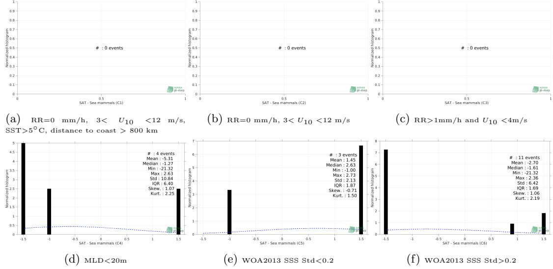
Figure 13: Normalized histogram of \Delta\text{SSS} (SMOS SSS L3 v2 - Daily - 0.5 Deg (CATDS-CECOS-IFREMER) - Sea mammals) for 6 different subdatasets corresponding to: RR=0 mm/h, 3 < U_{10} < 12 m/s, SST > 5^\circ\text{C} , distance to coast > 800 km (a), RR=0 mm/h, 3 < U_{10} < 12 m/s (b), RR > 1 mm/h and U_{10} < 4 m/s (c), MLD < 20 m (d), WOA2013 SSS Std < 0.2 (e), WOA2013 SSS Std > 0.2 (f).
