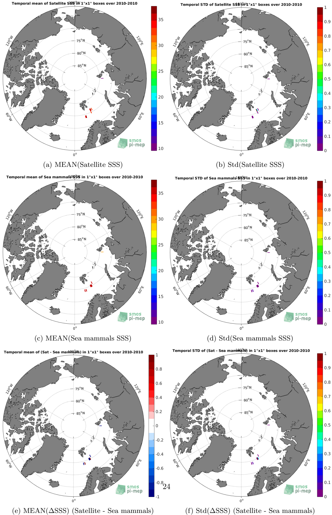
Figure 6: Temporal mean (left) and Std (right) of SSS from SMOS SSS L3 v2 - Daily - 0.5 Deg (CATDS-CECOS-IFREMER) (top), Sea mammals (middle), and of \Delta SSS (Satellite - Sea mammals). Only match-up pairs are used to generate these maps.
