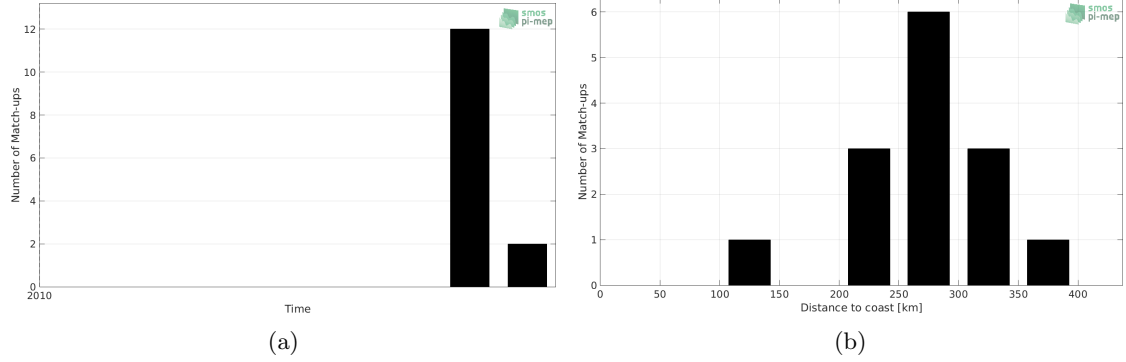
Figure 1: Number of match-ups between Sea mammals and SMOS SSS L3 v2 - Daily - 0.5 Deg (CATDS-CECOS-IFREMER) SSS as a function of time (a) and as function of the distance to coast (b) over the Arctic Ocean Pi-MEP region and for the full satellite product period.
