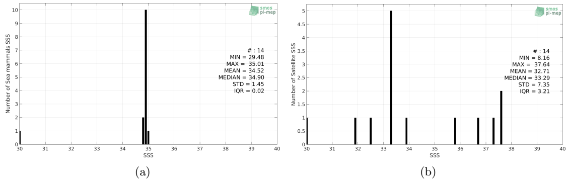
Figure 2: Histograms of SSS from Sea mammals (a) and SMOS SSS L3 v2 - Daily - 0.5 Deg (CATDS-CECOS-IFREMER) (b) considering all match-up pairs per bins of 0.1 over the Arctic Ocean Pi-MEP region and for the full satellite product period.
