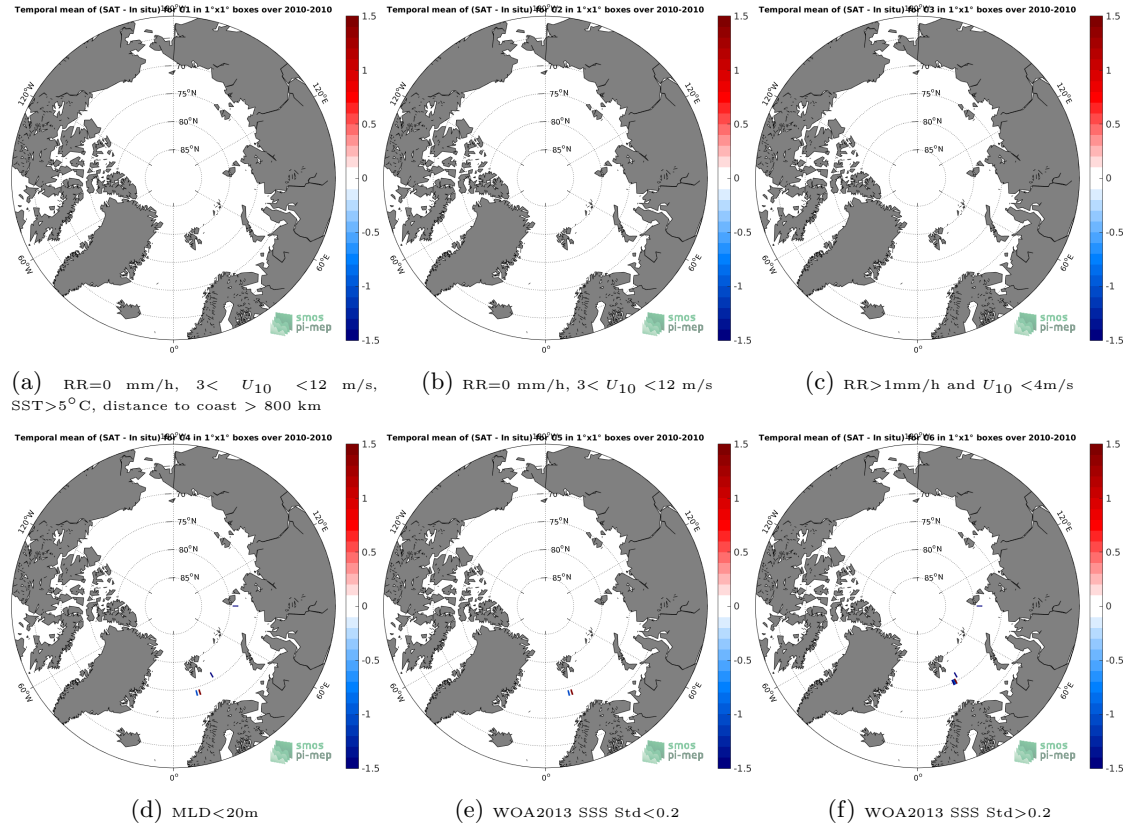
Figure 12: Temporal mean gridded over spatial boxes of size 1^{\circ}\times 1^{\circ} of \Delta\text{SSS} (SMOS SSS L3 v2 - Daily - 0.5 Deg (CATDS-CECOS-IFREMER) - Sea mammals) for 6 different subdatasets corresponding to:RR=0 mm/h, 3 < U_{10} < 12 m/s, SST >5^{\circ}\text{C} , distance to coast > 800 km (a), RR=0 mm/h, 3 < U_{10} < 12 m/s (b), RR >1 mm/h and U_{10} < 4 m/s (c),MLD <20 m (d),WOA2013 SSS Std <0.2 (e),WOA2013 SSS Std >0.2 (f).
