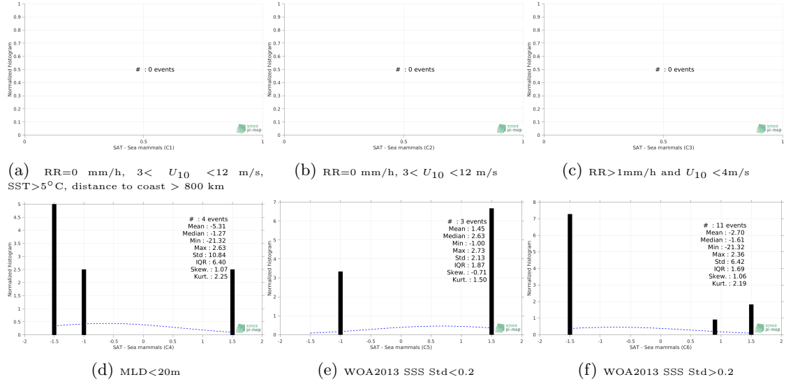
Figure 13: Normalized histogram of \Delta SSS (SMOS SSS L3 v2 - Daily - 0.5 Deg (CATDS-CECOS-IFREMER) - Sea mammals) for 6 different subdatasets corresponding to: RR=0 mm/h, 3 < U_{10} < 12 m/s, SST>5°C, distance to coast > 800 km (a), RR=0 mm/h, 3 < U_{10} < 12 m/s (b), RR>1mm/h and U_{10} < 4 m/s (c), MLD<20m (d), WOA2013 SSS Std<0.2 (e), WOA2013 SSS Std>0.2 (f).
