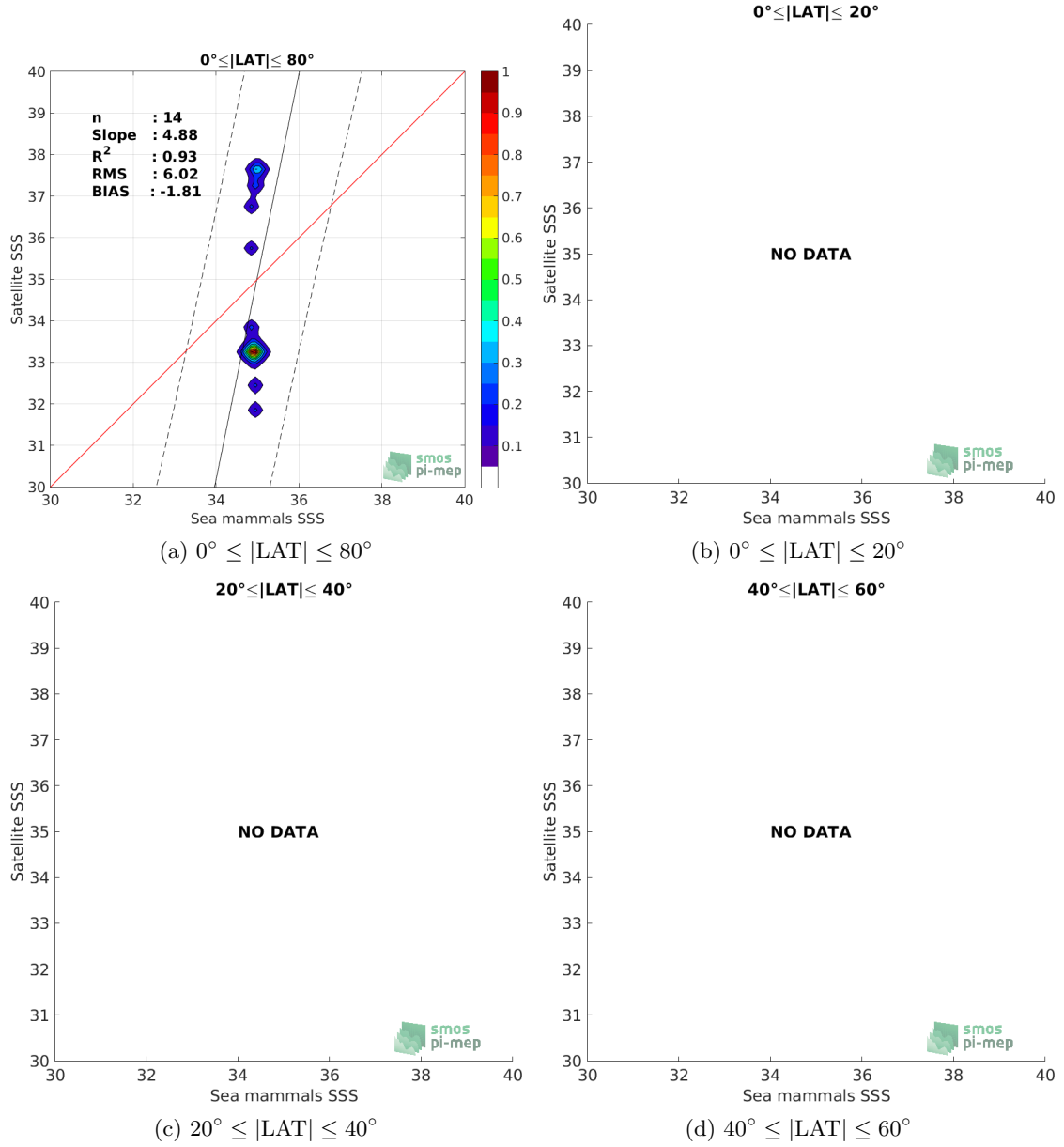
Figure 9: Contour maps of the concentration of SMOS SSS L3 v2 - Daily - 0.5 Deg (CATDS-CECOS-IFREMER) SSS (y-axis) versus Sea mammals SSS (x-axis) at match-up pairs for different latitude bands. For each plot, the red line shows x=y . The black thin and dashed lines indicate a linear fit through the data cloud and the \pm 95\% confidence levels, respectively. The number match-up pairs n , the slope and R^2 coefficient of the linear fit, the root mean square (RMS) and the mean bias between satellite and in situ data are indicated for each latitude band in each plots.
