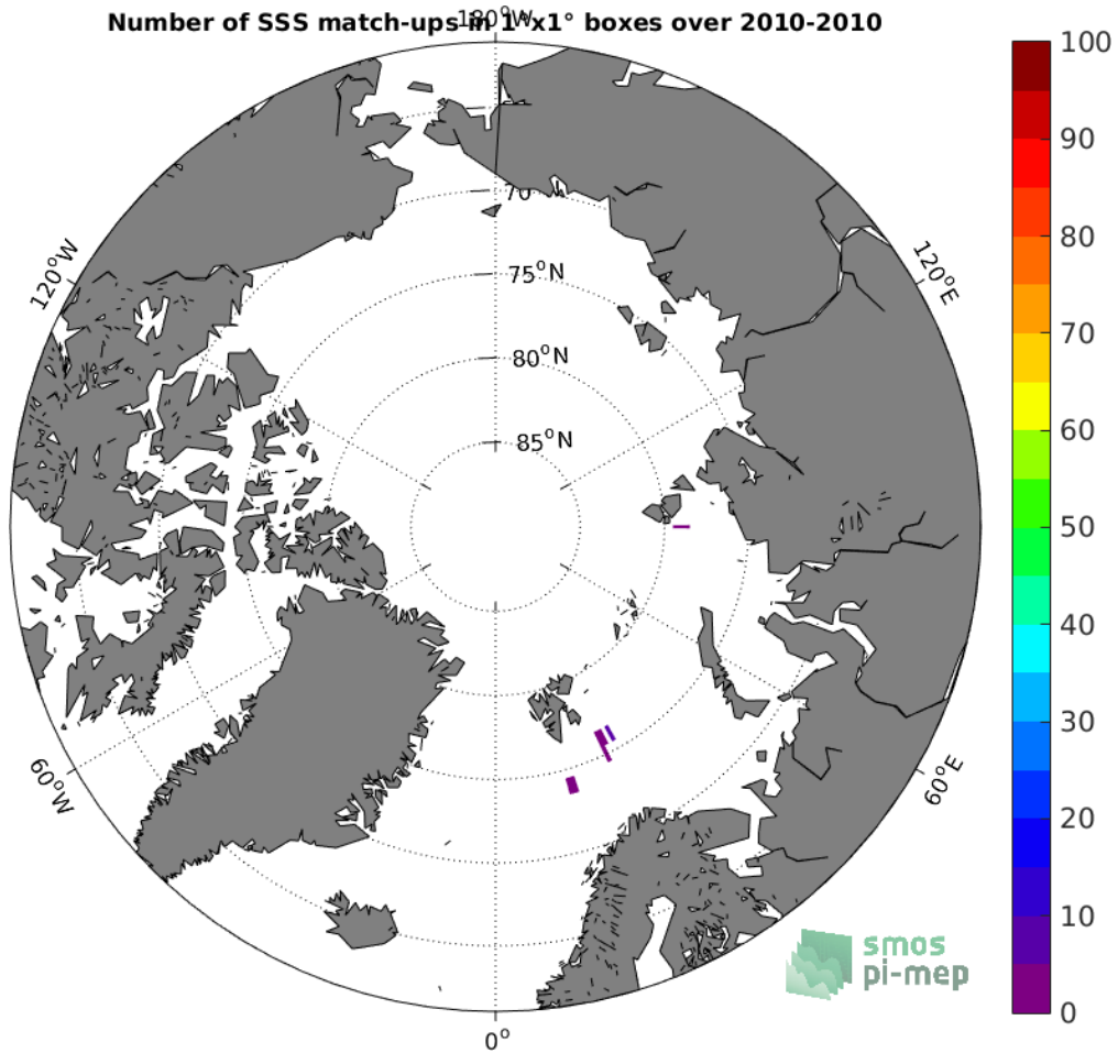
Figure 4: Number of SSS match-ups between Sea mammals SSS and the SMOS SSS L3 v2 - Daily - 0.5 Deg (CATDS-CECOS-IFREMER) SSS product for the Arctic Ocean Pi-MEP region over 1°x1° boxes and for the full satellite product period.
