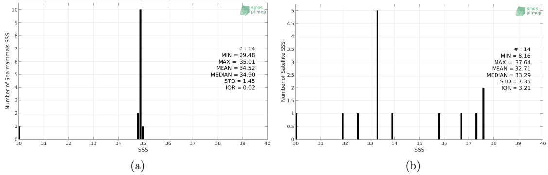
Figure 2: Histograms of SSS from Sea mammals (a) and SMOS L3 v2 - Daily - 0.5 Deg (CATDS-CECOS-IFREMER) (b) considering all match-up pairs per bins of 0.1 over the Arctic Ocean Pi-MEP region and for the full satellite product period.
