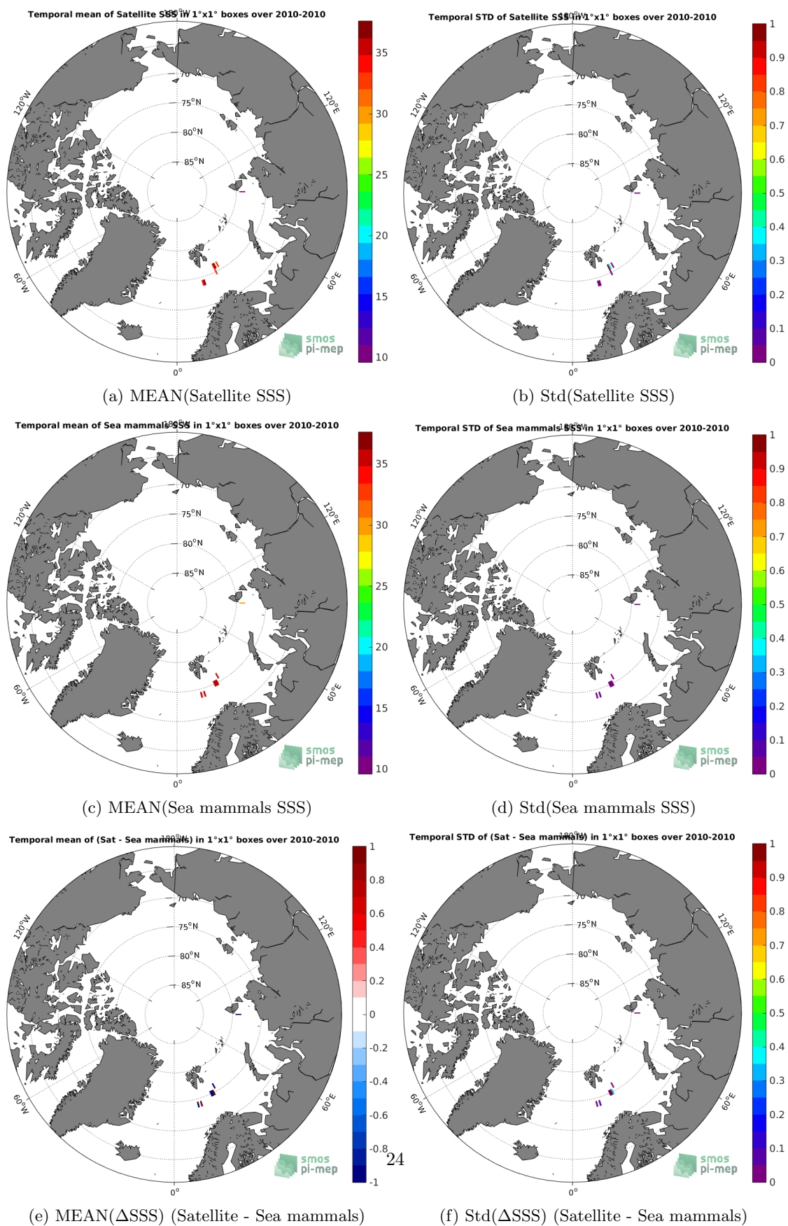
Figure 6: Temporal mean (left) and Std (right) of SSS from SMOS L3 v2 - Daily - 0.5 Deg (CATDS-CECOS-IFREMER) (top), Sea mammals (middle), and of \Delta SSS (Satellite - Sea mammals). Only match-up pairs are used to generate these maps.
