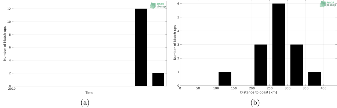
Figure 1: Number of match-ups between Sea mammals and SMOS L3 v2 - Daily - 0.5 Deg (CATDS-CECOS-IFREMER) SSS as a function of time (a) and as function of the distance to coast (b) over the Arctic Ocean Pi-MEP region and for the full satellite product period.
