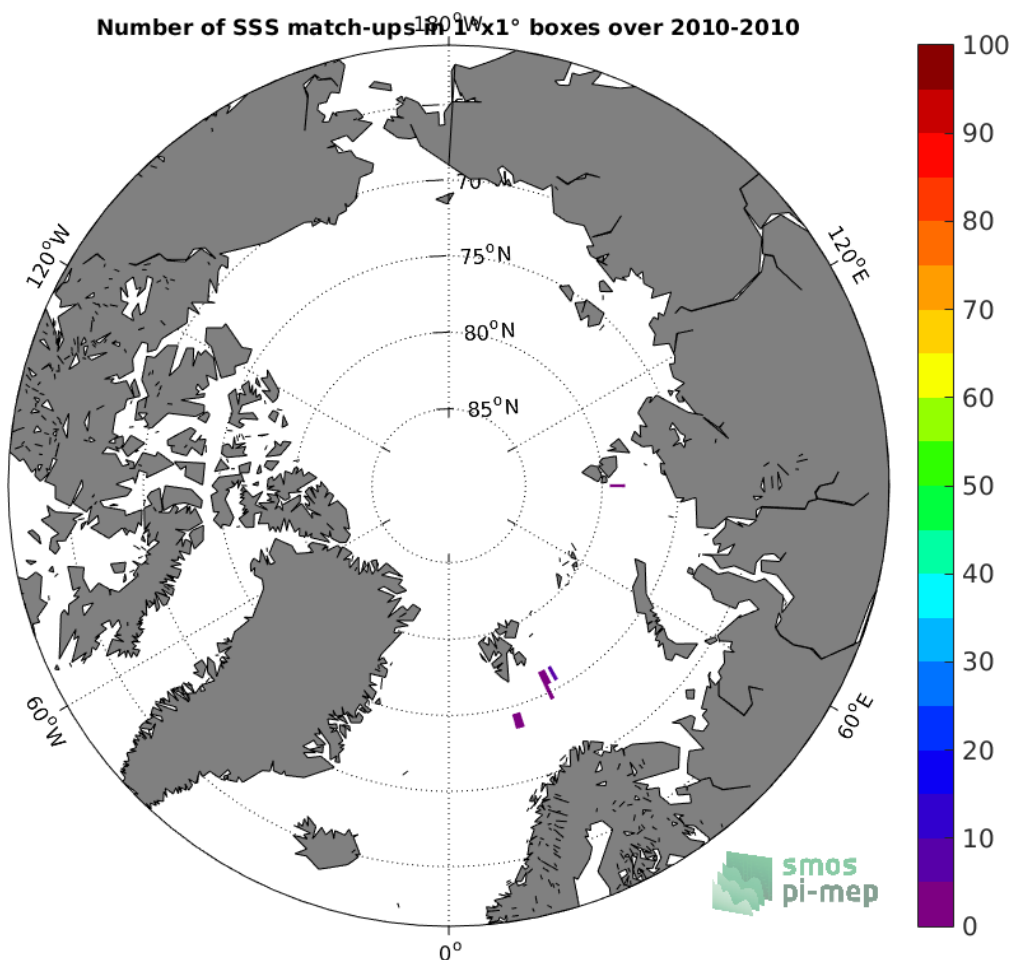
Figure 4: Number of SSS match-ups between Sea mammals SSS and the SMOS L3 v2 - Daily - 0.5 Deg (CATDS-CECOS-IFREMER) SSS product for the Arctic Ocean Pi-MEP region over 1^\circ \times 1^\circ boxes and for the full satellite product period.
