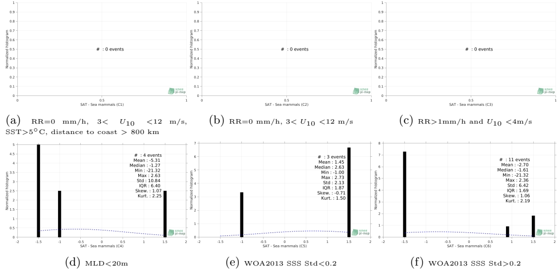
Figure 13: Normalized histogram of \Delta\text{SSS} (SMOS L3 v2 - Daily - 0.5 Deg (CATDS-CECOS-IFREMER) - Sea mammals) for 6 different subdatasets corresponding to: RR=0 mm/h, 3 < U_{10} < 12 m/s, SST > 5^\circ\text{C} , distance to coast > 800 km (a), RR=0 mm/h, 3 < U_{10} < 12 m/s (b), RR > 1\text{mm/h} and U_{10} < 4\text{m/s} (c), MLD < 20\text{m} (d), WOA2013 SSS Std < 0.2 (e), WOA2013 SSS Std > 0.2 (f).
