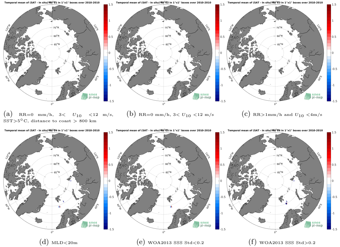
Figure 12: Temporal mean gridded over spatial boxes of size 1^{\circ}\times 1^{\circ} of \Delta\text{SSS} (SMOS L3 v2 - Daily - 0.5 Deg (CATDS-CECOS-IFREMER) - Sea mammals) for 6 different subdatasets corresponding to:RR=0 mm/h, 3 < U_{10} < 12 m/s, SST >5^{\circ}\text{C} , distance to coast > 800 km (a), RR=0 mm/h, 3 < U_{10} < 12 m/s (b), RR >1 mm/h and U_{10} < 4 m/s (c),MLD <20 m (d),WOA2013 SSS Std <0.2 (e),WOA2013 SSS Std >0.2 (f).
