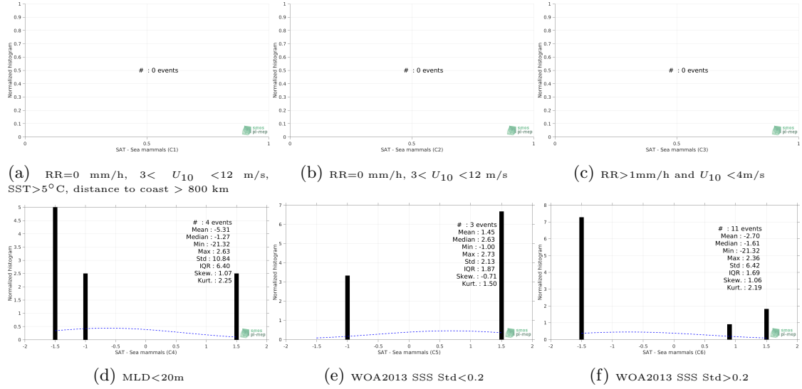
Figure 13: Normalized histogram of \Delta\text{SSS} (SMOS-L3-CATDS-CECOS-IFREMER-V2-1DAY-0.5DEG - Sea mammals) for 6 different subdatasets corresponding to: RR=0 mm/h, 3 < U_{10} < 12 m/s, SST > 5^\circ\text{C} , distance to coast > 800 km (a), RR=0 mm/h, 3 < U_{10} < 12 m/s (b), RR > 1 mm/h and U_{10} < 4 m/s (c), MLD < 20 m (d), WOA2013 SSS Std < 0.2 (e), WOA2013 SSS Std > 0.2 (f).
