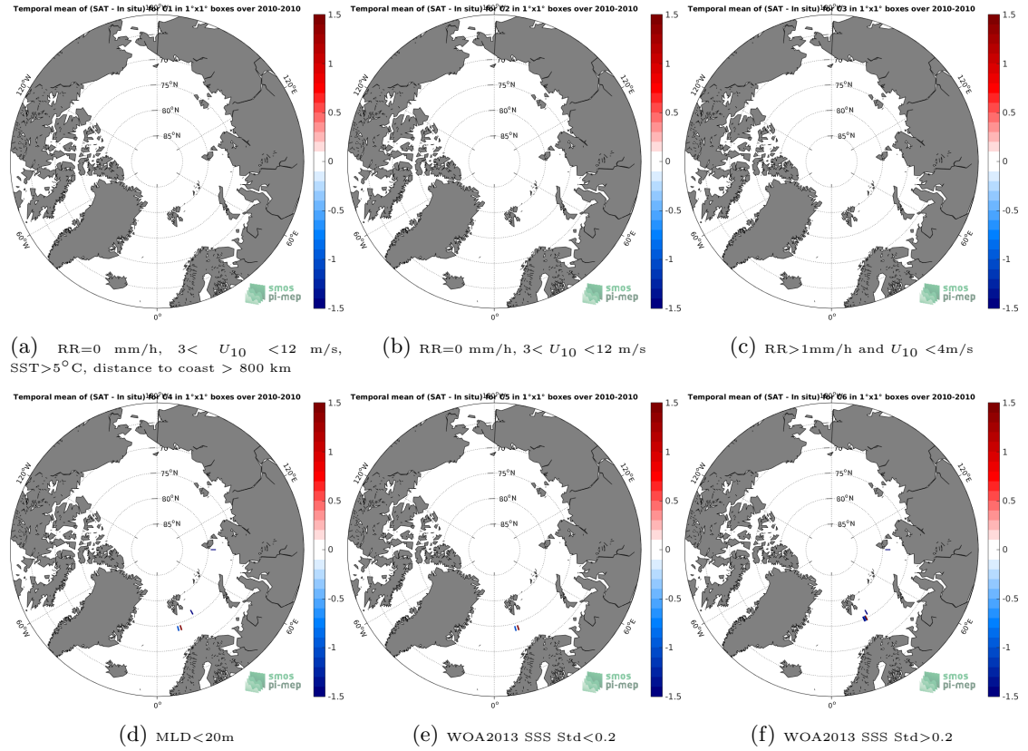
Figure 12: Temporal mean gridded over spatial boxes of size 1^\circ \times 1^\circ of \Delta SSS (SMOS-L3-CATDS-CECOS-IFREMER-V2-1DAY-0.5DEG - Sea mammals) for 6 different subdatasets corresponding to: RR=0 mm/h, 3 < U_{10} < 12 m/s, SST > 5^\circ\text{C} , distance to coast > 800 km (a), RR=0 mm/h, 3 < U_{10} < 12 m/s (b), RR > 1 mm/h and U_{10} < 4 m/s (c), MLD < 20 m (d), WOA2013 SSS Std < 0.2 (e), WOA2013 SSS Std > 0.2 (f).
