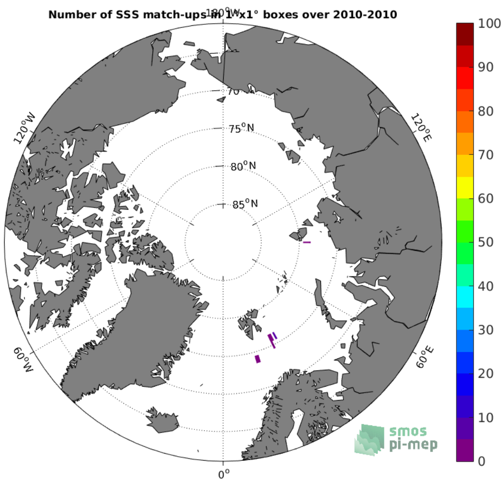
Figure 4: Number of SSS match-ups between Sea mammals SSS and the SMOS-L3-CATDS-CECOS-IFREMER-V2-1DAY-0.5DEG SSS product for the Arctic Ocean Pi-MEP region over 1^\circ \times 1^\circ boxes and for the full satellite product period.
