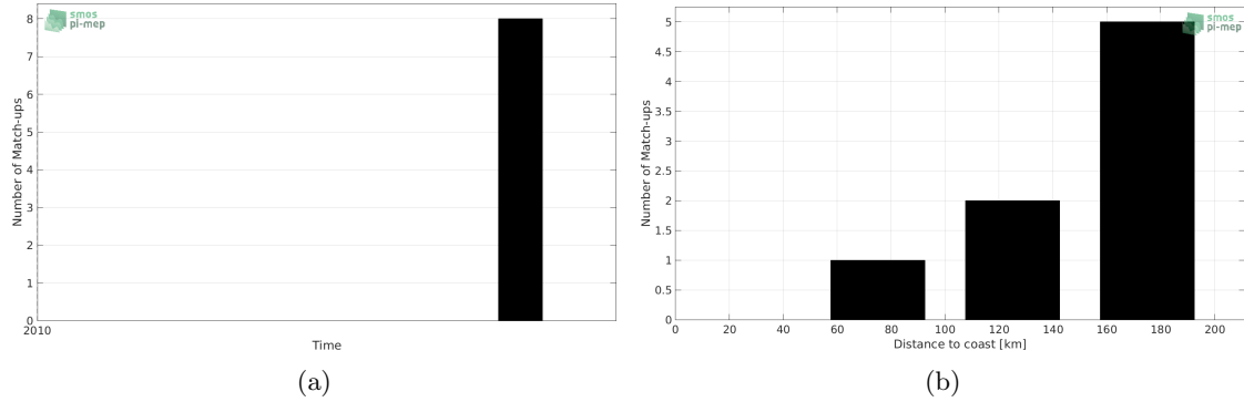
Figure 1: Number of match-ups between Sea mammals and SMOS-L3-CATDS-CECOS-IFREMER-V2-1DAY-0.5DEG SSS as a function of time (a) and as function of the distance to coast (b) over the Arctic Ocean Pi-MEP region and for the full satellite product period.
