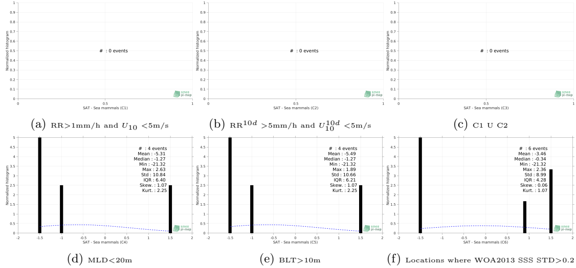
Figure 13: Normalized histogram of \Delta\text{SSS} (SMOS-L3-CATDS-CECOS-IFREMER-V2-1DAY-0.5DEG - Sea mammals) for 6 different subdatasets corresponding to: RR > 1\text{mm/h} and U_{10} < 5\text{m/s} (a), RR^{10d} > 5\text{mm/h} and U_{10}^{10d} < 5\text{m/s} (b), C1 U C2 (c), MLD < 20\text{m} (d), BLT > 10\text{m} (e), Locations where WOA2013 SSS STD > 0.2 (f).
