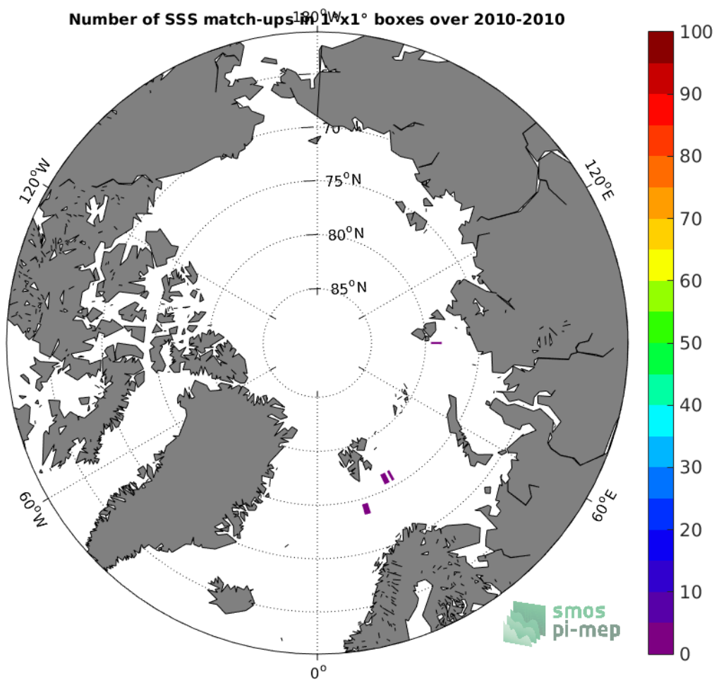
Figure 4: Number of SSS match-ups between Sea mammals SSS and the SMOS-L3-CATDS-CECOS-IFREMER-V2-1DAY-0.5DEG SSS product for the Arctic Ocean Pi-MEP region over 1°x1° boxes and for the full satellite product period.
