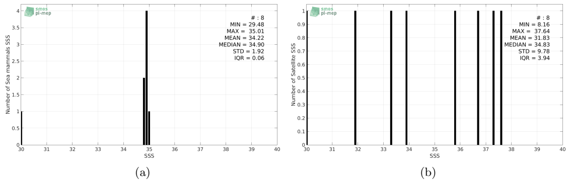
Figure 2: Histograms of SSS from Sea mammals (a) and SMOS-L3-CATDS-CECOS-IFREMER-V2-1DAY-0.5DEG (b) considering all match-up pairs per bins of 0.1 over the Arctic Ocean Pi-MEP region and for the full satellite product period.
