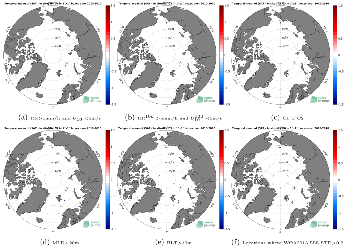
Figure 12: Temporal mean gridded over spatial boxes of size 1^\circ \times 1^\circ of \Delta\text{SSS} (SMOS-L3-CATDS-CECOS-IFREMER-V2-1DAY-0.5DEG - Sea mammals) for 6 different subdatasets corresponding to: \text{RR} > 1\text{mm/h} and U_{10} < 5\text{m/s} (a), \text{RR}^{10d} > 5\text{mm/h} and U_{10}^{10d} < 5\text{m/s} (b), C1 U C2 (c), \text{MLD} < 20\text{m} (d), \text{BLT} > 10\text{m} (e), Locations where WOA2013 SSS STD > 0.2 (f).
